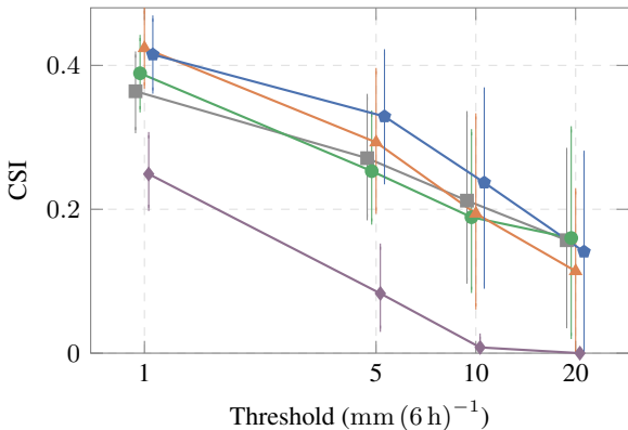
(a) Critical Success Index
