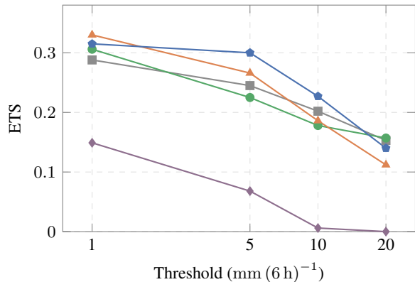
(b) Equitable Threat Score
