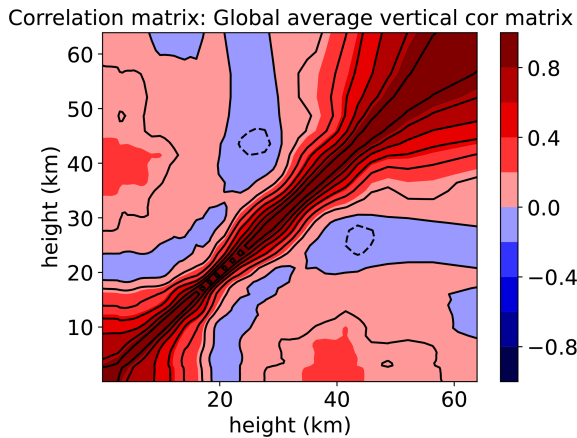
Figure 3. The vertical error correlation matrix for \chi(0) , which is used to find the eigenvectors, \mathbf{F}_{v\chi} , and eigenvalues, \mathbf{\Lambda}_{v\chi} . This matrix is computed according to the procedure outlined in Appendix C2.
