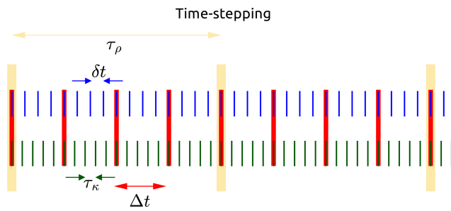
Figure 2. Timeline showing the time-stepping schemes used by EnviFlux, showing the four time intervals used. The back trajectories used for the semi-Lagrangian advection are of time length \Delta t , which are comprised of minor time-steps, \delta t . \Delta t is also the time interval of the wind files. Explicit diffusion effects are introduced with a timestep \tau_\kappa , and the flux fields have a time interval of \tau_\rho .
