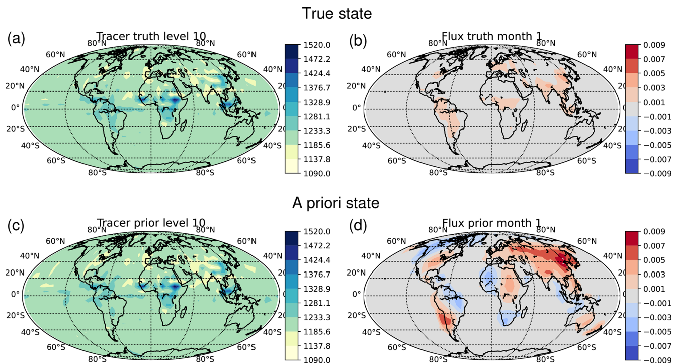
Figure 9. The true state (top row) and the a priori state (bottom row) chosen for the quasi-real experiments. The left column is for \chi(0) at level 10 (850 m above the ground, units \mu\text{g kg}^{-1} ) and the right column is for \rho(0) (corresponding to the first 30 d, units \mu\text{g m}^{-2} \text{s}^{-1} ). In (b) and (d), red is a source and blue is a sink.
