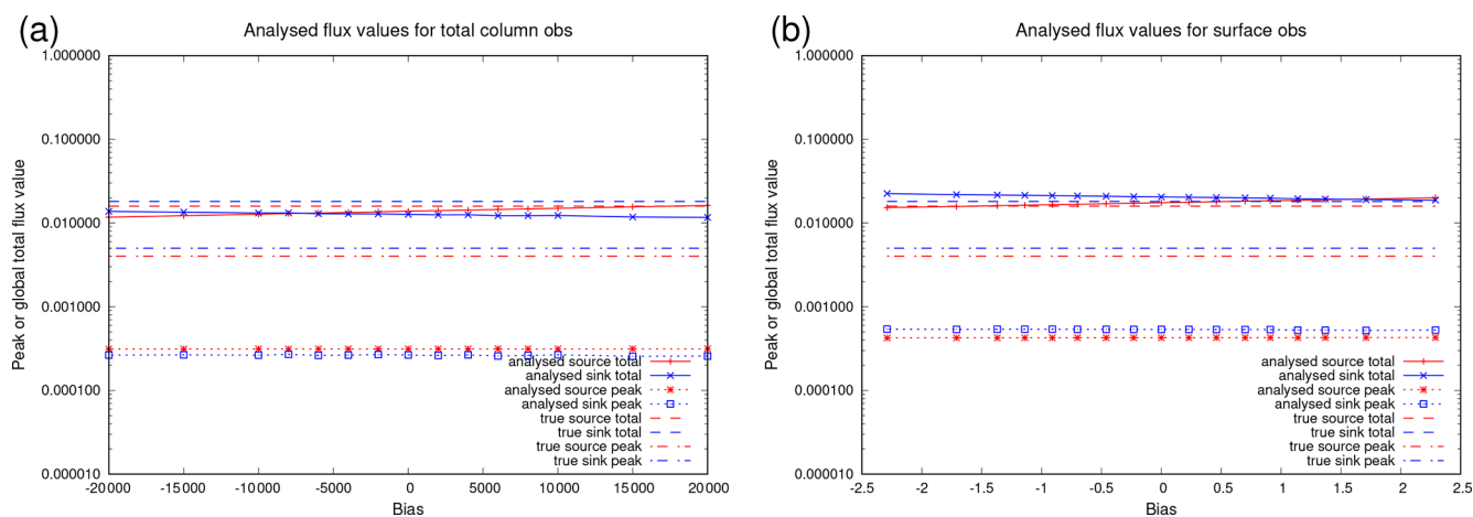
Figure 8. As Fig. 7a and c but for how the analysed global total, and the peak sources and sinks vary with observation bias. Panel (a) is for the TCA observations and (b) is for the SIS observations. The units are: global total values \text{Tg month}^{-1} and peak fluxes \mu\text{g m}^{-2} \text{s}^{-1} .
