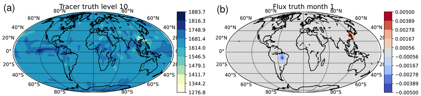
Figure 4. The true state chosen for the source/sink location detection experiments. Panel (a) is for \chi^t(0) at level 10 (850 m above the ground, units \mu\text{g kg}^{-1} ) and panel (b) is for \rho^t(0) (corresponding to the first 30 d, units \mu\text{g m}^{-2} \text{s}^{-1} ). In (b), red is a source and blue is a sink.
