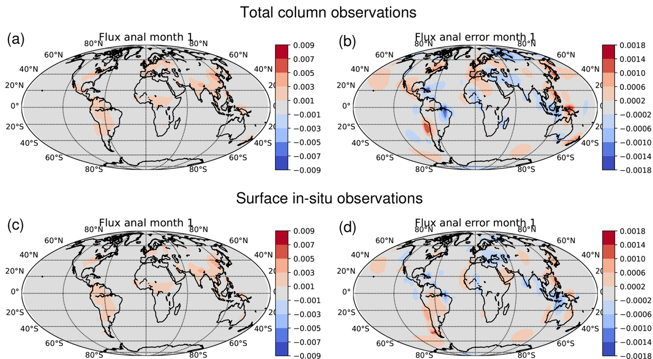
Figure 10. Analyses, \rho^a(0) (left column) and analysis errors (right column) for the quasi-real experiments (units \mu\text{g m}^{-2} \text{s}^{-1} ). The top row is for TCA and the bottom row is for SIS observations.
