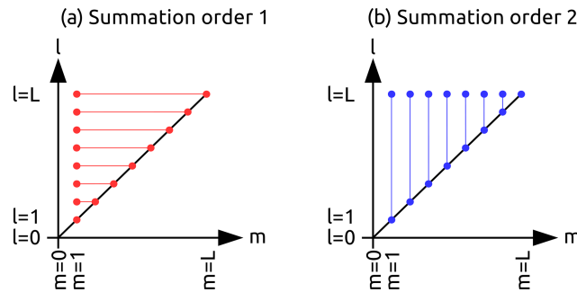
Figure A1. Orders of summations in m and l space as used in transforms (Eqs. A3 and A4). In order 1 (panel a), the sum over l is done first, and in order 2 (panel b), the sum over m is done first. Each order of summation is equivalent to the other as the same points are involved in the double summation.
