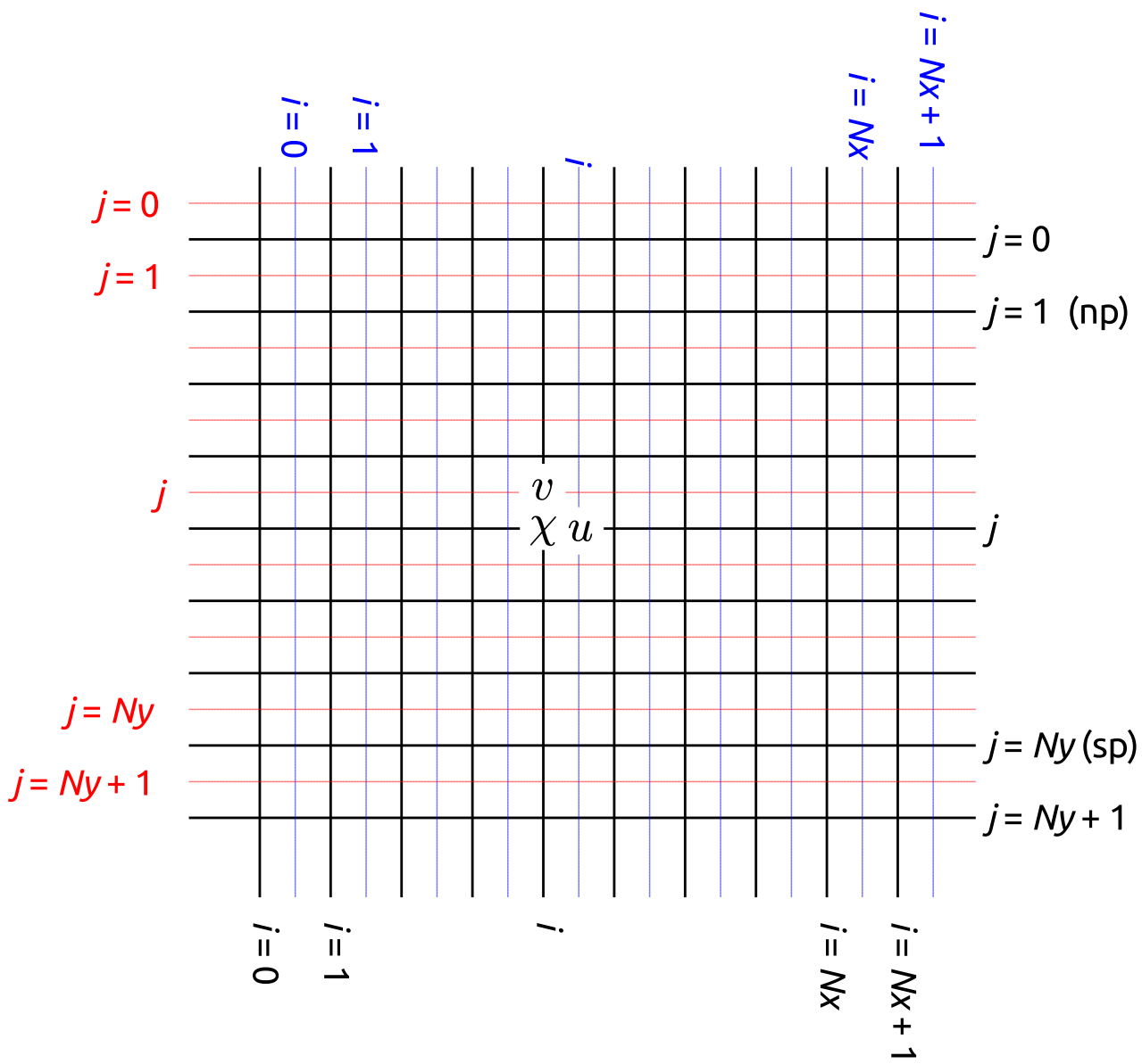
(a) The horizontal grid staggering
