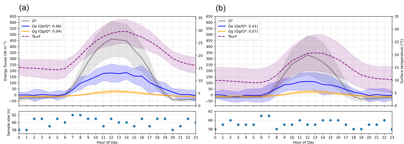
Figure 5. (a) Hourly composite diurnal cycle of the observed energy balance components for the summer period (July–August), and (b) the fall period (September–October), lower panels indicate the number of samples contributing to each hourly mean.
