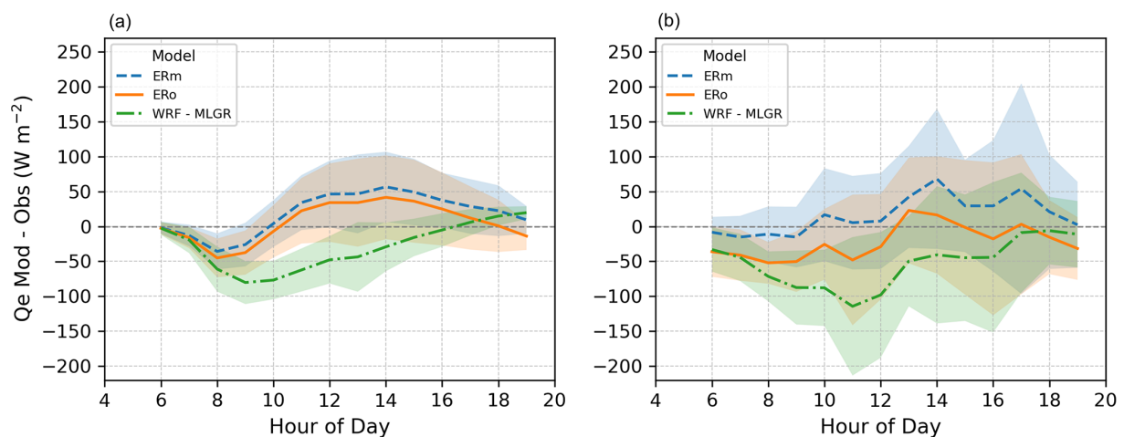
Figure 8. Hourly composite of the difference between modeled and observed Q_e for (a) dry days and (b) rainy days.
