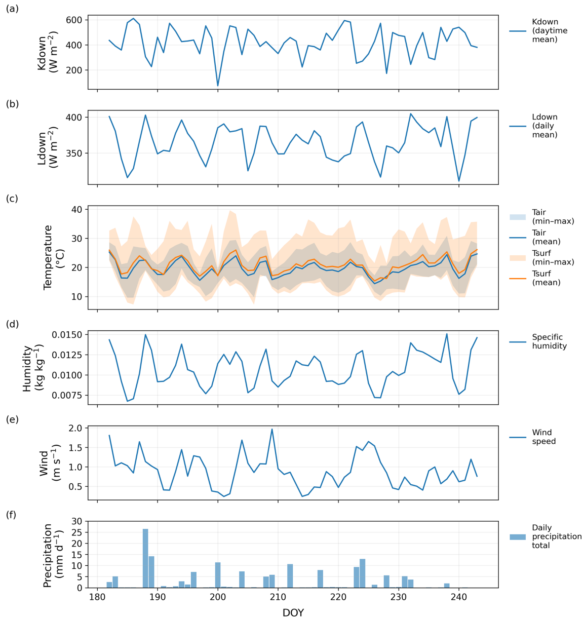
Figure 3. Weather conditions during the summer period. Panels (a) and (b) show daytime mean incoming shortwave ( K_{\text{down}} ) and daily mean longwave ( L_{\text{down}} ) radiation, respectively; panel (c) shows daily mean air and surface temperatures with shaded envelopes indicating the daily minimum–maximum temperature range; panel (d) shows daily mean specific humidity; panel (e) shows daily mean wind speed; and panel (f) shows daily precipitation totals.
