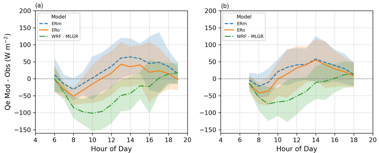
Figure 7. Hourly composite of the difference between modeled and observed Q_e for (a) the summer period and (b) the fall period.
