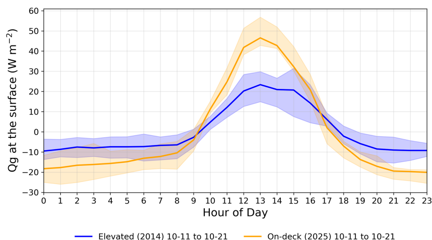
Figure 6. Hourly composite diurnal cycle of the observed soil heat flux ( Q_g ) for the elevated green roof on-deck configurations, data ranges from 11 to 21 October for both 2014 and 2025. Solid lines show the mean Q_g , while the shaded bands indicate \pm 1 standard deviation.
