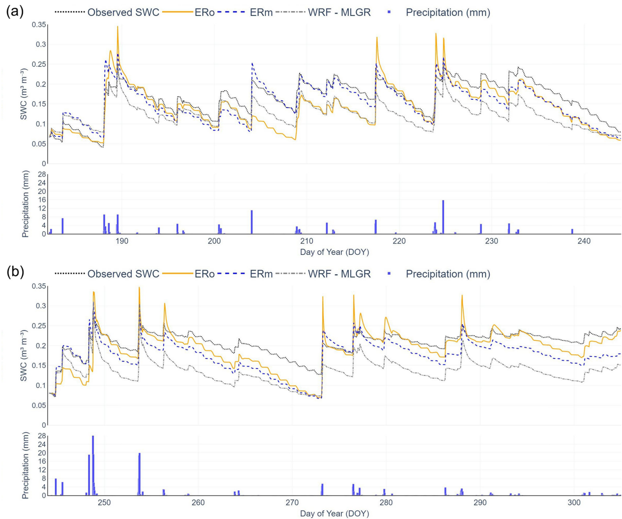
Figure 12. Time series of observed and modeled water content, with precipitation for (a) the summer period and (b) the fall period. Model simulations are shown as solid (ER o ), dashed (ER m ), and dash-dotted (WRF-MLGR) lines, while observations are shown as a dotted line, and blue bars indicate precipitation.
