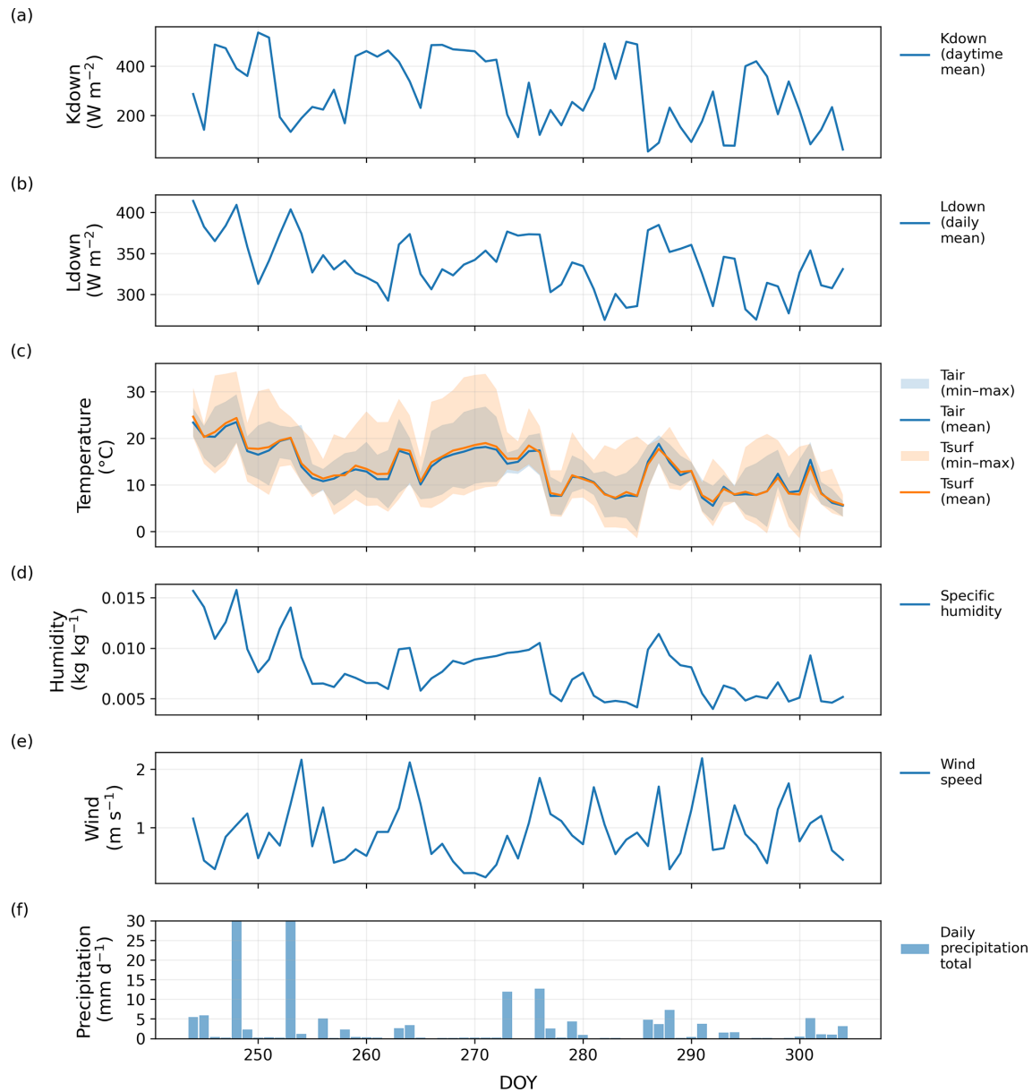
Figure 4. Weather conditions during the fall period. Panels (a) and (b) show daytime mean incoming shortwave ( K_{\text{down}} ) and daily mean longwave ( L_{\text{down}} ) radiation, respectively; panel (c) shows daily mean air and surface temperatures with shaded envelopes indicating the daily minimum–maximum temperature range; panel (d) shows daily mean specific humidity; panel (e) shows daily mean wind speed; and panel (f) shows daily precipitation totals.
