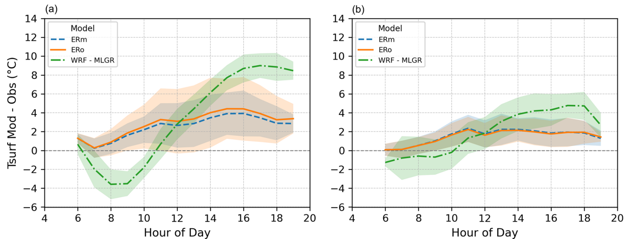
Figure 10. Hourly composite of the difference between modeled and observed T_{\text{surf}} for (a) high net radiation days and (b) low net radiation days.
