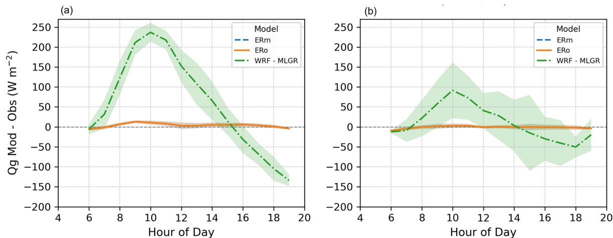
Figure 11. Hourly composite of the difference between modeled and observed Q_g for (a) high net radiation days and (b) low net radiation days.
