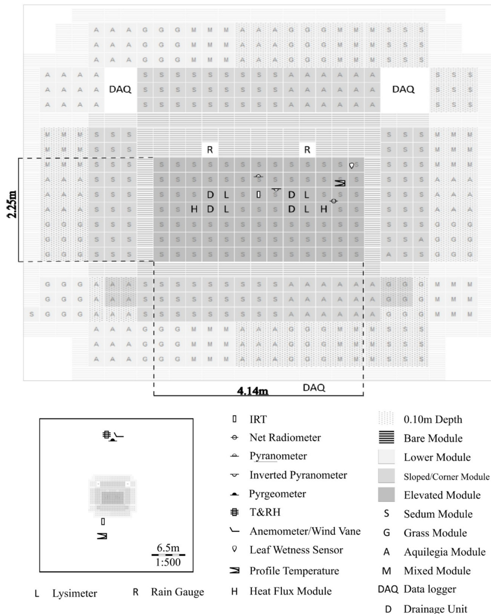
Figure 2. Green roof conceptual diagram (Kurukulaarachchi, 2017).
