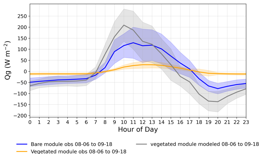
Figure 13. Hourly composite of the observed bare (non-vegetated) module (blue), observed vegetated module (yellow) and modeled vegetated module from WRF-MLGR (gray) Q_g . Solid lines represent the mean value and the shaded areas represent \pm 1 standard deviation. Legend also includes the plotted dates.
