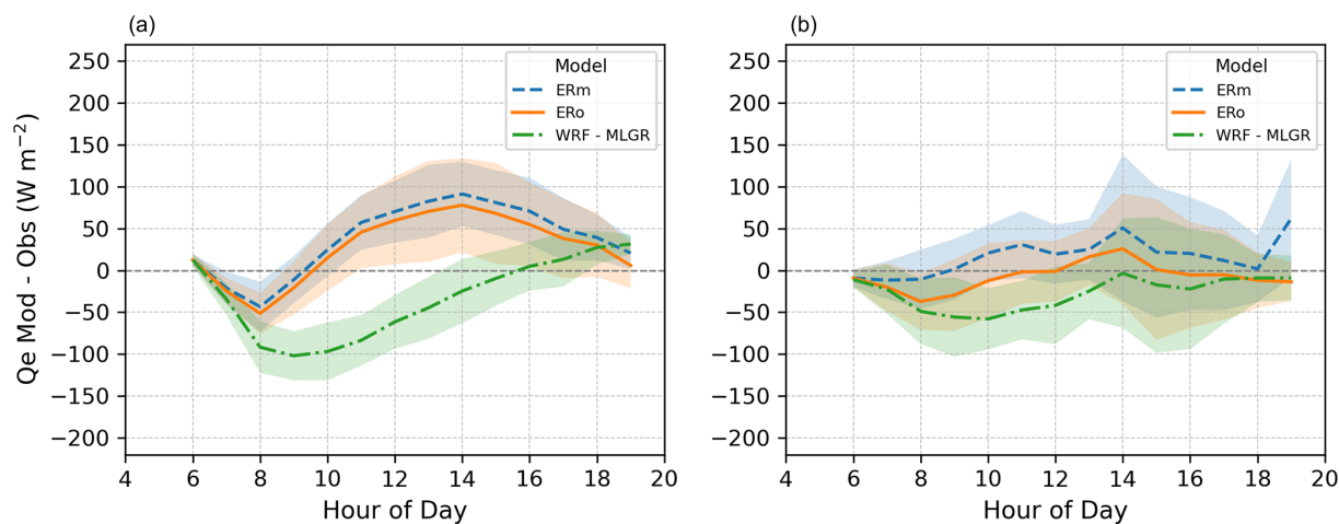
Figure 9. Hourly composite of the difference between modeled and observed Q_e for (a) high net radiation days and (b) low net radiation days.
