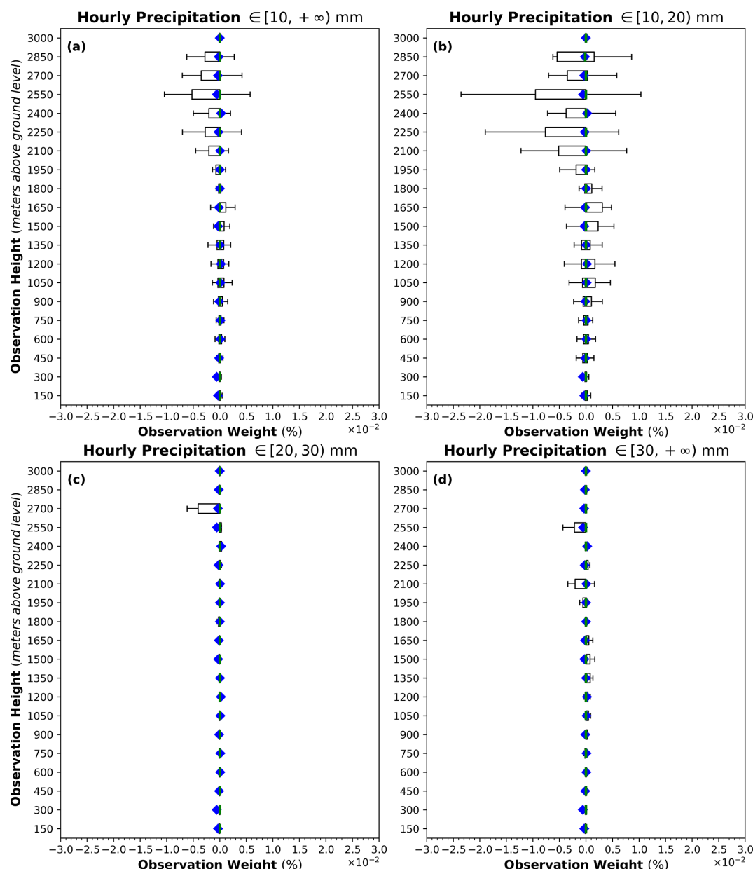
Figure 11. Same as Fig. 10, but for the differences in MRL observation weights between the GWMRnMRL and MRLOnly experiments.
