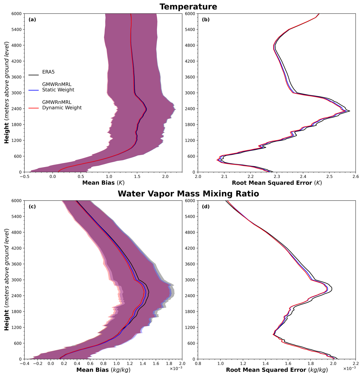
Figure 8. Same as Figs. 2 and 5, but for retrievals based on the synergistic assimilation of GMWR and MRL observations. Panels (a) and (b) show the vertical distributions of temperature MB and RMSE, respectively, while panels (c) and (d) show the corresponding statistics for water vapor mass mixing ratio. Gray, blue, and red curves represent the prior profiles, static observation weighting TCKF1D-Var retrievals, and adaptive observation weighting TCKF1D-Var retrievals, respectively. Shaded regions indicate the 95 % confidence intervals.
