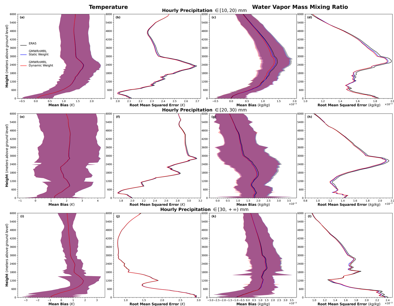
Figure 9. Same as Figs. 3 and 6, but for retrievals based on the synergistic assimilation of GMWR and MRL observations. Panels (a)–(d) show the MB and RMSE profiles of temperature and water vapor mass mixing ratio retrievals for cases with hourly accumulated precipitation of 10–20 mm. Panels (e)–(h) show the corresponding results for cases with hourly accumulated precipitation of 20–30 mm, while panels (i)–(l) present the results for cases with hourly accumulated precipitation exceeding 30 mm. Temperature retrieval statistics are shown in panels (a), (b), (e), (f), (i), and (j), and water vapor mass mixing ratio retrieval statistics are shown in panels (c), (d), (g), (h), (k), and (l). Gray, blue, and red curves denote the prior profiles, static observation weighting TCKF1D-Var retrievals, and adaptive observation weighting TCKF1D-Var retrievals, respectively. Shaded regions indicate the 95 % confidence intervals.
