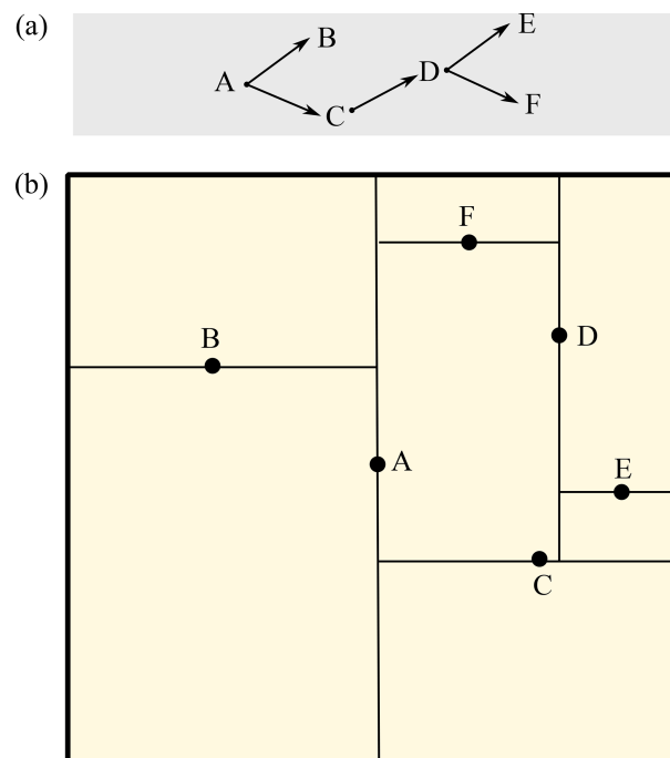
Figure B1. Simplified example of a k-d -tree in 2D (a) corresponding to the divisions in space shown in (b). Each level of the tree corresponds to a labelled line in the spatial visualisation. The levels of the tree alternate in axes (e.g., A is vertical, B and C are horizontal). Note that only a single branch is built completely, while others stop in earlier levels.
