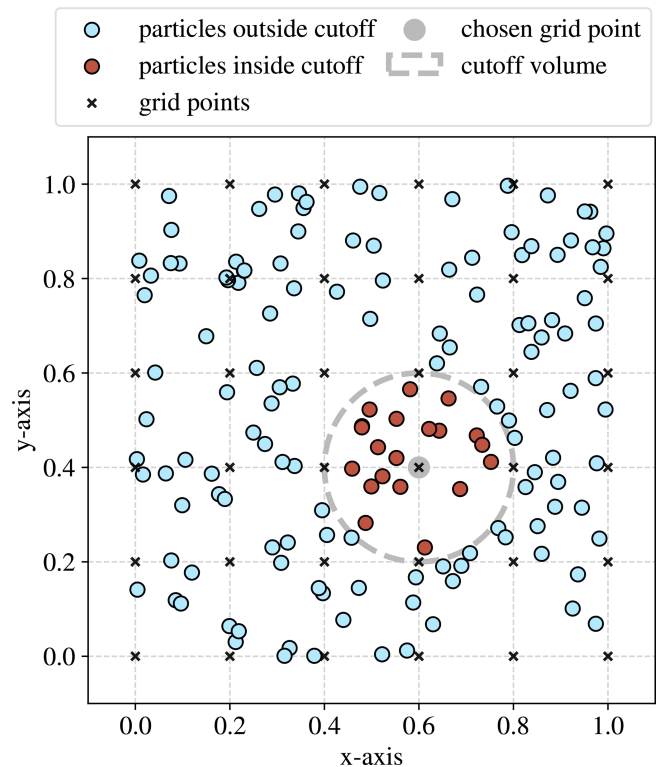
Figure 5. Visualisation of particle-to-node association. This plot displays an xy -plane projection of a synthetic set of particle positions in 3D (blue dots) within the framework of a regular grid (crosses). The particles associated with the grey grid point (red dots) are those within the cut-off volume (grey circle). The size of the dots is not informative of the size of the particles. For the sake of simplicity, no units are provided.
