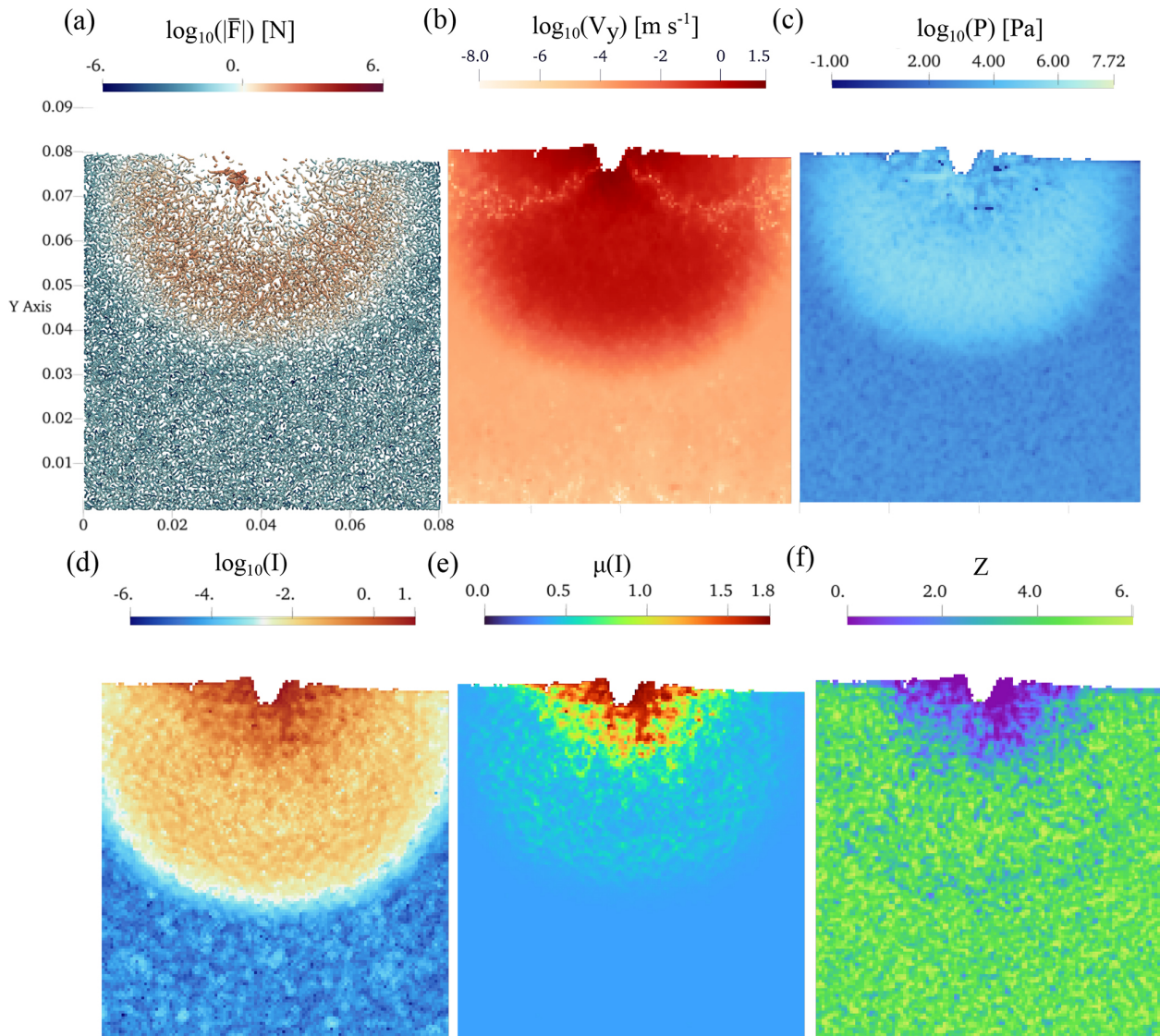
Figure 11. Vertical slices in the xy -plane ( z = 0.04 m) of the coarse-grained fields corresponding to the DEM numerical simulation of a polydisperse bed hit by an impactor presented in Fig. 10. The contact network is shown in (a), coloured by the normalised force magnitude ( |\bar{F}| ). The vertical component of the velocity ( V_y ), pressure ( P ), inertial number ( I ) and coordination number ( Z ) are displayed in (b), (c), (d) and (f), respectively. The coefficient of friction as a function of inertial number (i.e., \mu(I) -rheology) is shown in (e), where the static coefficient of friction of the mixture ( \sim 0.4 ) is coloured light-blue.
