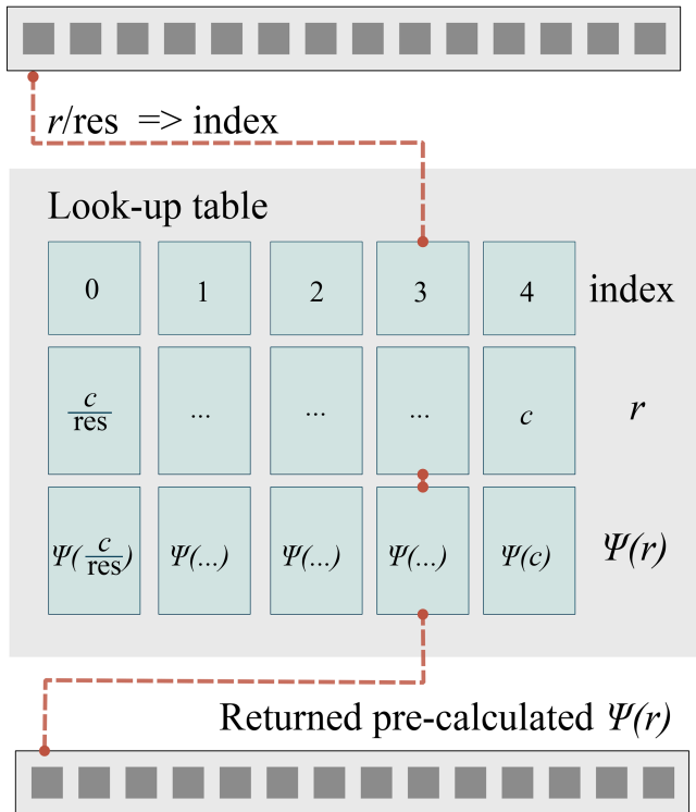
Figure B2. Schematic diagram of the lookup table algorithm implemented in Pysammos. r corresponds to the distance between a particle and a grid point. The resolution of the lookup table is \text{res} . \Psi(r) is the coarse-graining function, and c corresponds to its cut-off distance (i.e., \Psi(c) = 0 ).
