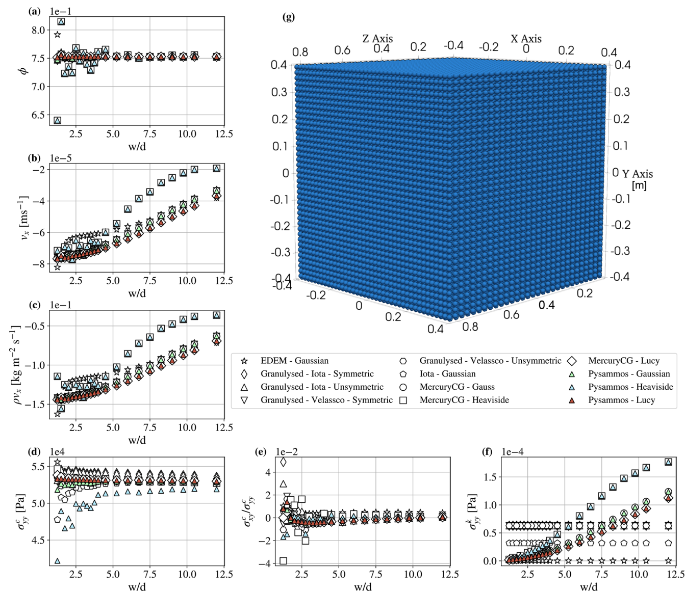
Figure 7. Benchmark of a monodisperse cubic lattice of grains with a diameter of 0.02 \text{ m} and density of 2500 \text{ kg m}^{-3} (g), at a point P = 0, 0, 0.42725 \text{ m} . It was coarse-grained with Pysammos (coloured triangles) and other coarse-graining software (void shapes): EDEM, Granulysed, Iota, and MercuryCG. Different smoothing functions (Gaussian, Heaviside and Lucy), are compared when available, for a range of smoothing half-width lengths multiples of the characteristic particle size (i.e., w/d ). The volume fraction is shown in (a). The horizontal component of the velocity and the momentum density are shown in (b) and (c), respectively. The vertical component of the contact stress is provided in (d), whereas (e) displays the ratio between the latter and the shear component in the xy -plane. Finally, the vertical component of the kinetic tensor is shown in (f).
