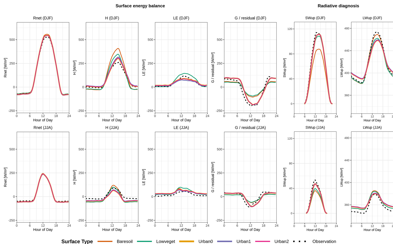
Figure 3. Diurnal cycle of net radiation ( R_{\text{net}} ), sensible heat ( H ), latent heat ( LE ), and ground heat flux ( G ) during summer months (DJF – first row), and winter months (JJA – second row) of observational period August 2003–November 2004 over the station AU-Preston in Melbourne, Australia, the reference station for the Urban-PLUMBER intercomparison projects. The black line represents the observations at the station, while the coloured lines represent the simulations outputs. G was not measured directly; the observational estimate shown here was diagnosed as the surface energy-balance residual, G = H + LE - R_{\text{net}} .
