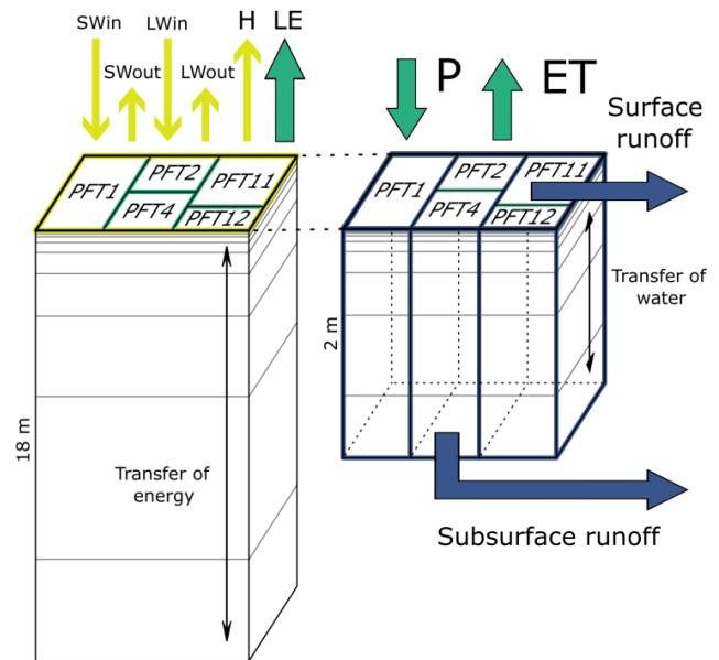
Figure 1. Schematic representation of the energy- and water-budget calculations in ORCHIDEE for a single grid cell, its plant functional types (PFTs), and the three associated soil columns representing bare soil, high vegetation, and low vegetation. Yellow arrows denote fluxes calculated directly at the grid-cell scale, green arrows denote fluxes calculated separately for each PFT and subsequently aggregated to the grid-cell scale, and dark-blue arrows denote fluxes calculated independently for each soil column. For example, sensible heat flux ( H ) is calculated at the grid-cell scale, evapotranspiration ( ET ) at the PFT scale, and surface runoff and subsurface runoff at the soil-column scale. Each soil column is discretized into 12 hydrological layers extending to a depth of 2 m, while the thermal discretization extends to 18 m. Abbreviations: P , precipitation; ET , evapotranspiration; H , sensible heat flux; SW , shortwave radiation; LW , longwave radiation; PFT, plant functional type.
