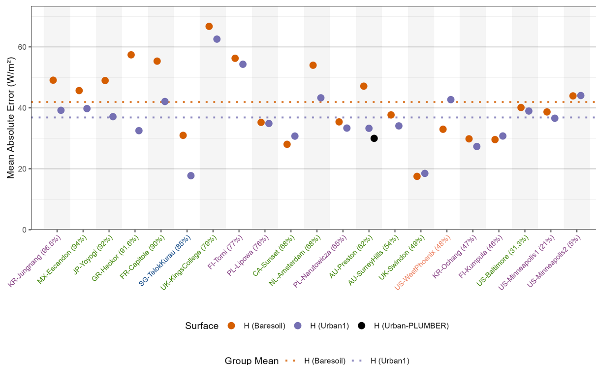
Figure 6. Same as Fig. 5, but for the sensible heat fluxes ( H ).
