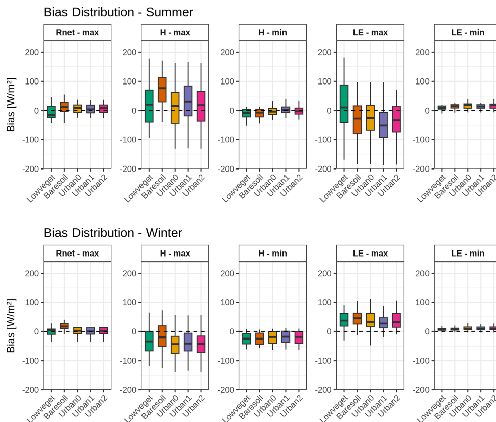
Figure 4. Distribution of mean bias in simulated daily maximum and minimum surface energy fluxes (sensible heat H , latent heat LE , and maximum net radiation R_{\text{net}} ) during summer (first row) and winter (second row) months (DJF/JJA based on hemisphere) across the 20 urban sites. For each boxplot, the central horizontal line indicates the median, the lower and upper edges of the box indicate the 25th and 75th percentiles, respectively, and the whiskers extend to the most extreme values within 1.5 times the interquartile range (IQR). The dashed horizontal line indicates zero bias.
