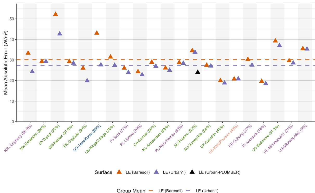
Figure 5. Mean Absolute Error (MAE) of latent heat fluxes ( LE ) over the 20 urban tower fluxes for the Baresoil and Urban1 simulations. The Urban-PLUMBER value (one black triangle) corresponds to the median Mean Absolute Error of latent heat flux from the “all – detailed” experiment shown in Fig. 6 of Lipson et al. (2024). The colours of the station’s labels along the x -axis indicate the climate of station: green for Temperate, purple for Continental, orange for Dry, and blue for Tropical. The percentage in these labels indicates the urban fraction around the station. The dashed horizontal lines indicate the mean MAE across all stations, shown in orange for Baresoil and in purple for Urban1.
