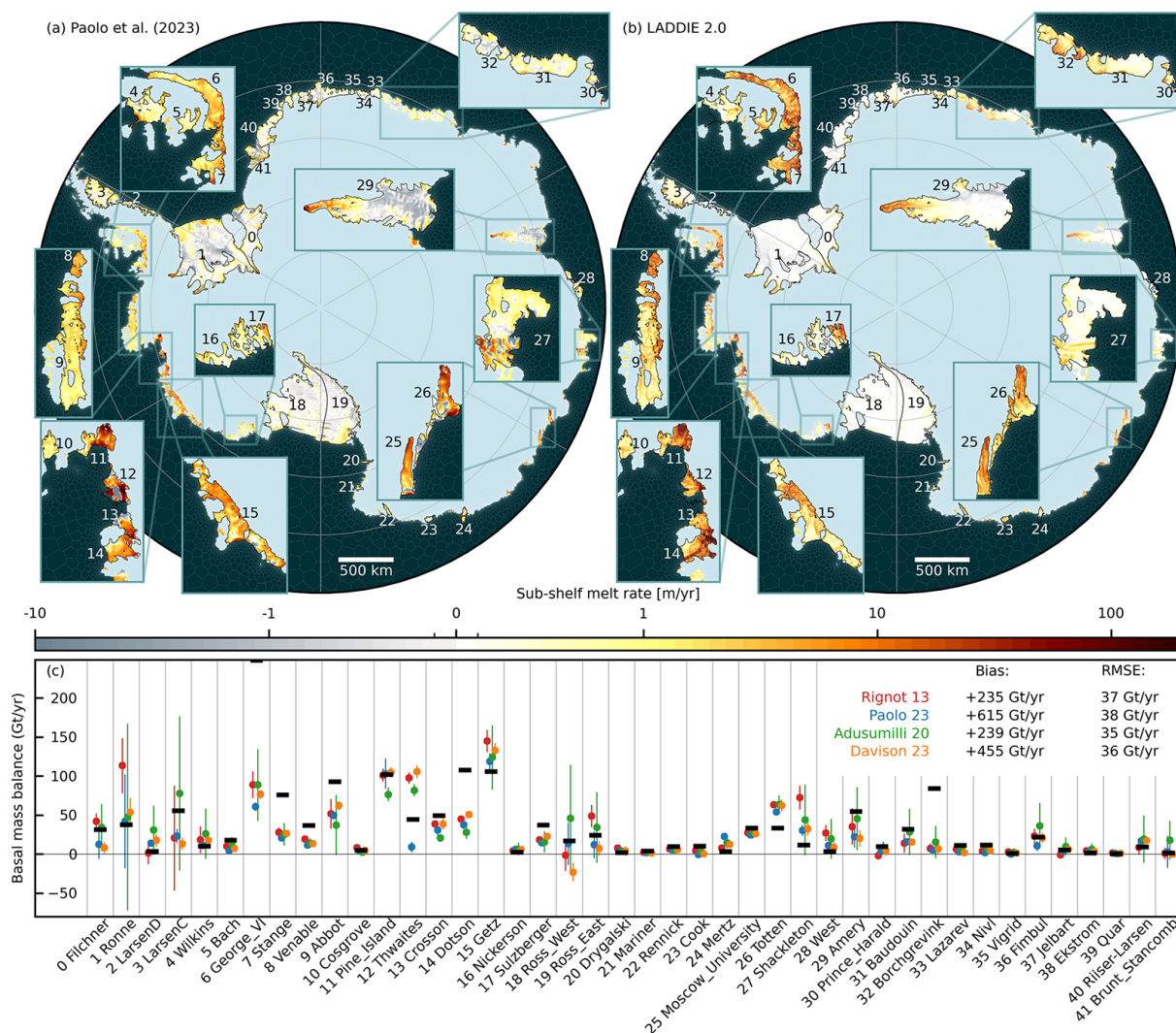
Figure 7. pan-Antarctic melt rates. (a) Remote sensing estimates by Paolo et al. (2023). (b) Model results from LADDIE 2.0, as in Fig. 6. Ice shelf boundaries (black) are derived from Measures (Mouginot et al., 2017). (c) A comparison of basal mass balance from LADDIE (black bars) to observations for individual ice shelves. Observations are from Rignot et al. (2013); Paolo et al. (2023); Adusumilli et al. (2020); Davison et al. (2023). The bulk metrics in the top right denote the bias in total basal mass balance of LADDIE with respect to individual remote sensing products, and the root mean squared error in basal mass balance of individual ice shelves.
