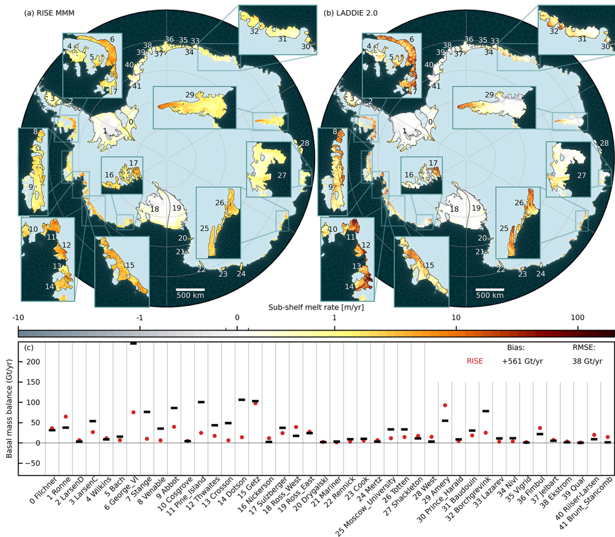
Figure 6. pan-Antarctic melt rates compared to 3D ocean models. (a) Multi-model mean from RISE (Galton-Fenzi et al., 2025). (b) Model results from LADDIE 2.0. Ice shelf boundaries (black) are derived from Measures (Mouginot et al., 2017). (c) A comparison of basal mass balance from LADDIE (black bars) to the RISE multi-model mean (red dots). The bulk metrics in the top right denote the bias in total basal mass balance of LADDIE with respect to RISE, and the root mean squared error in basal mass balance of individual ice shelves.
