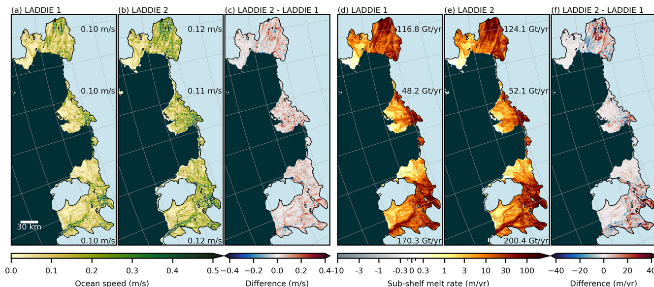
Figure 3. Amundsen Sea comparison between LADDIE 1.0 and LADDIE 2.0. Ocean speeds from (a) LADDIE 1.0, (b) LADDIE 2.0, and (c) the difference between the two model versions. White velocity vectors in (a) and (b) indicate the direction of the upper ocean flow. Average values for the Pine Island (top), Thwaites (middle), and Crosson–Dotson (bottom) ice shelves are noted. Sub-shelf melt rates for (d) LADDIE 1.0, (e) LADDIE 2.0, and (f) the difference. The numbers in (d) and (e) are integrated melt rates for the same three ice shelves. For visual reference, the grounding line (black line) as determined by LADDIE 2.0 is shown in each panel. Light blue colors denote grounded ice, dark green colors denote open ocean.
