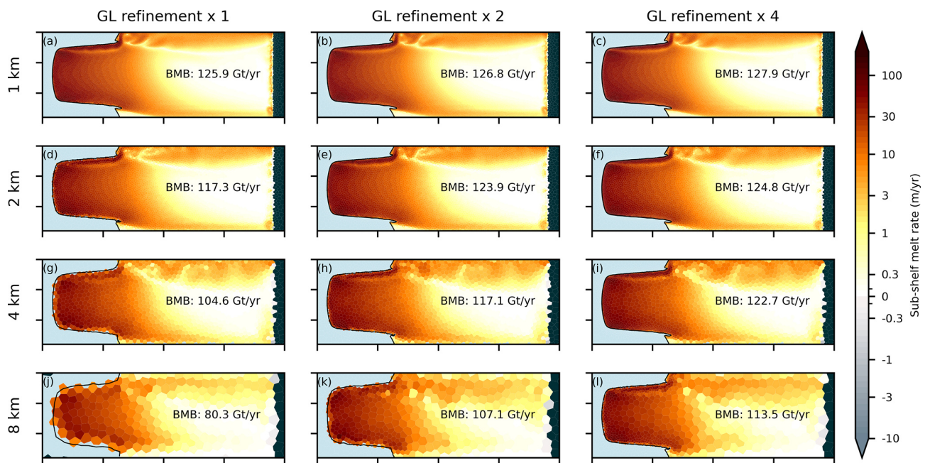
Figure A1. Sensitivity analysis to resolution over the ice shelf and refinement at the grounding line. The ISOMIP+ simulation of Sect. 3.2.1 was redone for four ice shelf resolutions (rows) and three refinement factors along the grounding line (columns). For each resolution, the integrated melt rate is expressed in \text{Gt yr}^{-1} .
