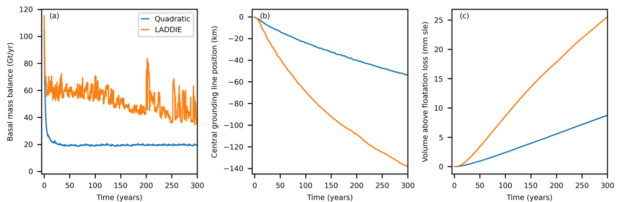
Figure 10. Time series of the two MISOMIP+ simulations. (a) The integrated basal mass balance over the whole ice shelf. (b) The grounding line position at y = 0 km, relative to the initial position at x = 450 km. (c) The volume above floatation loss.
