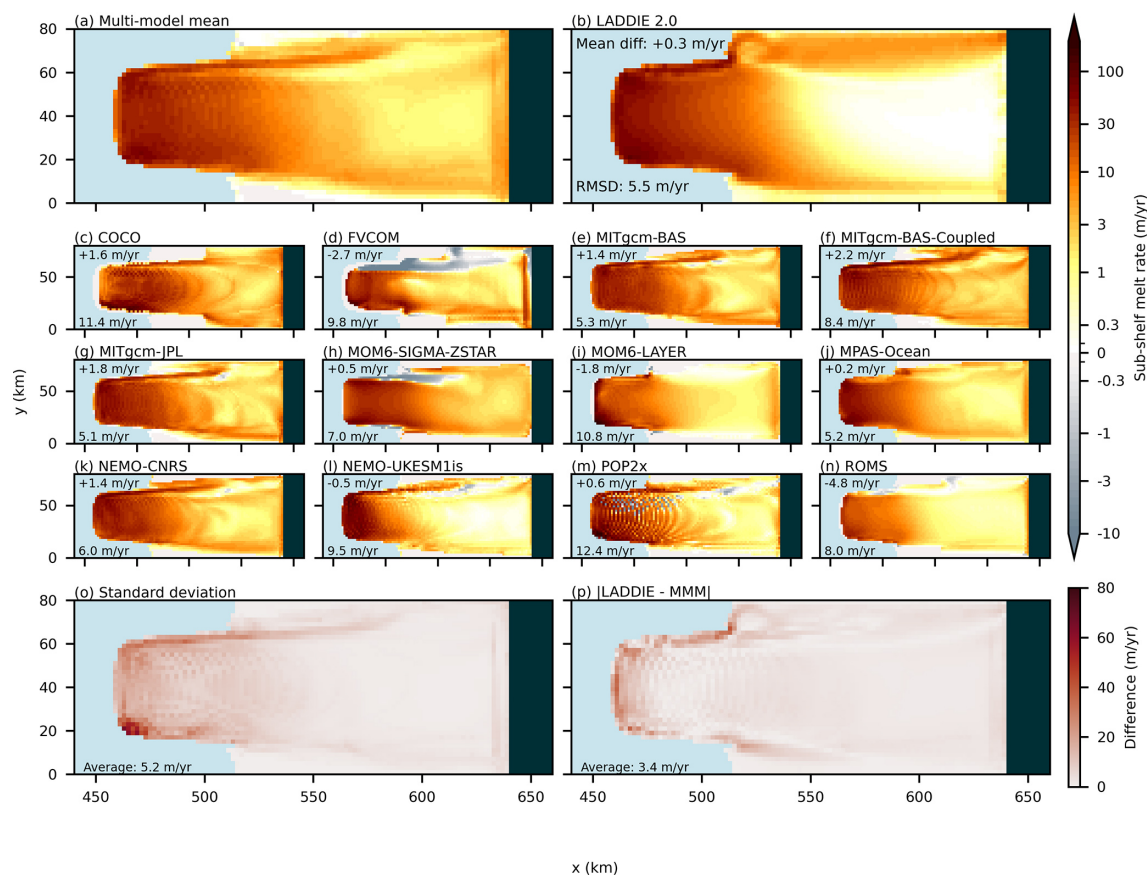
Figure 5. A comparison with 3D models based on the ISOMIP+ Ocean1 experiment. (a) The multi-model mean sub-shelf melt rates of 12 ocean models. (b) The results of LADDIE 2.0. (c–n) The results of the individual models. (o) The standard deviation of the 12 models. (p) The absolute difference between LADDIE 2.0 and the multi-model mean. In panels (b)–(n) , two bulk quantities are included: the top number is the mean difference with respect to the multi-model mean; the bottom number is the root mean squared difference.
