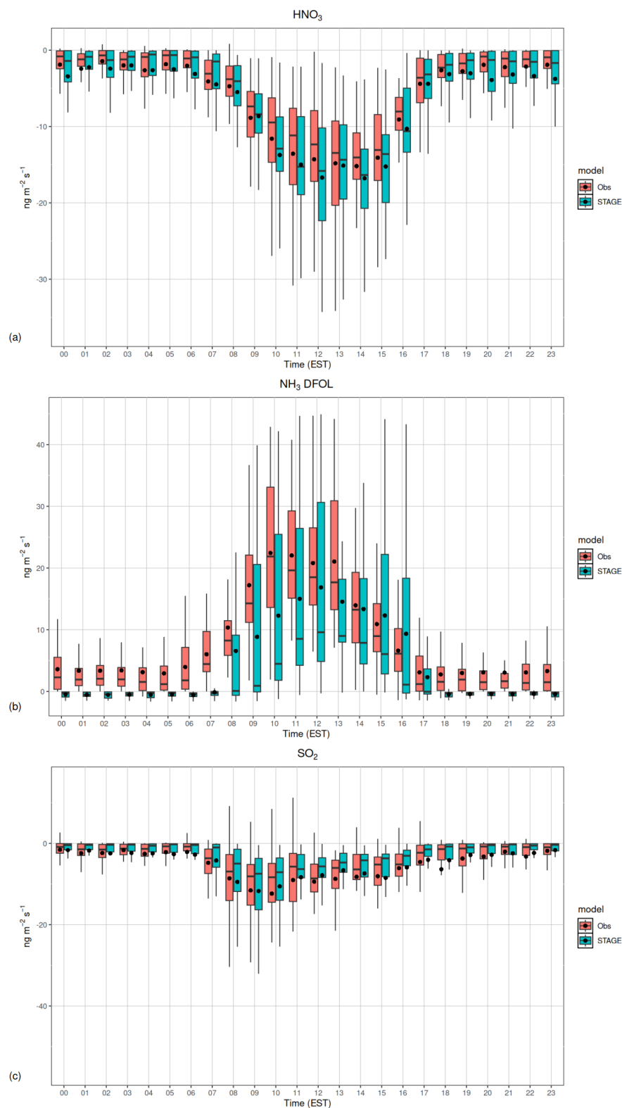
Figure 2. STAGE model estimates (blue) and observations (red) of the \text{HNO}_3 (a), \text{NH}_3 (b), and \text{SO}_2 (c) flux measurements taken at the Duke Forest grasslands flux tower. The box bounds the 25th to 75th percentiles, the lines extend to the 5th and 95th percentile, the black horizontal line is the median and the black point represents the mean of the modeled or observed hourly values. Note that negative values indicate net deposition and positive values indicate net evasion.
