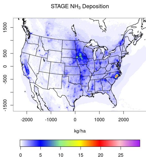
Figure 5. Annual \text{NH}_3 dry deposition, in \text{kg N ha}^{-1} , for the CMAQ STAGE model simulation evaluated in Appel et al. (2021).
