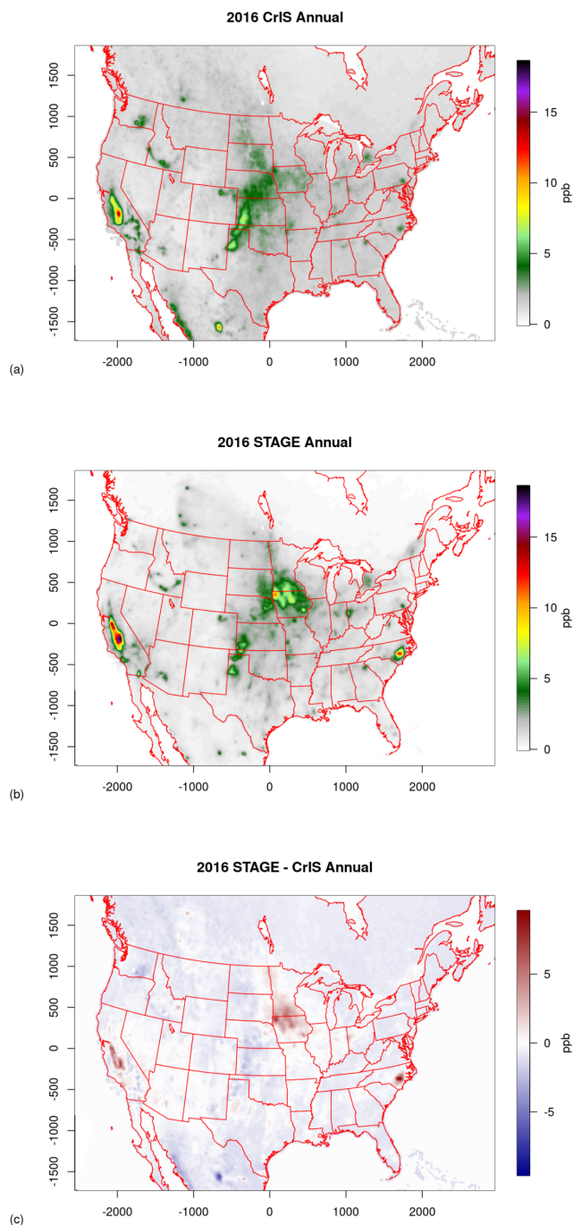
Figure 4. Annual mean Cross Infrared Sounder (CrIS) satellite surface \text{NH}_3 observations binned to CMAQ grid cells for 2016 (Top), mean CMAQ surface \text{NH}_3 estimates paired in space and time with CrIS observations for 2016 (Middle), the mean difference between CMAQ estimates and CrIS observations of \text{NH}_3 paired in space and time for 2016 (Bottom).
