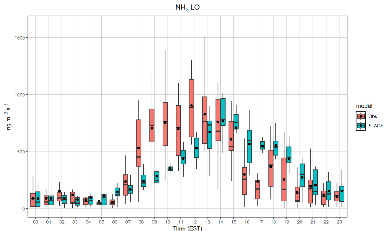
Figure 3. STAGE model estimates (blue) and observations (red) of NH 3 flux measurements taken at the Lillington, NC flux tower over a fertilized corn canopy. The box bounds the 25th to 75th percentiles, the lines extend to the 5th and 95th percentile, the black horizontal line is the median and the black point represents the mean of the modeled or observed hourly values.
