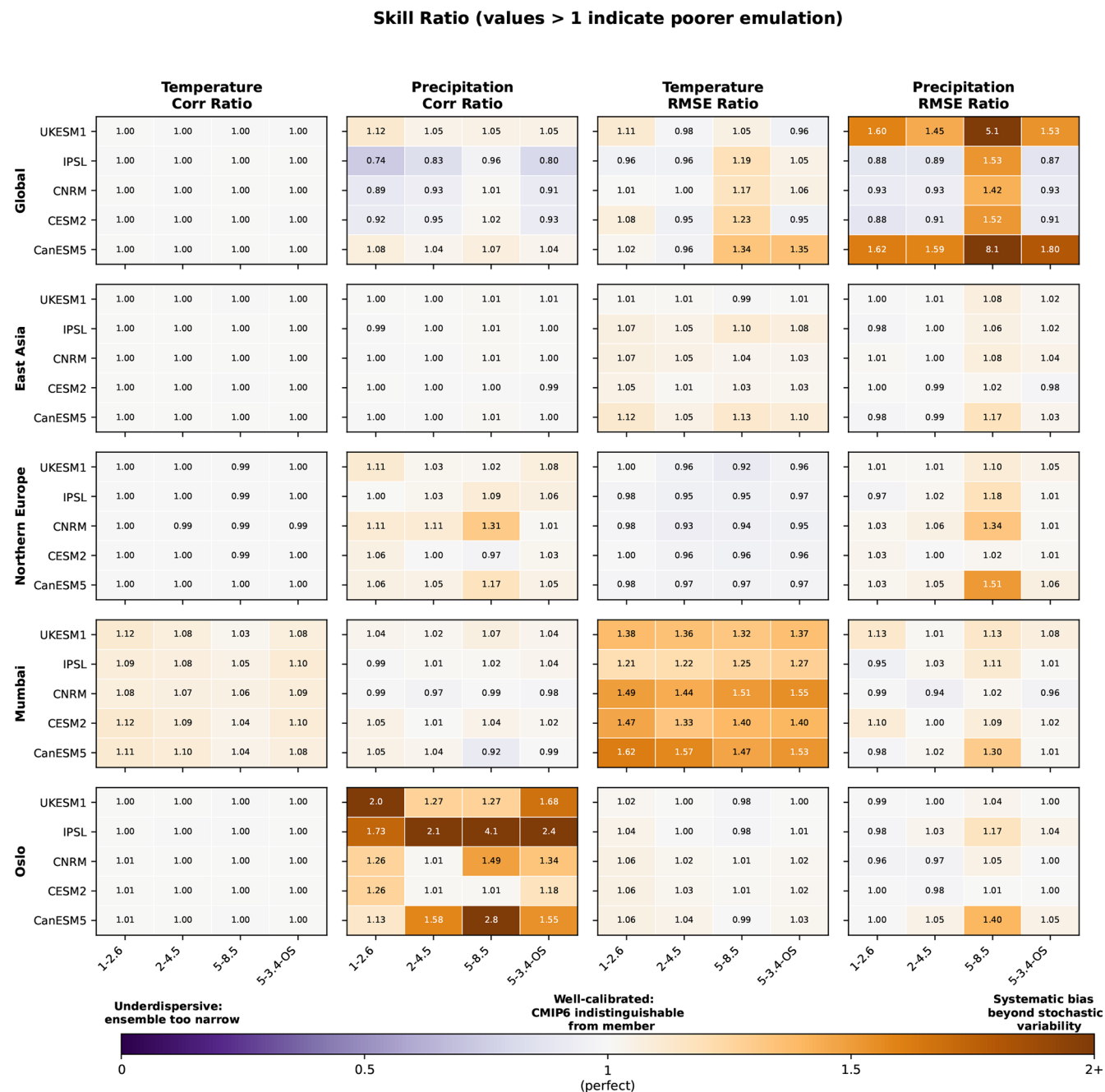
Figure 10. Skill ratio analysis for out-of-sample validation across all spatial scales (rows), models, and scenarios. Each panel shows a grid of model-scenario combinations. Skill ratios are defined such that values > 1 (orange) indicate poorer emulation for both metrics: for correlation, ratio = Member-Member / Member-CMIP6; for RMSE, ratio = Member-CMIP6 / Member-Member. Values near 1 (white) indicate CMIP6 is statistically indistinguishable from a METEOR ensemble member; values < 1 (purple) suggest ensemble underdispersion. Temperature ratios are consistently near unity; precipitation shows more variability, particularly at global scales where forced response bias is evident.
