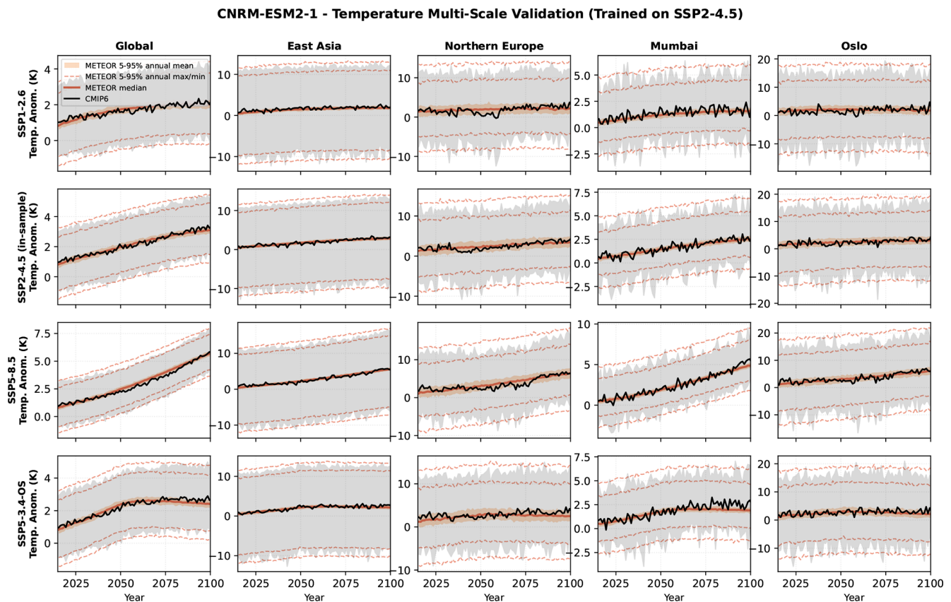
Figure 7. Out-of-sample temperature validation for CNRM-ESM2-1 trained on SSP2-4.5. Each row shows a validation scenario (SSP1-2.6, SSP2-4.5, SSP5-8.5, SSP5-3.4-OS); each column shows a spatial scale (global, East Asia, Northern Europe, Mumbai, Oslo). Orange shading: METEOR 5 %–95 % ensemble range of annual means. Orange dashed lines: 5 %–95 % range of annual maximum and minimum values. Orange solid line: ensemble median of annual means. Black line and grey shading: CMIP6 annual mean and monthly min/max envelope. Results for other models are shown in Figs. S1–S4.
