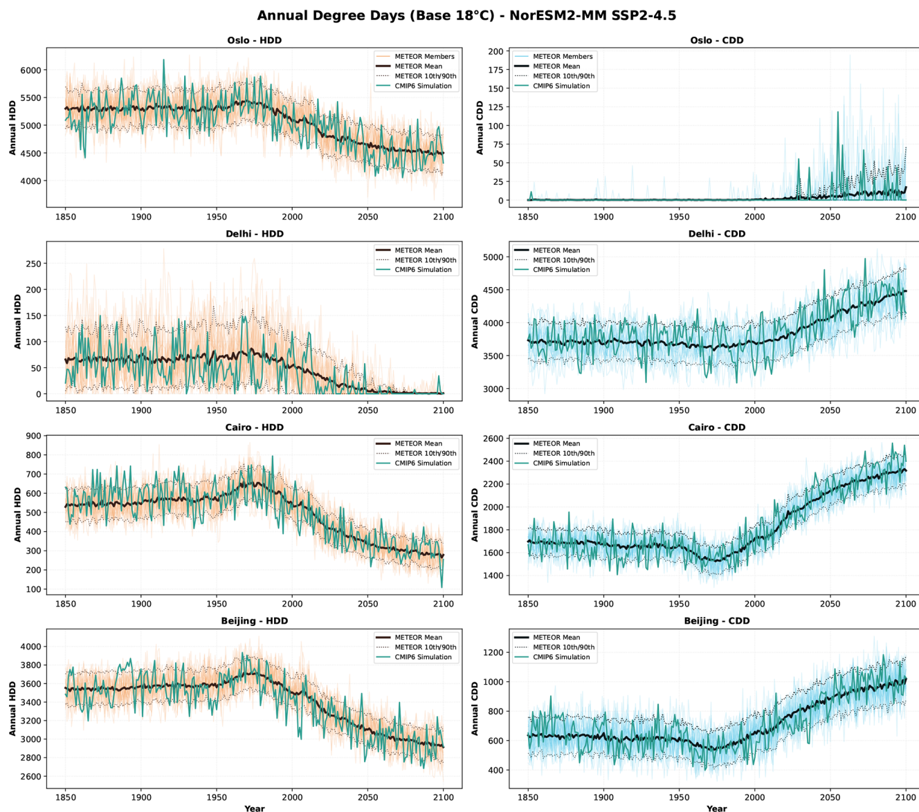
Figure 6. Heating degree days (HDD) and cooling degree days (CDD) for selected cities, comparing METEOR ensemble projections with NorESM2-MM. Notable features include the aerosol-related increase in HDD in Beijing during the late 20th century and the absence of cooling demands in Oslo until mid-21st century, both faithfully reproduced by the emulator.
