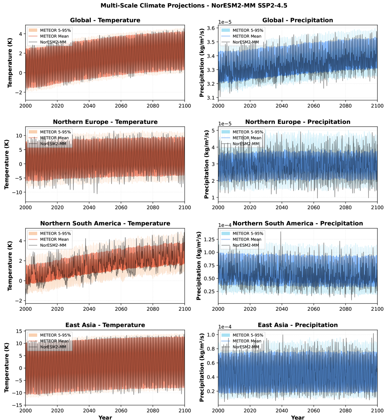
Figure 3. METEOR ensemble projections compared with NorESM2-MM SSP2-4.5 output for the extended period 2000–2100, showing that long-term regional climate trends are preserved by the emulator.
