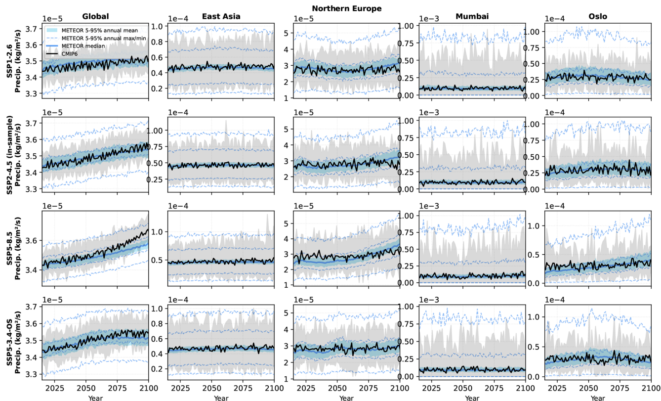
Figure 8. Out-of-sample precipitation validation for CNRM-ESM2-1 trained on SSP2-4.5. Layout and visual encoding as in Fig. 7: blue shading shows the 5 %–95 % range of annual means, dashed lines show the 5 %–95 % range of annual extrema, and the solid line shows the ensemble median. Precipitation changes are generally well captured, though SSP5-8.5 changes are somewhat underestimated. Results for other models are shown in Figs. S5–S8.
