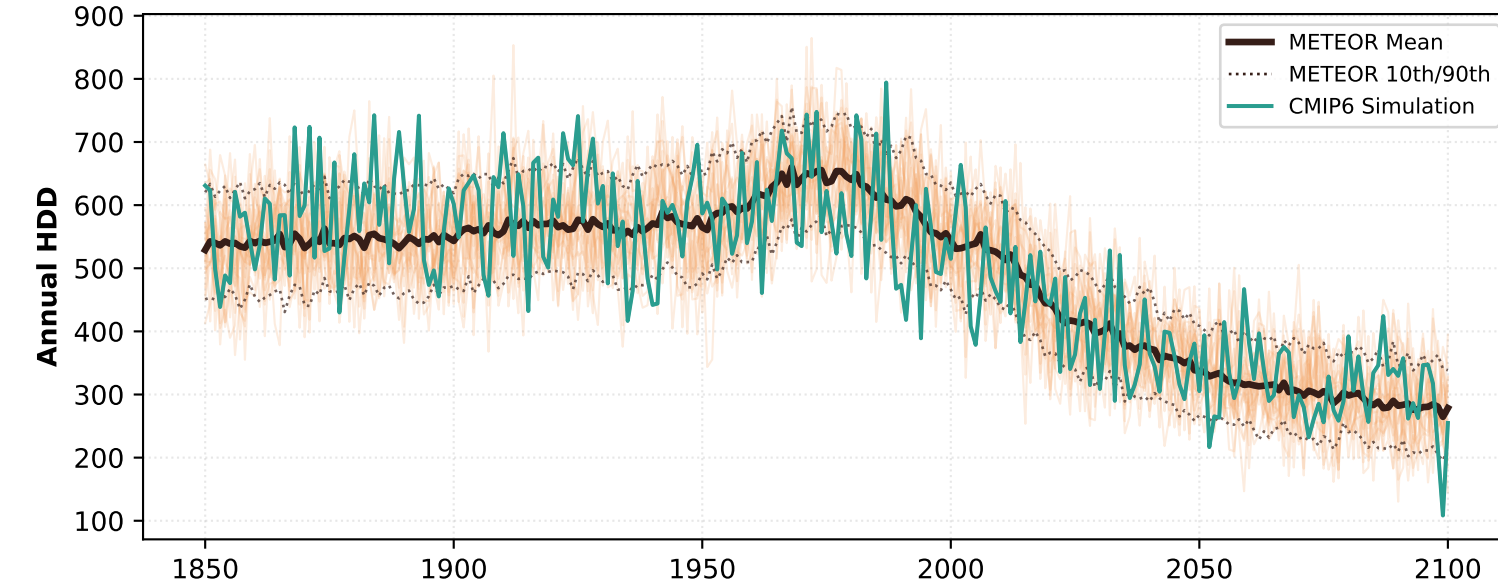
Beijing - HDD
