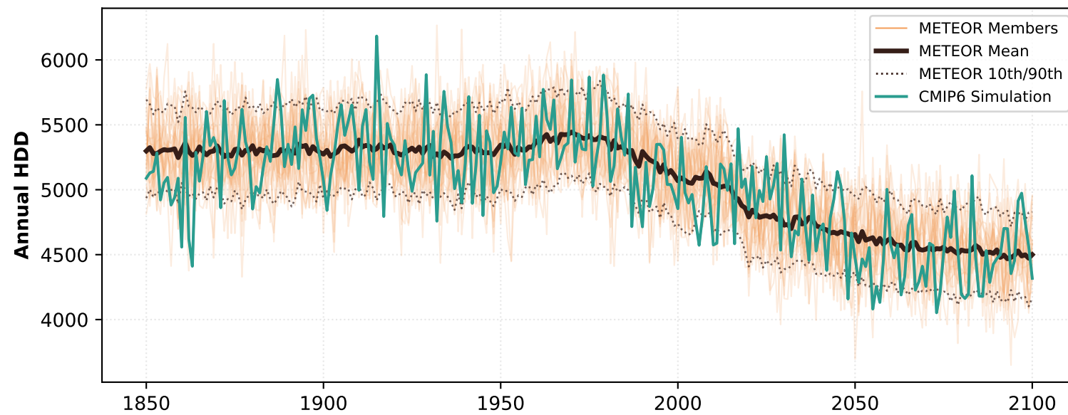
Delhi - HDD
