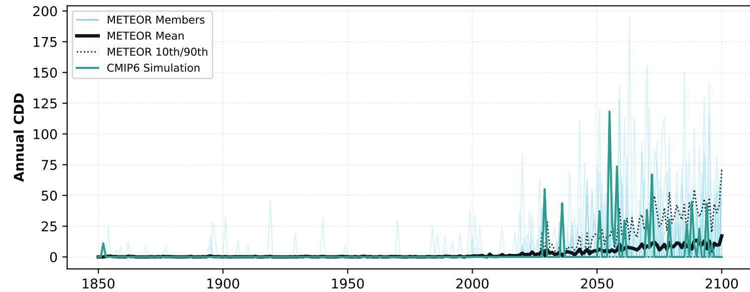
Delhi - CDD
