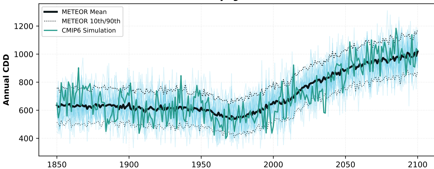
Beijing - CDD
