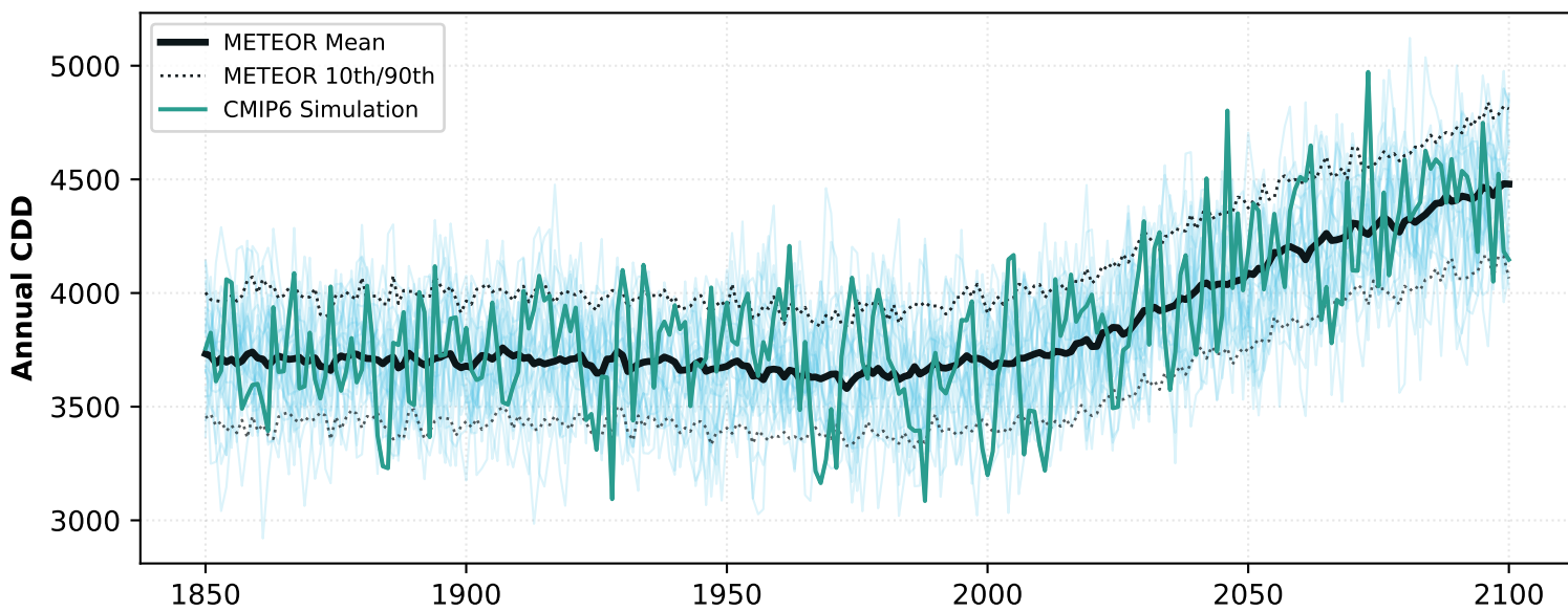
Cairo - CDD
