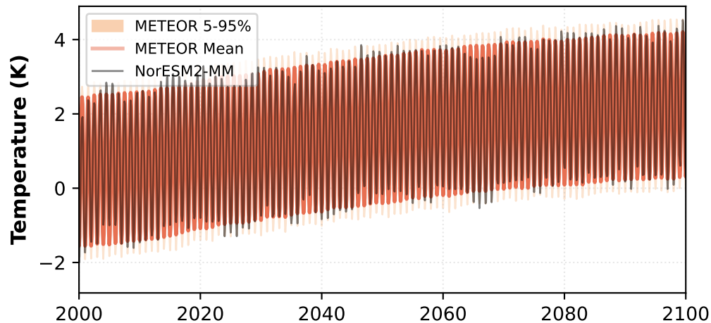
Global - Temperature
