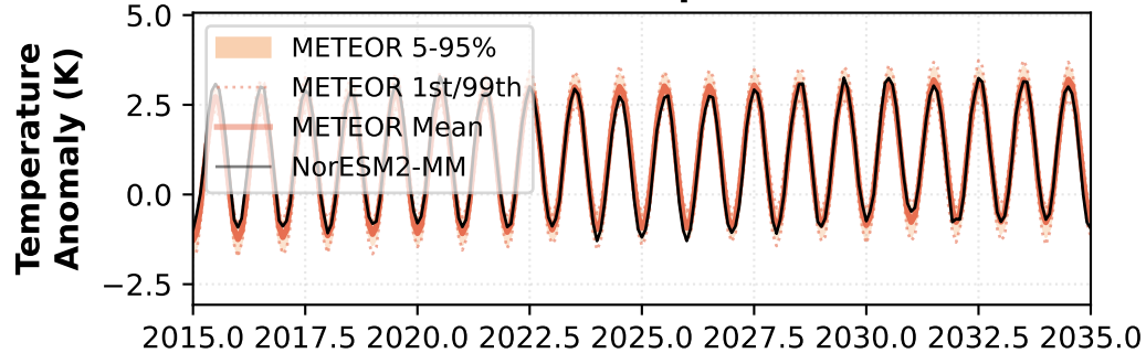
Northern South America - Temperature
