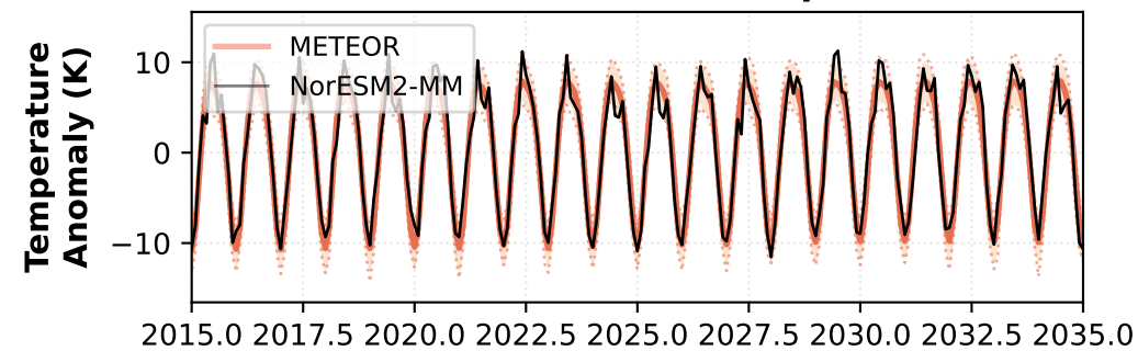
Beijing (39.9°, 116.4°) - Temperature
