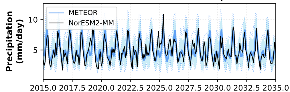
East Asia - Precipitation
