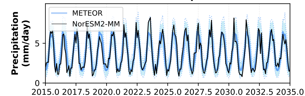
Oslo - Precipitation
