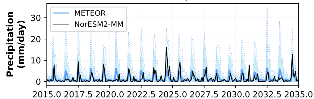
Beijing - Precipitation
