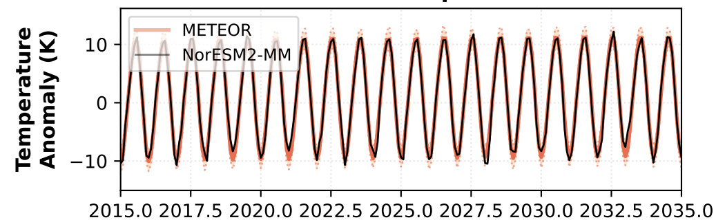
Oslo (59.9°, 10.8°) - Temperature
