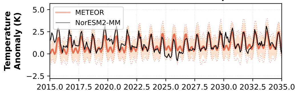
East Asia - Temperature
