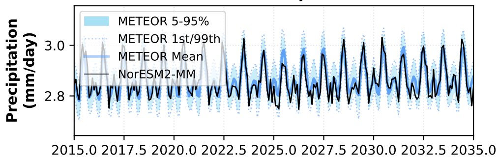
Northern South America - Precipitation
