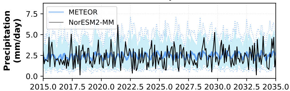
Delhi - Precipitation
