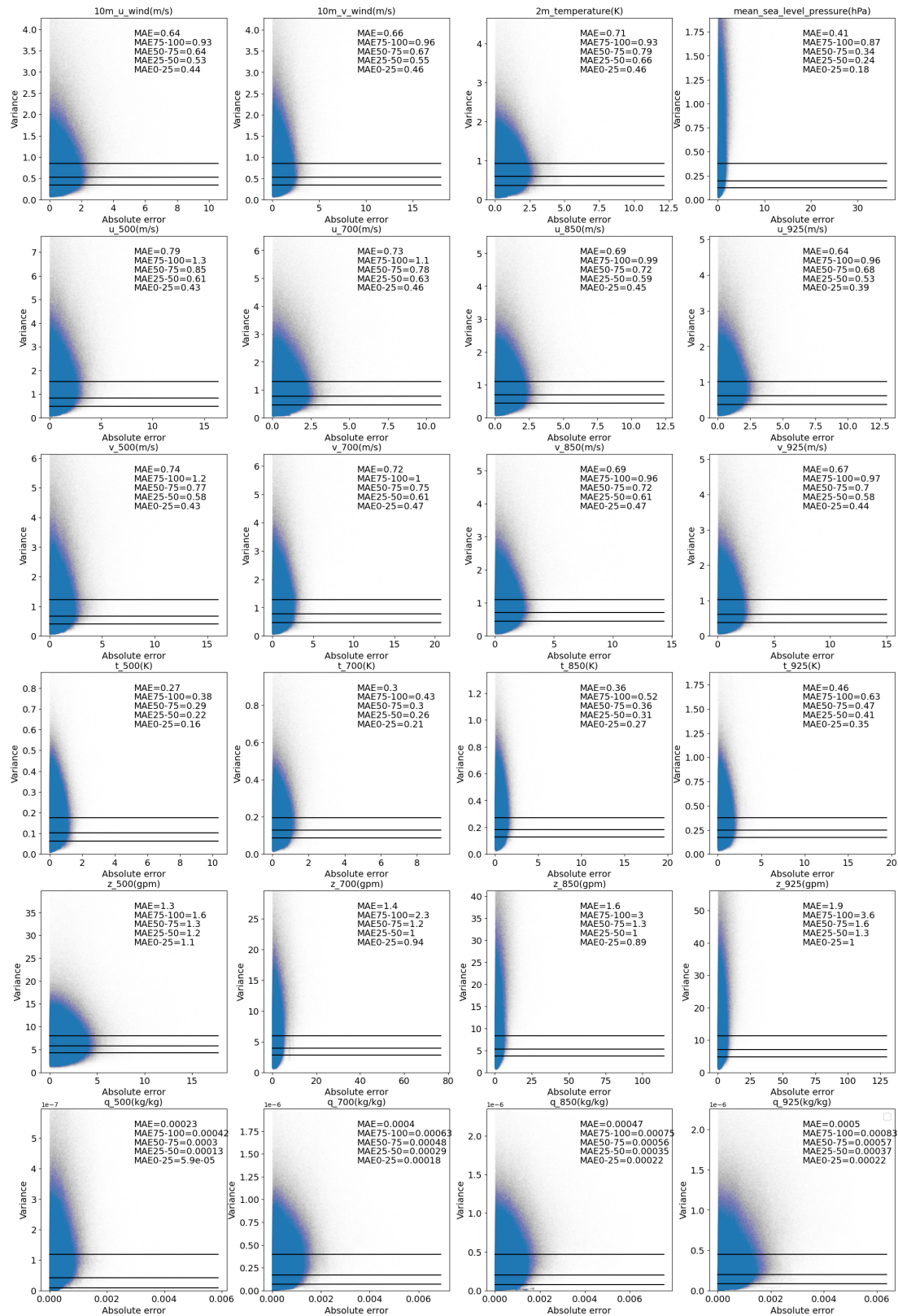
Figure 8. Correlation between the absolute error of Regression 4 and the variance of 20-member CorrDiff 4 predictions for the data from 1 October 2023 00:00 UTC. Each point in the figure corresponds to a grid point. The three black lines in each subplot represent the 75th, 50th and 25th percentile of the variance. These three lines separate the grid points into four groups. MAE75-100 is the MAE of the grid points above the 75th line, MAE50-75 is the MAE of the grid points between the 50th and 75th line, etc.
