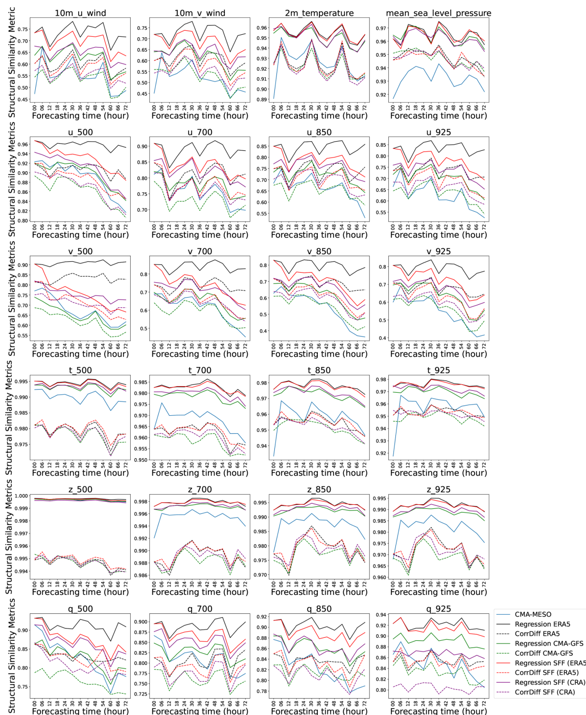
Figure 15. The structural similarity index measure of the 3 km forecasts that include the downscaled SFF forecasts (taking CRA1.5 or ERA5 as initial fields), the downscaled CMA-GFS forecasts and the CMA-MESO forecasts, using the 3 km reanalysis data as the ground truth. The downscaled ERA5 are also present for comparison. The downscaling models are Regression 4 and CorrDiff 4. The initialization time is 1 March 2023 00:00 UTC.
