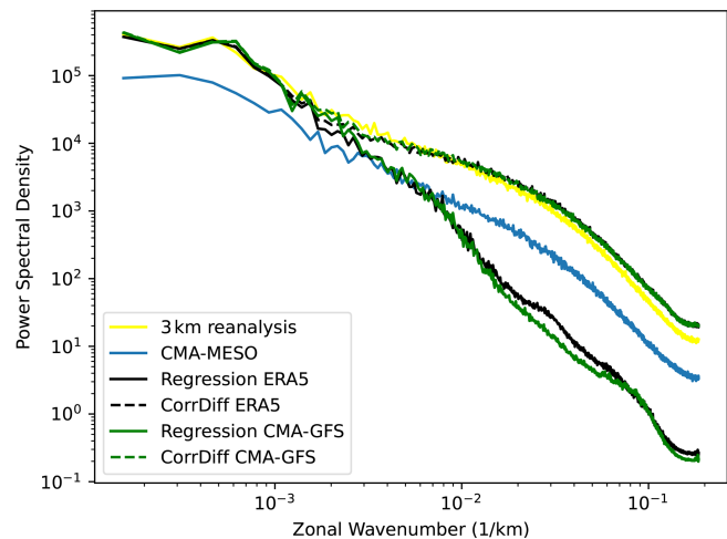
Figure 14. Power spectral density of the radar composite reflectivity. The downscaling models are Regression 2 and CorrDiff 2. The used 3 km reanalysis data and ERA5 are from 31 July 2023 00:00 UTC. The CMA-GFS and CMA-MESO forecasts are 24 h forecasts that are initialized at 30 July 2023 00:00 UTC.
