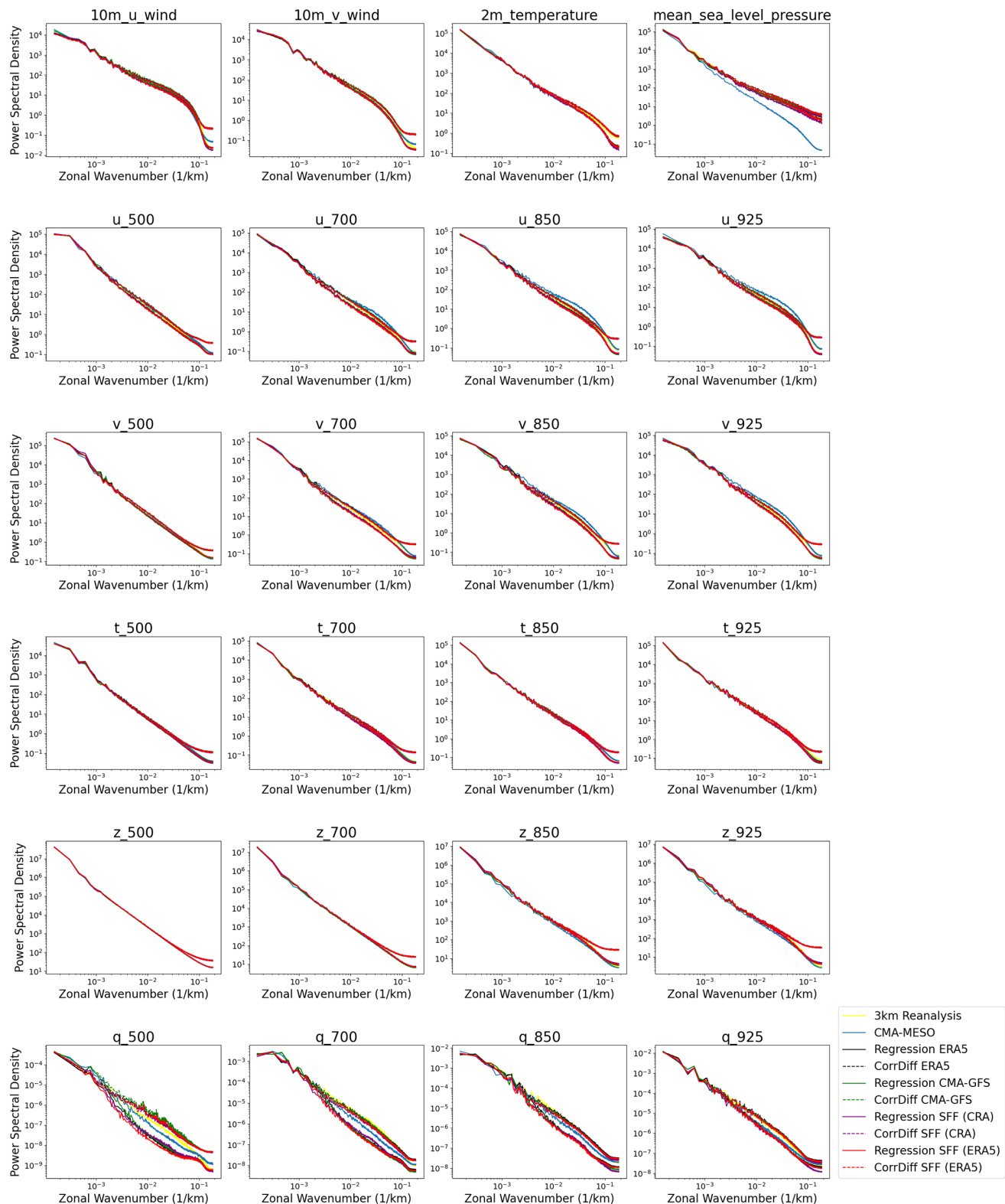
Figure 12. Power spectral density of the downscaling variables. The downscaling models are Regression 4 and CorrDiff 4. The used 3 km reanalysis data and ERA5 are from 2 March 2023 00:00 UTC. The CMA-GFS, CMA-MESO and SFF forecasts are 24 h forecasts that are initialized at 1 March 2023 00:00 UTC.
