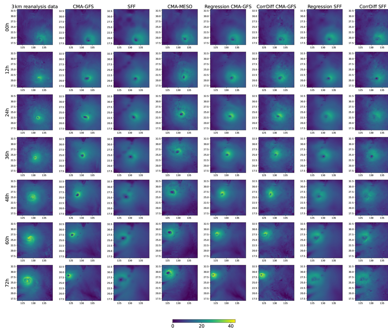
Figure 17. Illustration of the downscaling of CMA-GFS and SFF forecasts of Typhoon Khanun by Regression 4 and CorrDiff 4, compared to the 3 km reanalysis data, CMA-GFS, SFF and CMA-MESO. Figures represent 10 m wind speed. The initialization time is 30 July 2023 00:00 UTC. The initial fields of SFF are CRA1.5.
