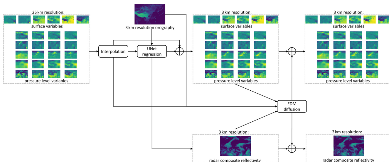
Figure 1. Illustration of the overall architecture of one of our trained CorrDiff models.
