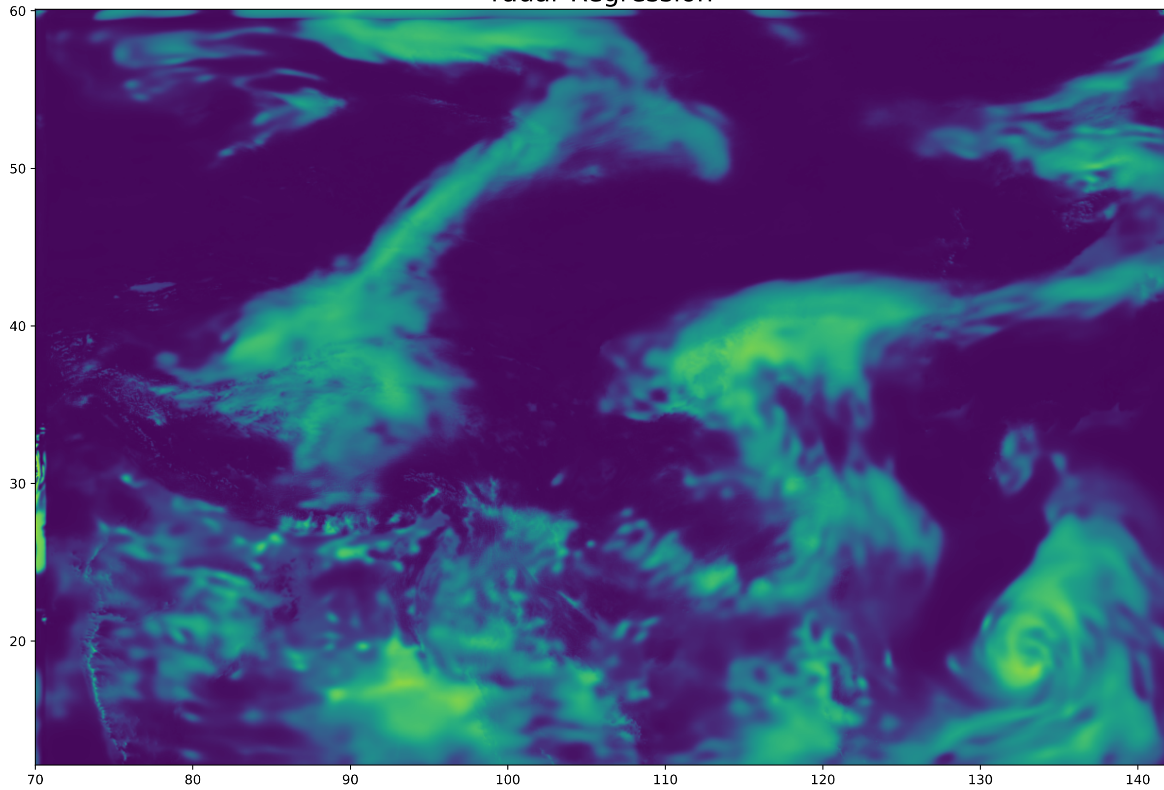
radar Regression
