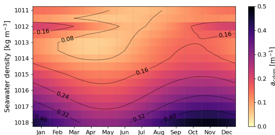
Figure 2. CDOM absorption forcing with regard to seawater density and day of the year.
