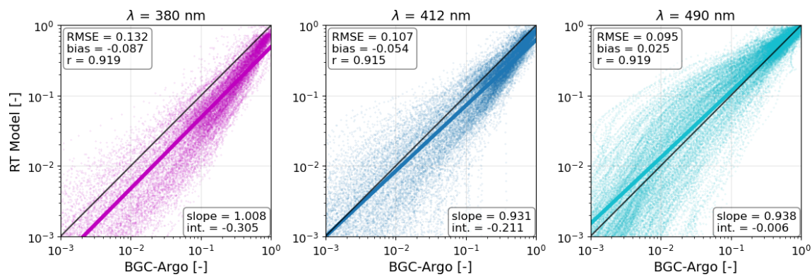
Figure 4. Logarithm of normalised downwelling irradiance from BGC-Argo data and the RT model in the RT configuration at the location of BGC-Argo floats between 2017 and 2020, for the upper 100 m. Irradiance measurements are normalised by the closest available value to the surface. The indexes of the BGC-Argo floats used are 6901866, 6903240 and 7900591. RMSE, correlation coefficient ( r ), regression slope and intercept are displayed for each wavelength. Scatter plots show 19 556, 25 628 and 43 268 points respectively for the 380, 412 and 490 nm wavebands.
