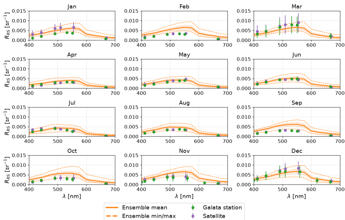
Figure 14. Monthly composites of sea surface reflectance spectra in 2018 at the Galata station (43.045° N, 28.193° E, Romania). Remote-sensing data are taken at the closest grid point to the Galata station. For observations, points represent the average R_{RS} for the month and bars represent one standard deviation in the data of the month. Model results are taken from the stochastic RT configuration with the ensemble mean in bold lines, the ensemble standard deviation in shaded, and the ensemble minimum and maximum in dotted lines.
