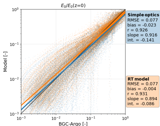
Figure 5. Logarithm of normalised E_0 derived from BGC-Argo PAR data with the simple optics and RT configurations at the location of BGC-Argo floats between 2017 and 2020, for the upper 100 m. RMSE, bias, correlation coefficient ( r ), regression slope and intercept are displayed. Scatter plots show 36 376 points. Normalisation is performed relative to the maximum value of the E_0 profile, which is the closest data from sea surface.
