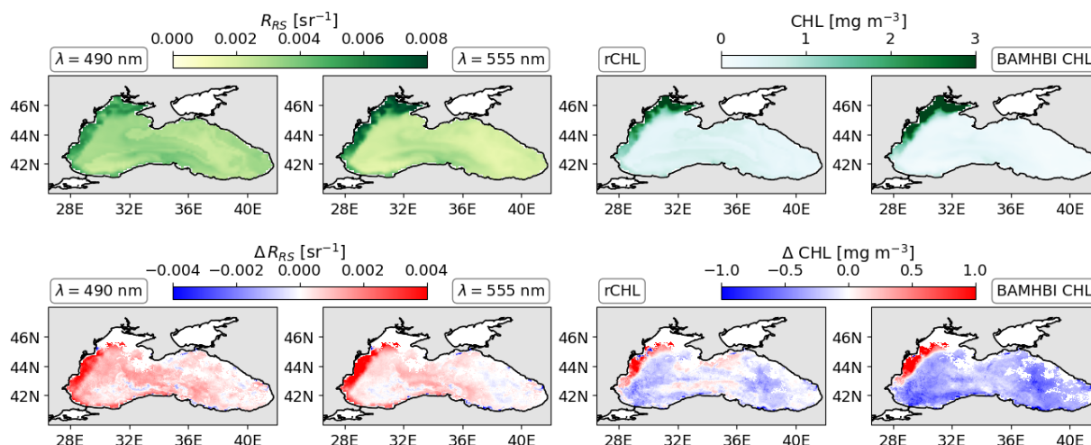
Figure 11. On the top row, maps of simulated R_{RS}(490) (1st column), R_{RS}(555) (2nd column), rCHL (3rd column) and BAMHBI chlorophyll (4th column) for the 27 October 2018. On the bottom row, difference with the remote-sensing product.
