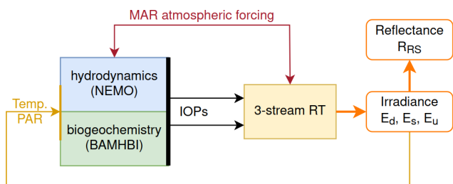
Figure 3. Coupling of the 3-stream RT model within the NEMO-BAMHBI framework. Forcing for physics and surface radiation are provided by a regional MAR simulation (see Sect. 3.2). In a configuration without a biogeochemical model, the IOPs would be forced from external data into the three-stream RT module.
