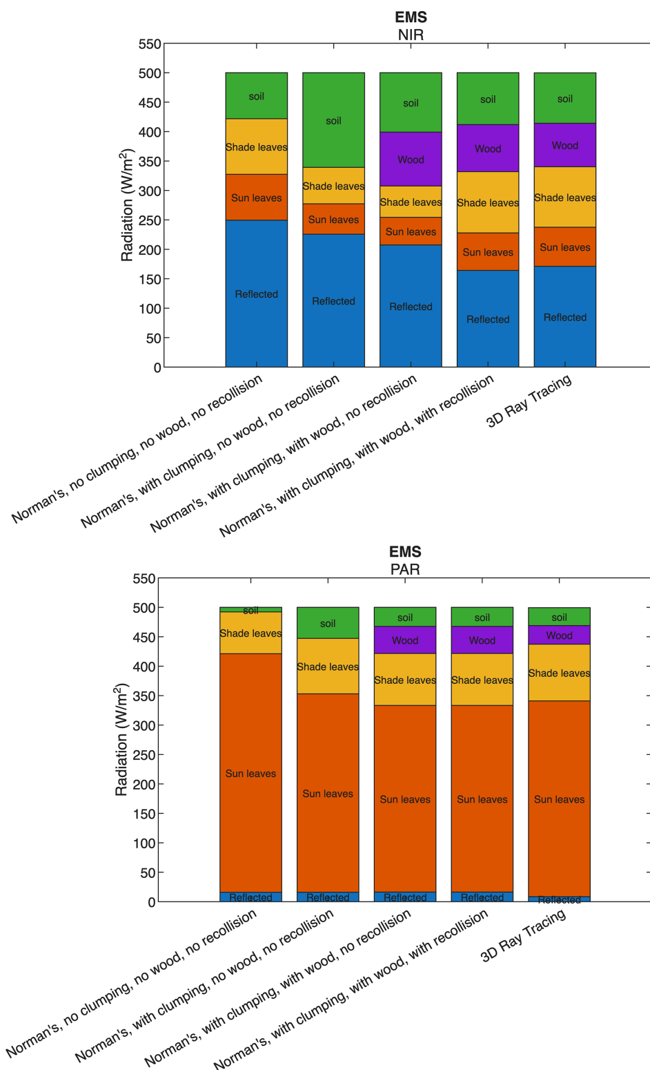
Figure 2. Budget for the proportions of NIR (top) and PAR (bottom) reflected, and absorbed by sunlit and shaded leaves, by wood and soil, simulated using the Norman model with four different configurations and the FLIESvox 3D ray tracing model. All simulations are for sun zenith angle of 35°, diffuse fraction of 20 % and incoming radiation of 500 W m -2 . Shown here are results for the Harvard Forest site (equivalent figures for all other sites are provided in the Supplement).
