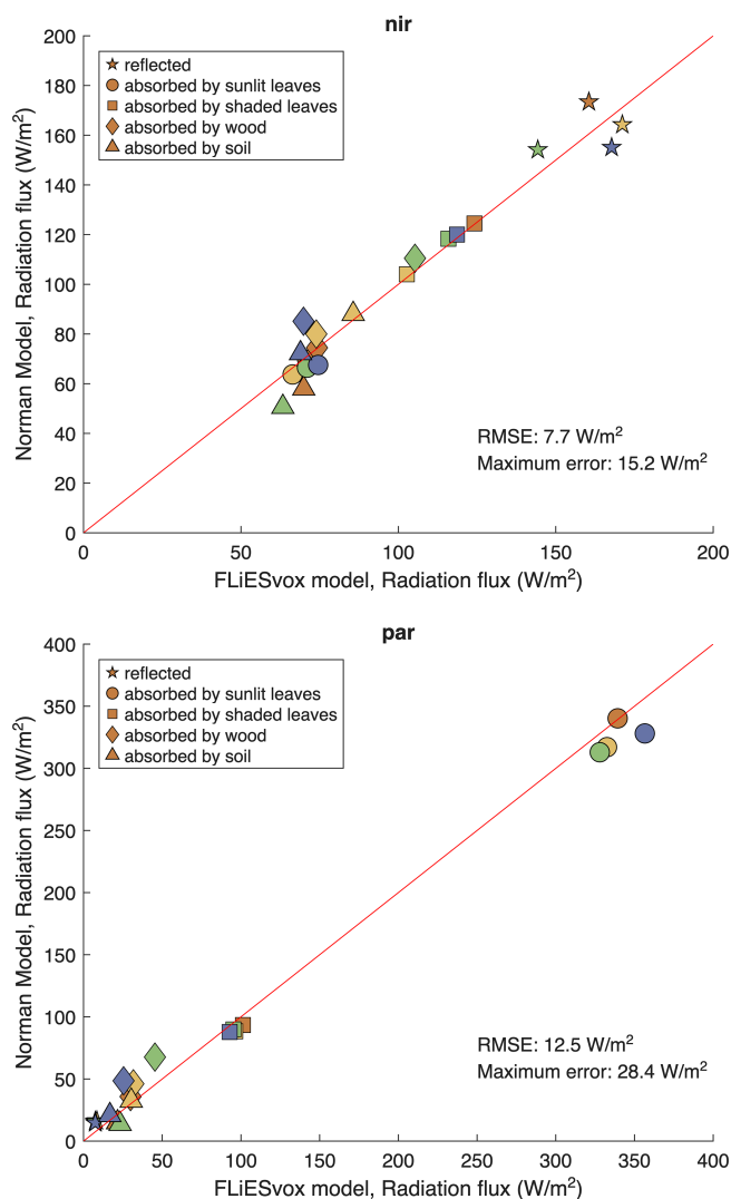
Figure 3. Correspondence between the total radiation fluxes reflected and absorbed for the modified Norman and FLiESvox models in the NIR (top) and PAR (bottom) for all sites. The Morgan Monroe site is in orange, Harvard Forest in yellow, Pasoh in green, and SERC in blue. The red line is 1 : 1.
