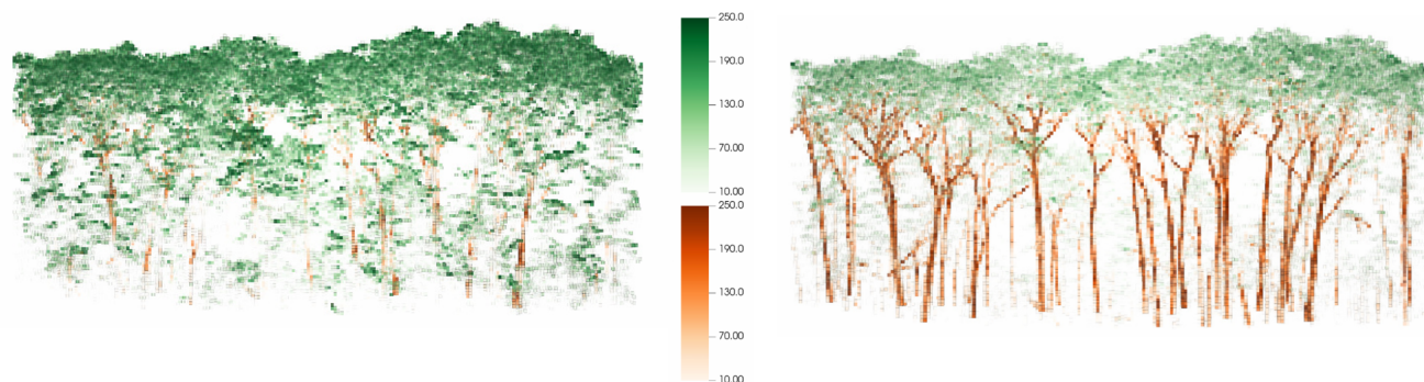
Figure 1. Examples of a 3D voxel-based mapping of absorbed radiation (in \text{W m}^{-2} ) by leaves (green) and wood (brown) in PAR (left) and NIR (right) as simulated by the FLiESvox 3D raytracing radiative transfer model at the Harvard Forest site.
