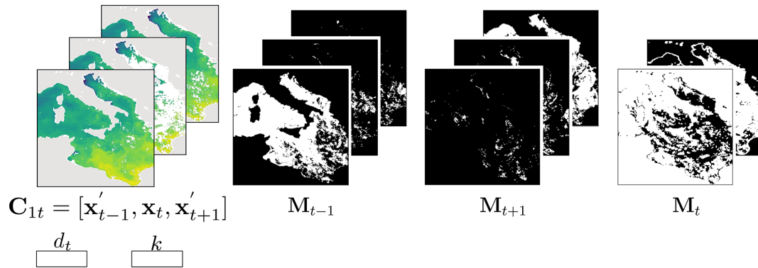
Figure 2. Context information fields provided to DIRECT at input. DIRECT uses a three-day SST window C_{1t} = [x'_{t-1}, x_t, x'_{t+1}] , with corresponding one-hot encoded masks M_{t-1} and M_{t+1} indicating the temporal origin of filled pixels, and M_t marking observed versus missing values in the central frame. Additional conditioning is provided by the day-of-year ( d_t ) and the flow timestep k .
