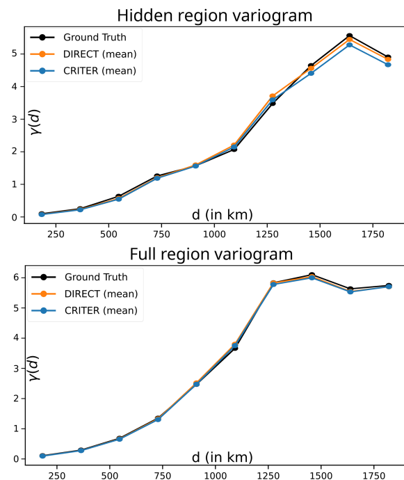
Figure 13. Visualization of the spatial scales and correlation properties analysis. Top plot: empirical semivariograms computed exclusively over hidden regions. Bottom plot: semivariograms computed over the full SST domain. Each curve represents the mean semivariance across 10 different mask realizations.
