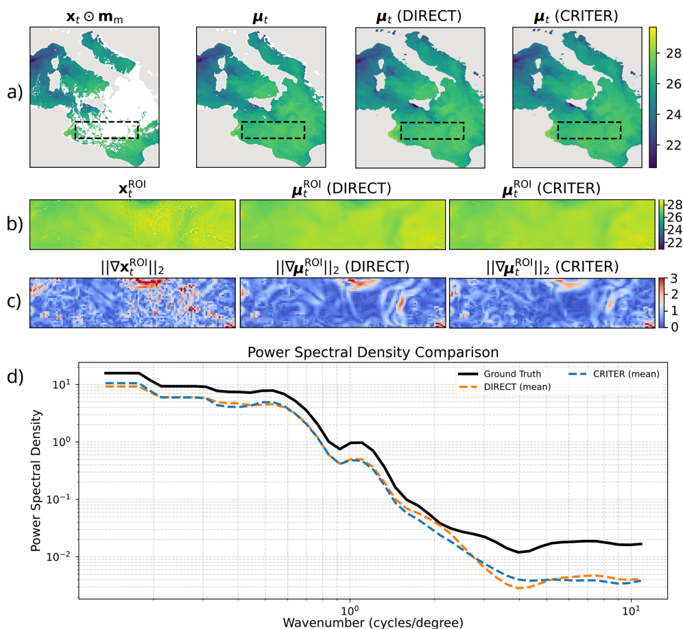
Figure 11. Power spectral density (PSD) analysis for a selected region of interest (ROI). (a) Masked SST input, ground truth field, and reconstructions from DIRECT and CRITER. (b) Zoomed views of the ROI. (c) Gradient magnitudes \|\nabla \mu_t^{\text{ROI}}\|_2 highlighting structural differences. (d) Isotropic PSD computed from the plane-detrended ROI fields using an FFT with a Blackman–Harris window. The displayed curves represent the average spectral density across 10 independent mask realizations.
