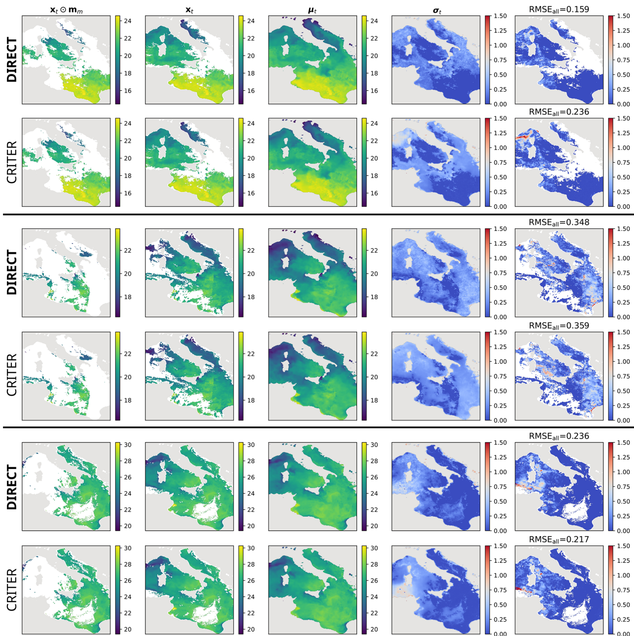
Figure 6. Comparison of DIRECT and CRITER reconstructions on the Mediterranean region. The columns show (from left to right): the partially observed input ( x_t \odot m_m ), the ground truth x_t , the reconstruction \mu_t , the estimated uncertainty \sigma_t , and the absolute reconstruction error ( \text{RMSE}_{\text{all}} ). All values are in ^{\circ}\text{C} .
