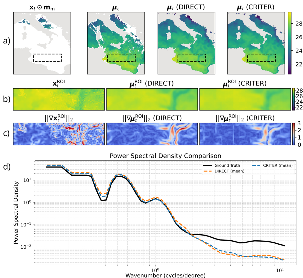
Figure 10. Power spectral density (PSD) analysis for a selected region of interest (ROI). (a) Masked SST input, ground truth field, and reconstructions from DIRECT and CRITER. (b) Zoomed views of the ROI. (c) Gradient magnitudes \|\nabla \mu_t^{\text{ROI}}\|_2 highlighting structural differences. (d) Isotropic PSD computed from the plane-detrended ROI fields using an FFT with a Blackman–Harris window. The displayed curves represent the average spectral density across 10 independent mask realizations.
