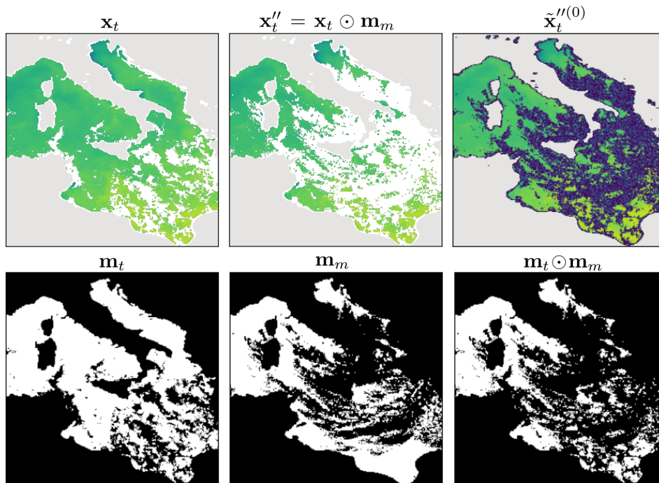
Figure 5. First row: ground truth incomplete central day observation ( x_t ), simulated central day observation ( x_t'' ), noised initialized simulated central day observation ( \tilde{x}_t^{(0)} ). Second row: mask denoting valid observations in ground truth observation ( m_t ), sampled mask from a different day ( m_m ), mask denoting observed regions in the simulated central day observation ( m_t \odot m_m ).
