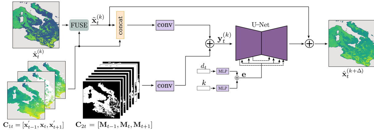
Figure 4. Overview of the DIRECT architecture. The SST field \hat{x}_t^{(k)} estimated at k th iteration is accompanied by the temporal context C_{1t} and the time-stamp masks C_{2t} , seasonal context d_t , and the current flow iteration value k . The FUSE rectified reconstruction \tilde{x}_t^{(k)} is concatenated with context frames C_{1t} and summed with the embedded origin masks C_{2t} to form the network input. Token e modulates the U-Net via FiLM (Perez et al., 2018). The network output updated the initial SST estimate into \hat{x}_t^{(k+\Delta)} by Euler integration.
