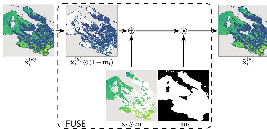
Figure 3. The FUSE operation. At each integration step k , the current estimate \hat{x}_t^{(k)} is merged with the original observations x_t . This ensures that measured pixels remain preserved (non-corrupted) while the model updates the missing regions.
