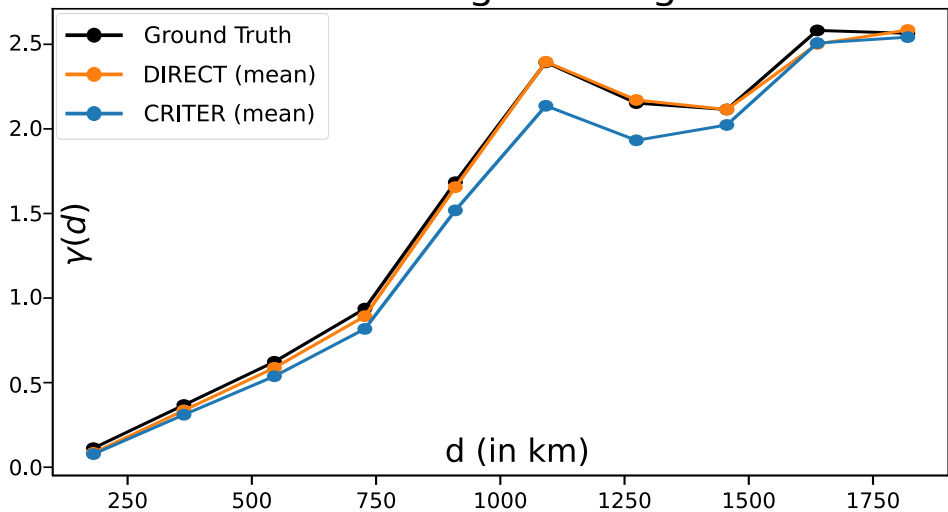
Full region variogram
