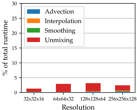
Bilinear method
