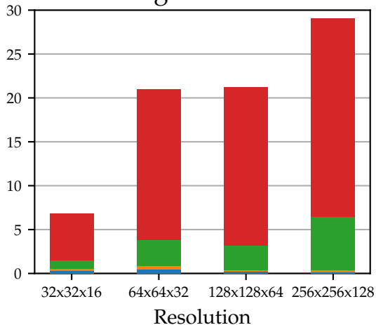
Integral method
