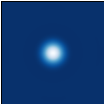
Bilinear method
