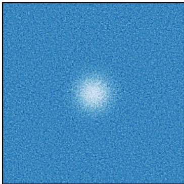
Marker-in-cell
