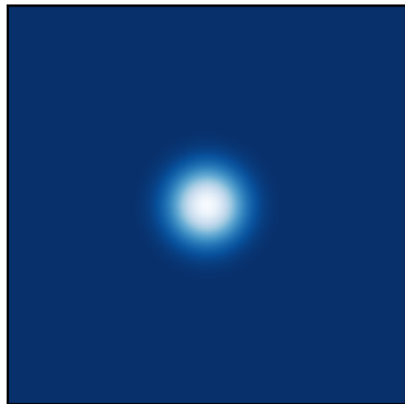
Integral method
