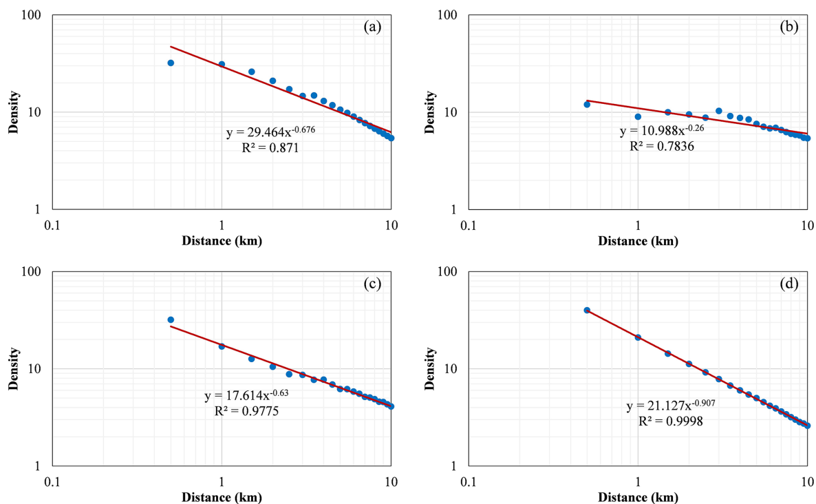
Figure 5. Log–log plots of deposits density vs. buffer width: (a) faults, (b) Yanshanian intrusions, (c) Taihua rock groups strata, and (d) Xiong'er rock groups strata.
