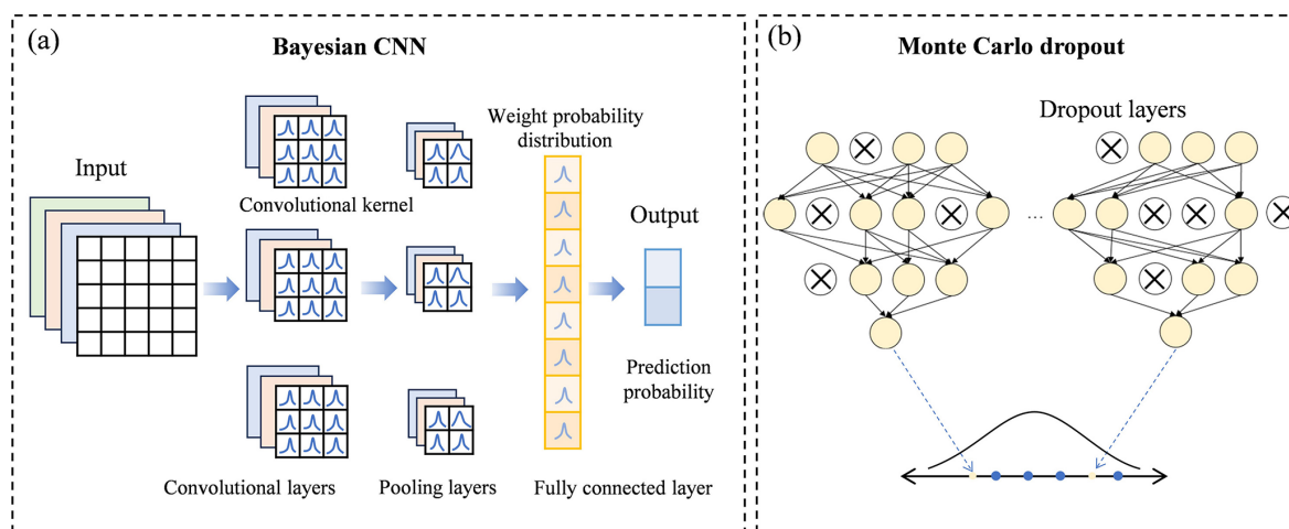
Figure 3. A workflow of model uncertainty modeling: (a) Bayesian CNN, (b) Monte Carlo dropout. Model uncertainty is quantified by treating network weights probabilistically in a Bayesian CNN. Bayesian inference is approximated using Monte Carlo dropout by activating dropout during inference and performing multiple stochastic forward passes to estimate uncertainty.
