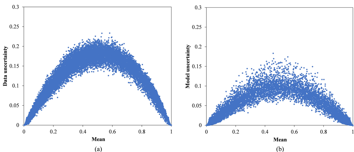
Figure 16. Scatter plots of mean probability versus uncertainty: (a) data uncertainty, (b) model uncertainty. The x -axis denotes the mean predictive probability obtained from multiple stochastic forward passes and the y -axis denotes the corresponding uncertainty (entropy).
