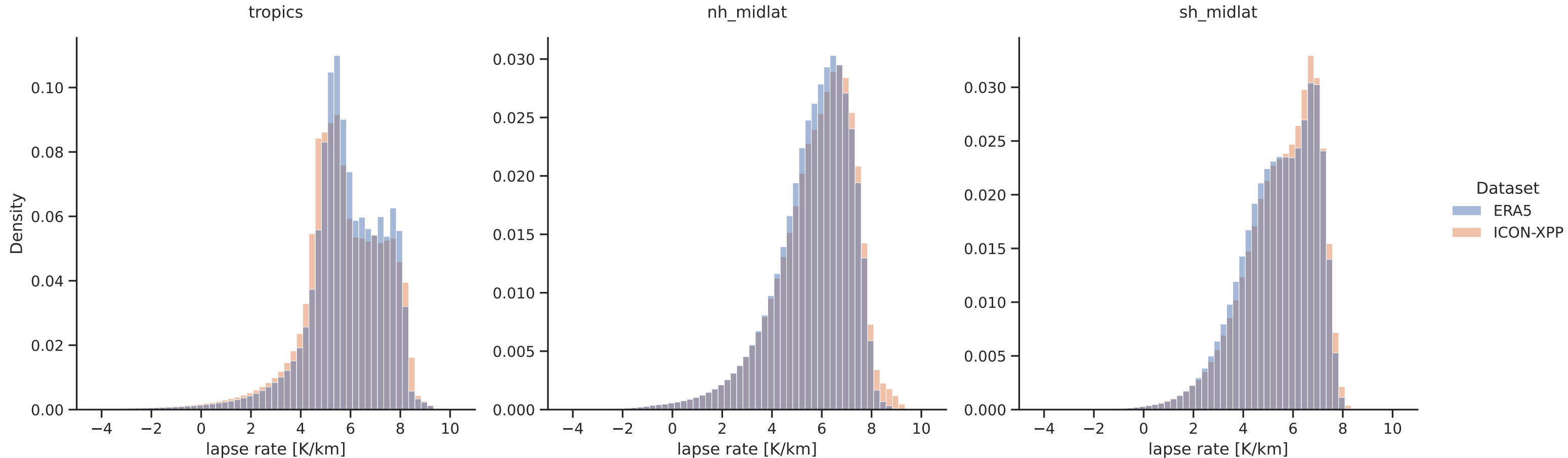
PDF of lapse rates (850 hPa to 250 hPa)
