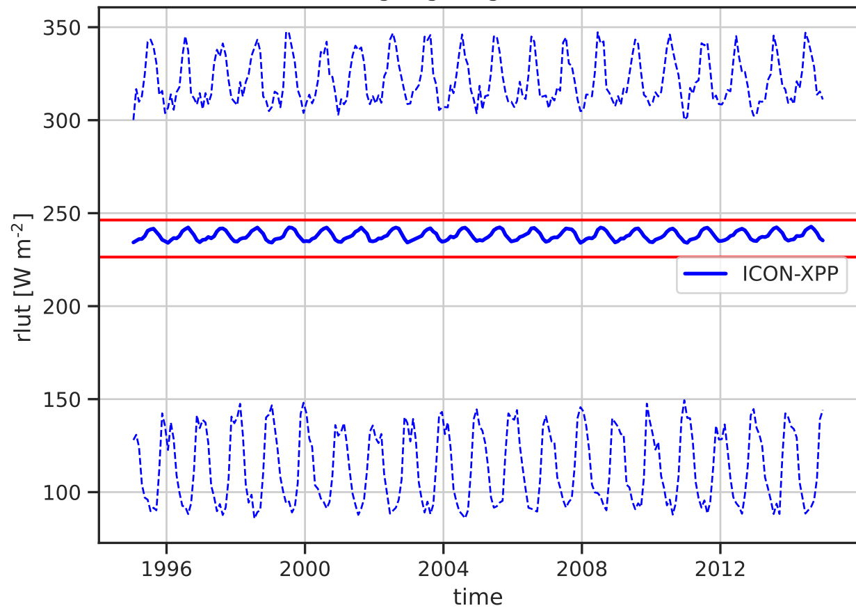
TOA Outgoing Longwave Radiation
