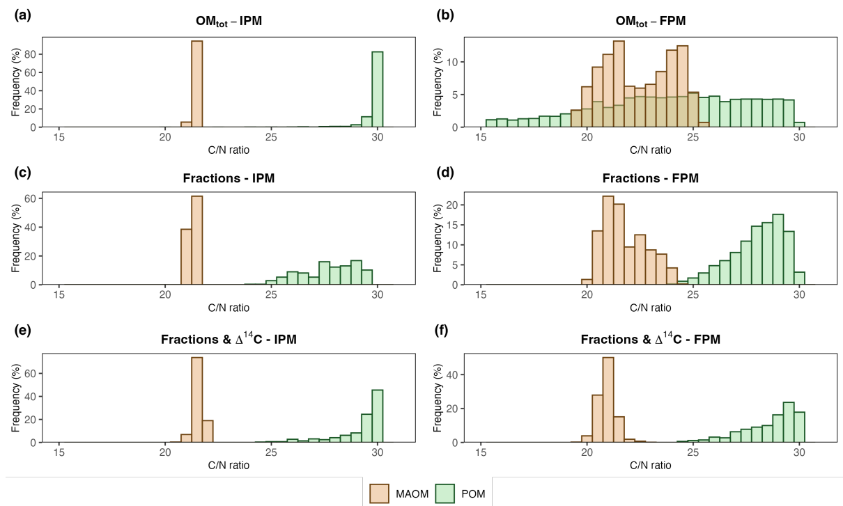
Figure S4. The simulated C/N ratio of particulate organic matter (POM) and mineral-associated organic matter (MAOM) for the behavioural SOM models at steady state (i.e., the last year before OC inputs were doubled). The calibration scenario Fractions and Fractions and \Delta^{14}\text{C} (second and third row) were calibrated using an assumed C/N ratio of 29 for POM, and 20 for MAOM. The left column shows the results for the identifiable parameter models (IPM), while the right column shows the results for the full parameter model (FPM).
