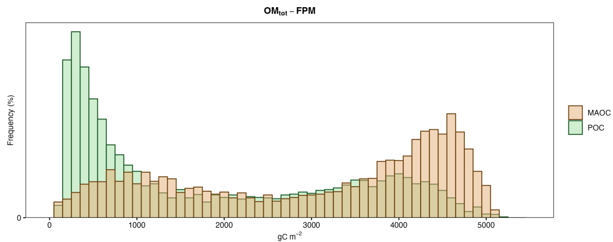
Figure S3. The simulated size of particulate organic carbon (POC) and mineral-associated organic carbon (MAOC) pools for the behavioural SOM models at steady state (i.e., the last year before OC inputs were doubled) for the SOM model optimised using only data on total SOC and N while calibrating all model parameters (full parameter model; FPM).
