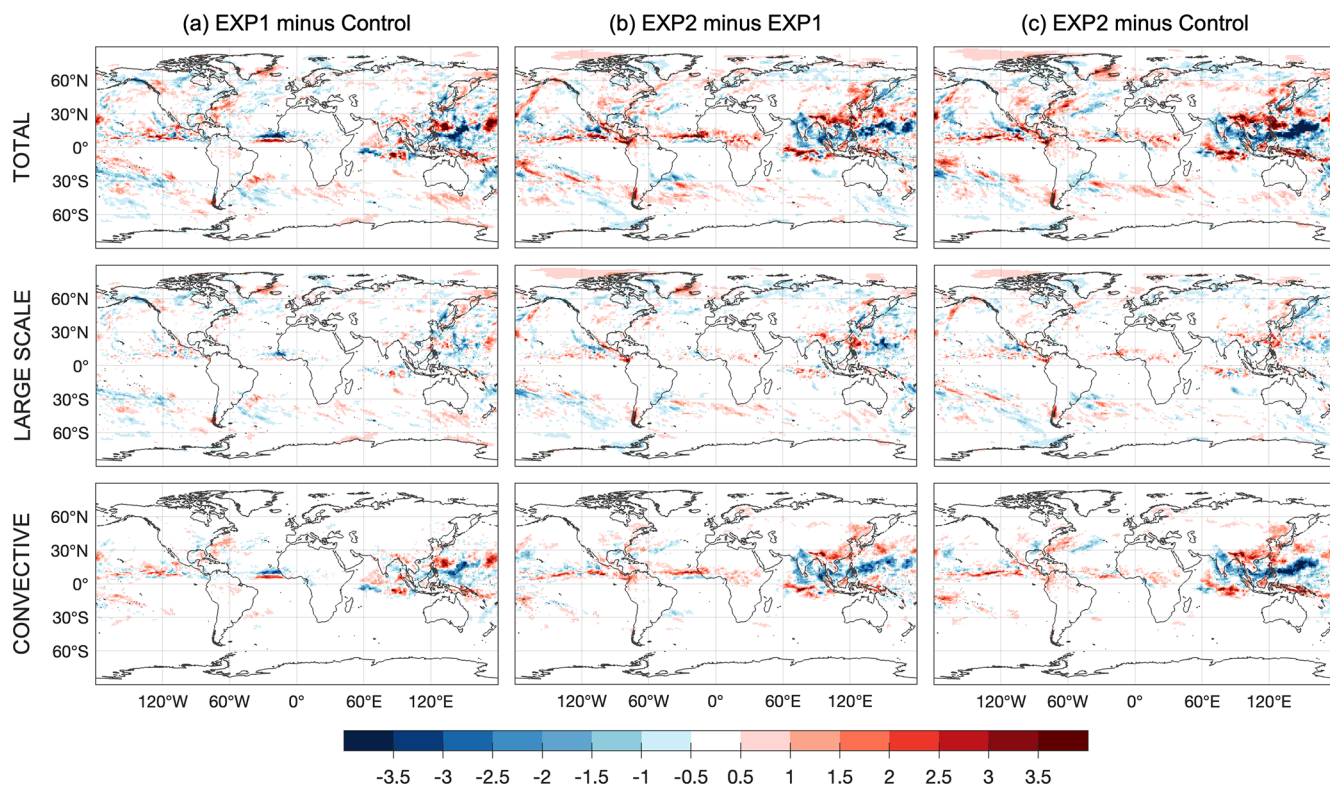
Figure 13. Six-year averaged (2012–2017) differences in total precipitation (top row; \text{mm d}^{-1} ), large-scale precipitation (middle row; \text{mm d}^{-1} ) and convective precipitation (bottom row; \text{mm d}^{-1} ) for August in UFS-Chem. (a) Effect of aerosol radiative feedback (EXP1 minus Control). (b) Aerosol indirect effects (EXP2 minus EXP1). (c) Combined effect of aerosol radiative feedback and aerosol indirect effects (EXP2 minus Control).
