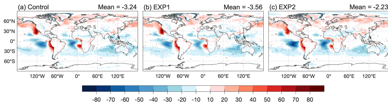
Figure 10. Six-year averaged (2012–2017) TOA net radiative flux bias compared with CERES for August in UFS-Chem for the (a) Control, (b) EXP1, and (c) EXP2 experiments.
