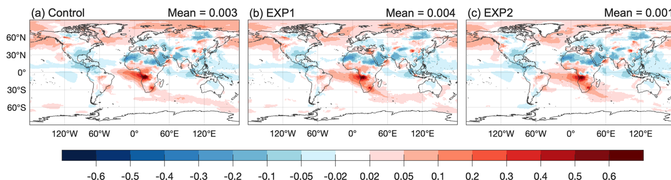
Figure 8. The same as in Fig. 6, but averaged over the six-year of August (2012–2017).
