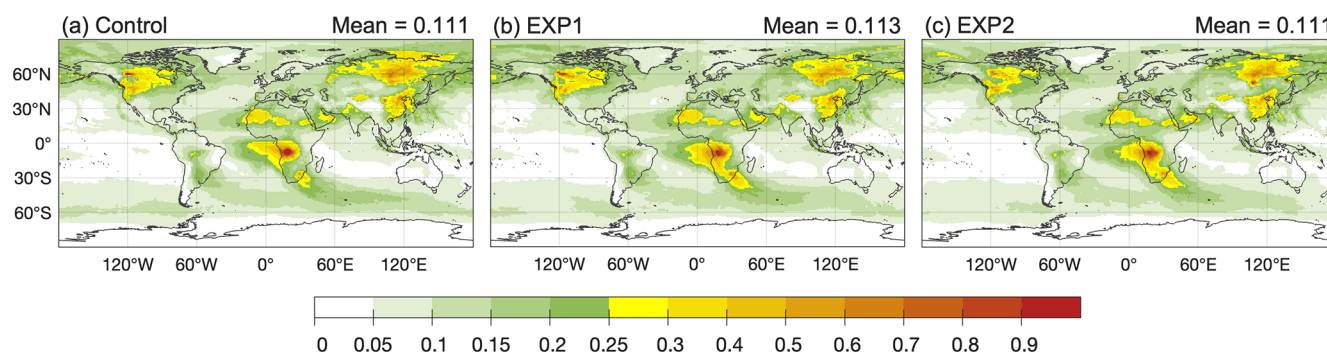
Figure 9. The same as in Fig. 8, but for AOD RMSE.
