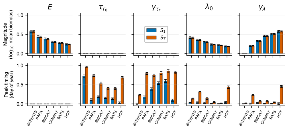
Figure 6. Sobol sensitivity indices of the biomass to the five biological parameters at the six stations, ordered from coldest to warmest. The rows are the two output descriptors, the magnitude (base-10 logarithm of the mean biomass, top) and the seasonal peak timing (day of year of the maximum, bottom). The columns are the five parameters E , \tau_{r0} , \gamma_{\tau_r} , \lambda_0 and \gamma_\lambda . In each panel the blue bars are the first-order index S_1 , the share of output variance due to that parameter alone, and the orange bars the total-order index S_T , which adds its interactions with the other parameters. Error bars are 95 % bootstrap confidence intervals. The indices are computed from a Saltelli design of N = 8192 base samples, that is 57 344 model runs at each station. The magnitude is governed by the energy transfer and the two mortality parameters, the peak timing by the two recruitment parameters.
