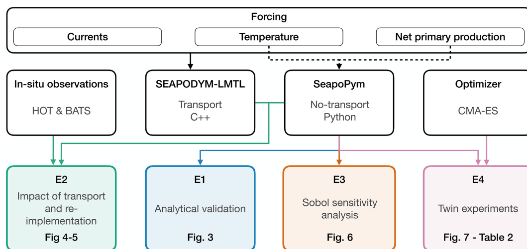
Figure D1. Overview of the SeapoPym modeling and experimental workflow. Temperature and NPP drive both models, whereas the currents drive only the SEAPODYM-LMTL model (with transport, C++). The dashed link marks that SeapoPym (without transport, Python) omits the currents. Each experiment is color-coded and linked to the components it uses, with the figures that report it. E1 (analytical validation, Fig. 3) and E3 (Sobol sensitivity analysis, Fig. 6) exercise the SeapoPym model. E2 (impact of transport and re-implementation, Figs. 4–5) compares SeapoPym with the operational SEAPODYM-LMTL product and with the in-situ observations at HOT and BATS. E4 (twin experiments, Fig. 7 and Table 2) recovers the SeapoPym parameters with the CMA-ES optimizer from synthetic observations generated by SeapoPym itself.
