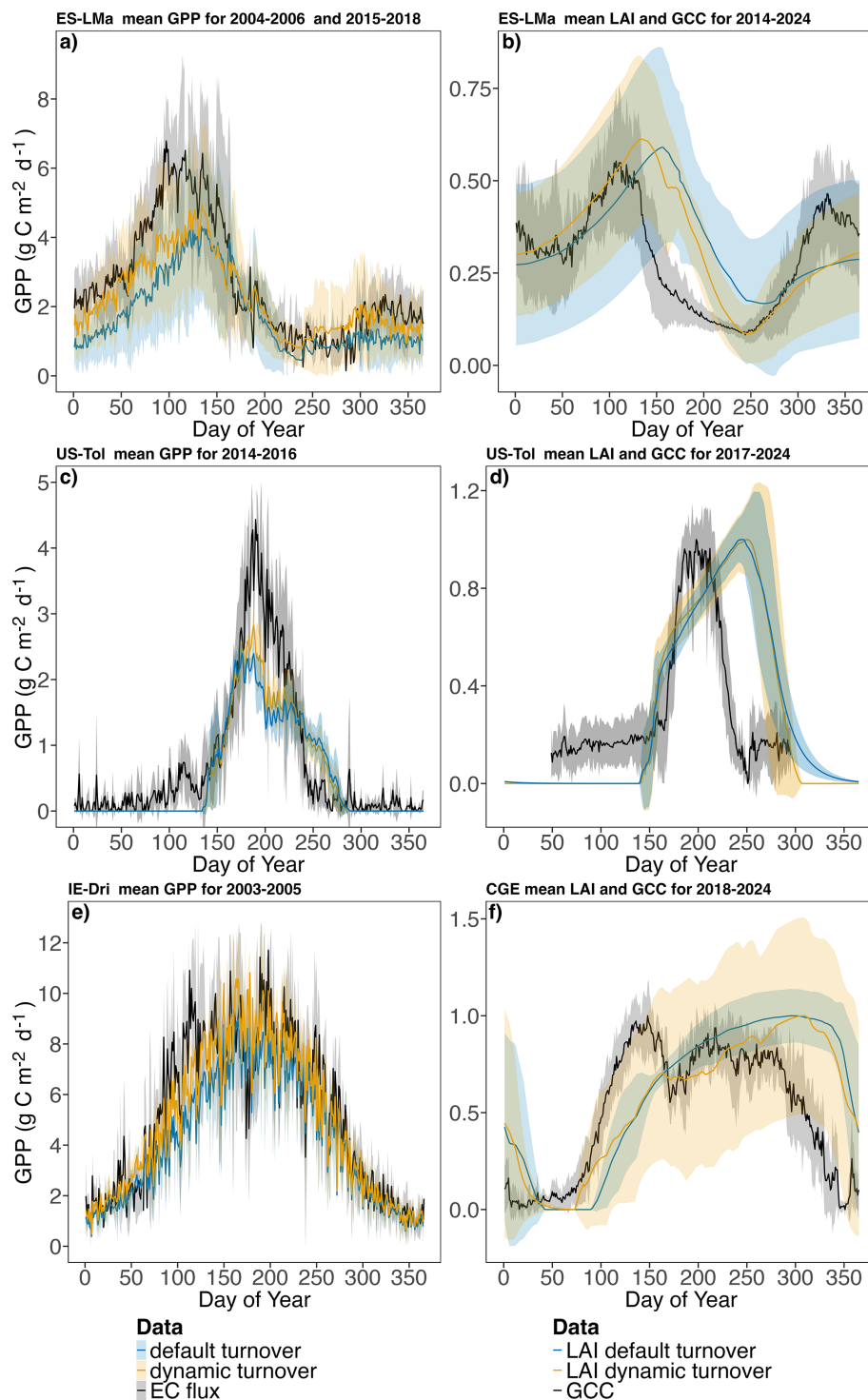
Figure 2. Default and dynamic turnover model performance at sites ES-LMa (a), US-Tol (c) and IE-Dri (e) with mean daily GPP and ES-LMa (b), US-Tol (d) and CGE (f) with normalized mean daily LAI and GCC. Shaded areas show one standard deviation.
