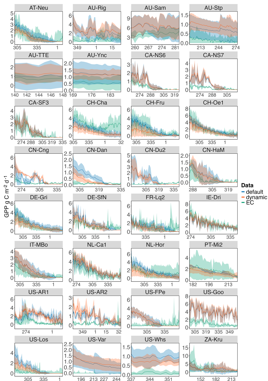
Figure 6. End of season (EOS) fit of modeled mean daily GPP (g C m -2 d -1 ; blue: default and orange: dynamic model) and flux tower mean daily GPP (g C m -2 d -1 ; green) at 32 PLUMBER2 sites (for explanation of site IDs see Ukkola et al., 2021). The EOS period displayed for each data source is defined as the period between the calculated mean EOS date (see Table 6) and the first mean minimum GPP date following it and for comparison the overlap of all end of season periods (EC flux, default and dynamic model) is used here. The shaded areas represent 1 SD. The EOS dates are calculated using “ phenofit ” package (Kong et al., 2022) and only sites with one EOS date per year have been selected.
