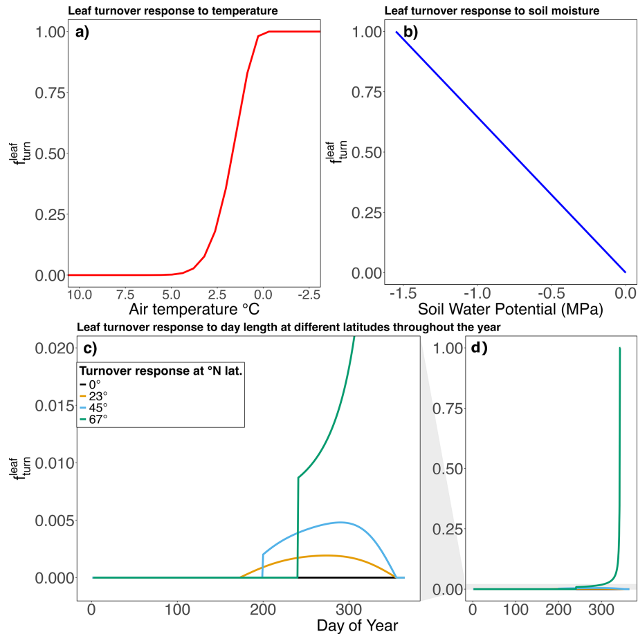
Figure 1. The individual impacts of the three environmental stressors: (a) air temperature (see Eq. 6), (b) soil moisture (see Eq. 7), and (c, d) day length (see Eqs. 13–15) on leaf turnover ( f_{\text{turn}}^{\text{leaf}} ) in the dynamic model (see Sect. 2.3). The combined f_{\text{turn}}^{\text{leaf}} from these three components is shown in Eq. (16). The leaf turnover response to day length (c, d) is shown for example latitudes on the northern hemisphere, but the model provides continuous global coverage for all latitudes. Panel (d) shows the full range of light induced leaf turnover and panel (c) is an enlarged view of this to show the exact pattern as well as timing of leaf turnover response to changing day length.
