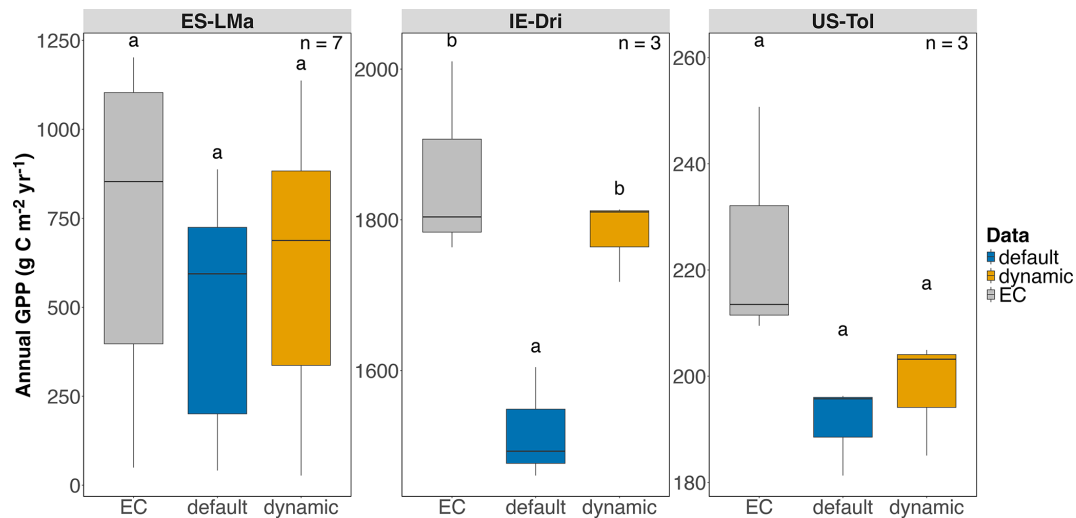
Figure 3. Mean annual GPP and 25th- and 75th-percentile for ES-LMa, IE-Dri and US-Tol for the two models (default and dynamic) as well as EC flux data with number of available years of data ( n , see Table 2). The displayed simulations for the default and dynamic model matches the time series range of the EC data. Letters above each bar indicate statistical significance (Tukey's p < 0.05 ), where groups sharing the same letter are not significantly different and groups with different letters represent a significant difference between means (for p values see Table 4).
