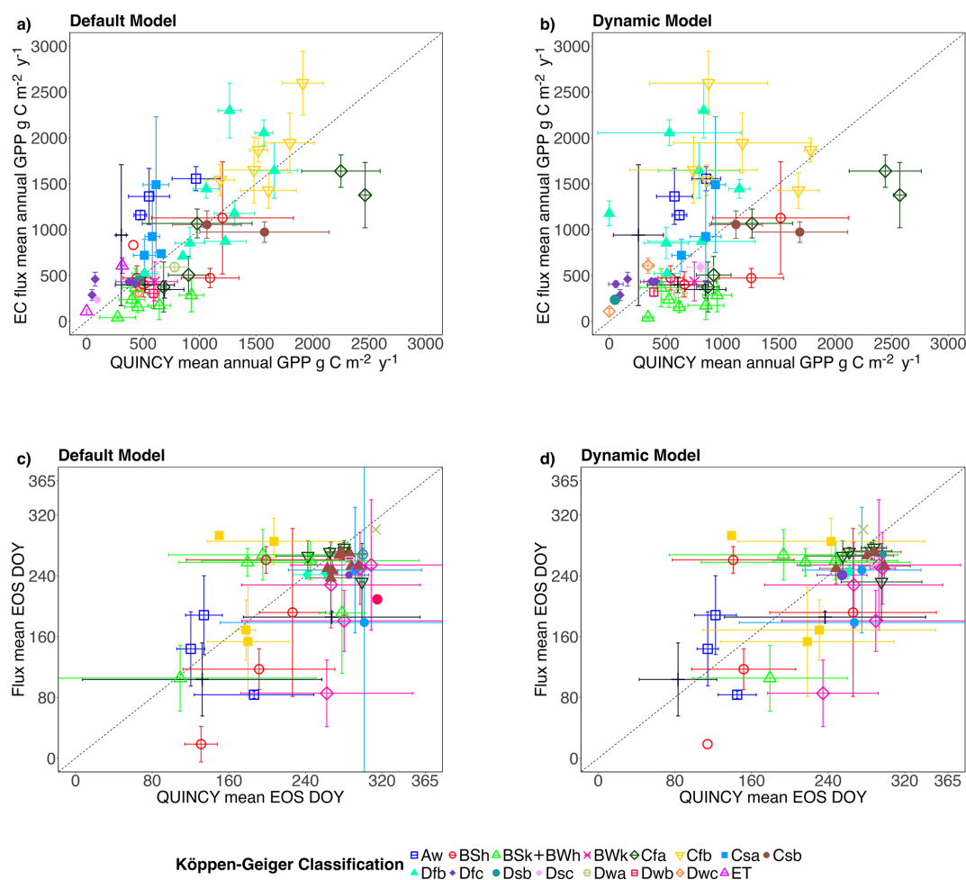
Figure 5. Capability of the default and the dynamic turnover model to predict mean annual GPP (a, b) compared to observed EC flux mean annual GPP ( \text{g C m}^{-2} \text{yr}^{-1} ) at 56 sites (see Table C2) as well as mean EOS dates (c, d) at 37 sites (see Table 5) of the default and the dynamic model and compared with EC flux EOS dates. EOS dates were calculated from daily GPP using “ phenofit ” package (Kong et al., 2022). The number of sites is lower in the panel (c) and (d) due to the exclusion of sites with dual growing seasons or where no EOS could be detected. This is documented in detail in Sect. 2.4.3. Error bars are 1 SD representing inter-annual variation and the colors and point shapes represent Köppen-Geiger climate zones. The climate zones displayed are: Aw: Tropical Savanna, As: Tropical Dry Summer, BSh: Hot Semi-Arid, BSk: Cold Semi-Arid, BWk: Hot Desert, BWk: Cold Desert, Cfa: Humid Subtropical, Cfr: Temperate Fully Humid Warm Summer, Csa: Hot-Summer Mediterranean, Csb: Warm-Summer Mediterranean, Dfb: Humid Continental Warm Summer, Dfc: Subarctic Cold Summer, Dwa: Continental Dry Winter Hot Summer, Dwb: Continental Dry Winter Warm Summer, Dwc: Continental Dry Winter Cold Summer, ET: Tundra.
