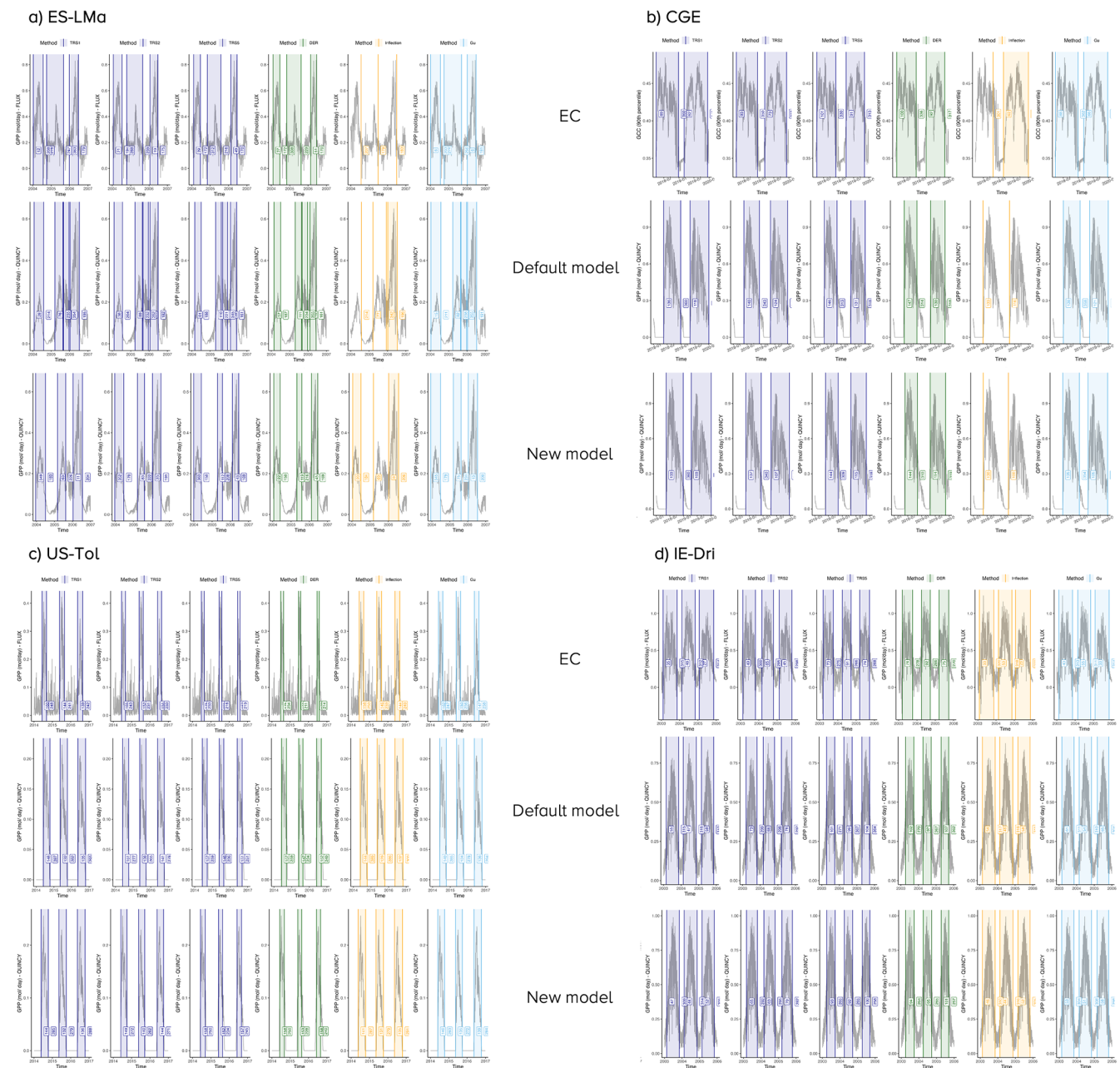
Figure B3. GPP from EC data, default and dynamic model at the four main sites with comparison of different methods of the “phenofit” package (Kong et al., 2022): threshold 10 % (TRS1), 20 % (TRS2), 50 % (TRS5), derivative (the method used in our study), Inflection and Gu. The vertical solid lines show the start and end of the season (day of the year) with the growing seasons between them as indicated by the shaded areas.
