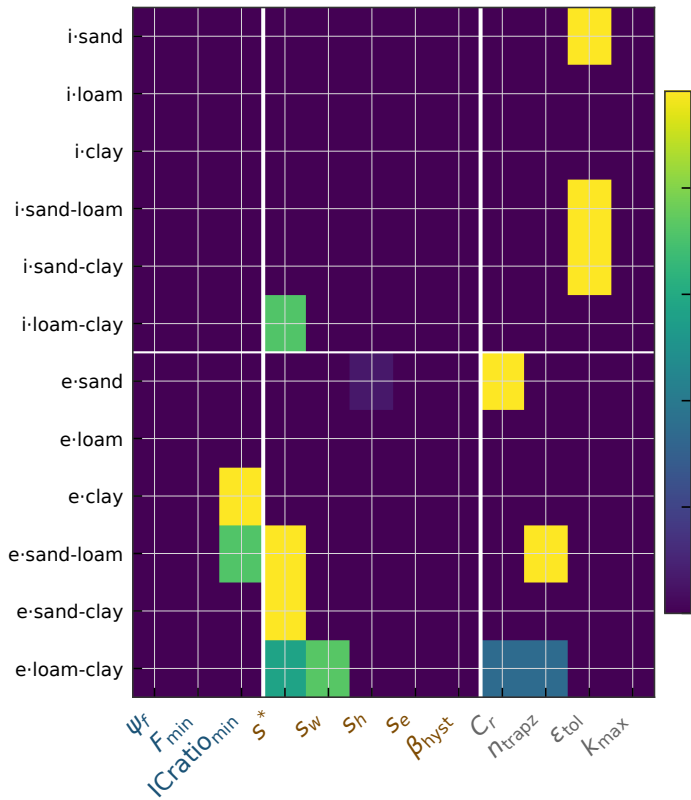
basic: per-parameter RMSE improvement [%]
