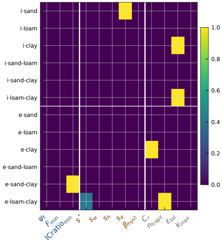
intensive: per-parameter RMSE improvement [%]
