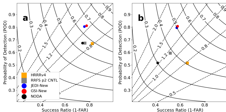
Figure 11. Performance diagrams of hourly accumulated precipitation for (a) 1.016 mm and (b) 6.35 mm thresholds over the 6 h forecast period. HRRRv4 (orange square), RRFS p2 CNTL (gray square), JEDI-New (blue circle), GSI-New (red circle), and NODA (black circle) are verified against Stage-IV observation. Black dashed lines and solid contours denote bias and CSI, respectively.
