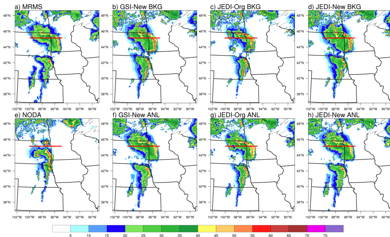
Figure 5. The composite reflectivity at final analysis time (00:00 UTC on 13 May 2022) from (a) MRMS observations, (b) GSI-New background, (c) JEDI-Org background, (d) JEDI-New background, (e) NODA forecast, (f) GSI-New analysis, (g) JEDI-Org analysis, and (h) JEDI-New analysis. The red line in each panel indicates the location of the vertical cross sections shown in Figs. 6 and 7. Because no data assimilation is performed in NODA, no analysis field is available for that experiment.
