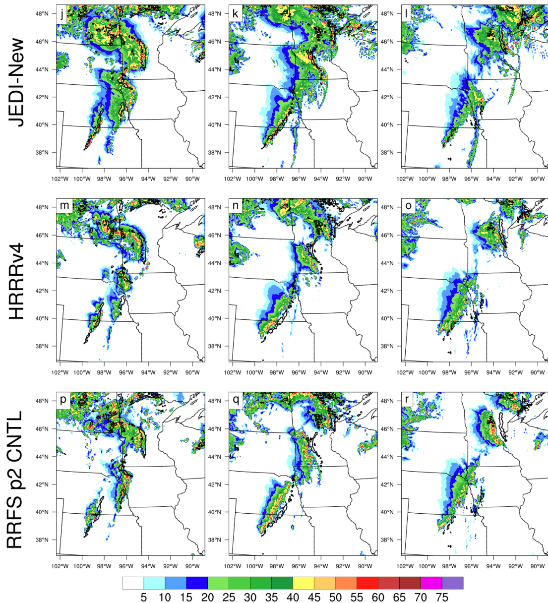
Figure 8. Composite reflectivity forecasts and observations at 1, 3, and 5 h lead times, valid at 01:00, 03:00, and 05:00 UTC 13 May 2022, respectively. Rows show MRMS observations, NODA, GSI-New, JEDI-New, HRRRv4, and RRFS p2 CNTL, and columns show the 1, 3, and 5 h forecasts. In the forecast panels, the observed 40 dBZ composite reflectivity contour is overlaid in black.
