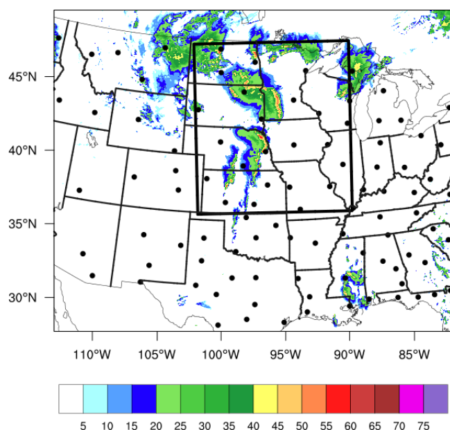
Figure 2. MRMS composite reflectivity (dBZ) at 00:00 UTC 13 May 2022 over the FV3-LAM model domain. The bold black box marks the verification domain, and WSR-88D radar locations are indicated by black dots.
