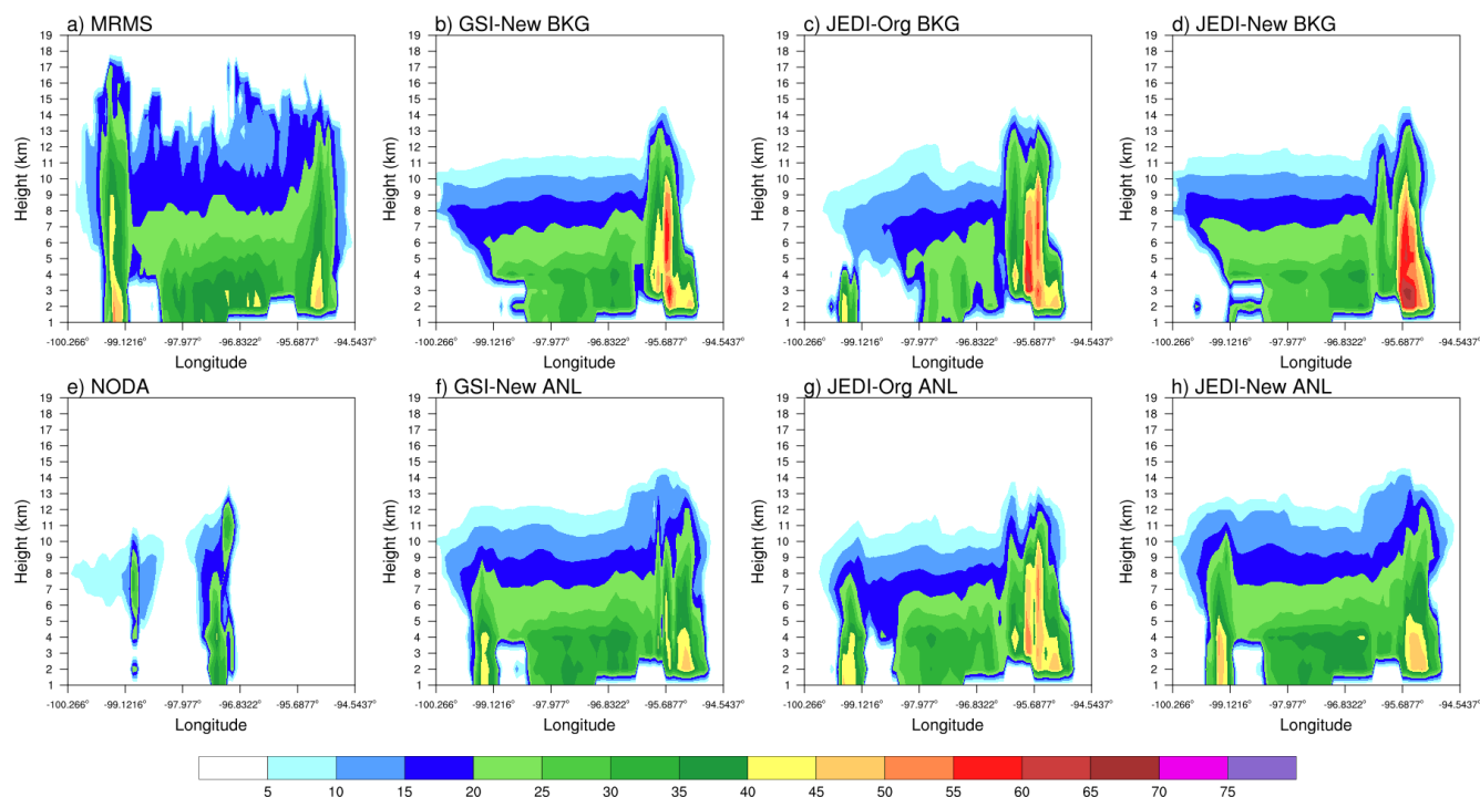
Figure 6. Vertical cross sections of composite reflectivity at the final analysis time (00:00 UTC 13 May 2022) along the red line shown in Fig. 5, from (a) MRMS observations, (b) GSI-New background, (c) JEDI-Org background, (d) JEDI-New background, (e) NODA forecast, (f) GSI-New analysis, (g) JEDI-Org analysis, and (h) JEDI-New analysis.
