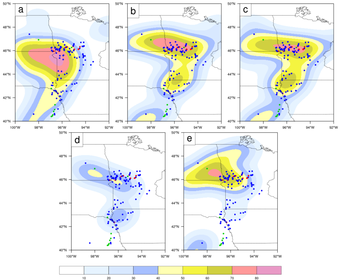
Figure 12. Neighborhood probability (%) shaded of 2 h maximum updraft helicity exceeding 75 \text{ m}^2 \text{ s}^{-2} from 00:00 to 02:00 UTC on 13 May 2022 from the forecasts of (a) NODA, (b) GSI-New, (c) JEDI-New, (d) HRRRv4 and (e) RRFS p2 CNTL. The red, green, and blue dots denote the SPC reports of tornado, hail, and wind, respectively.
