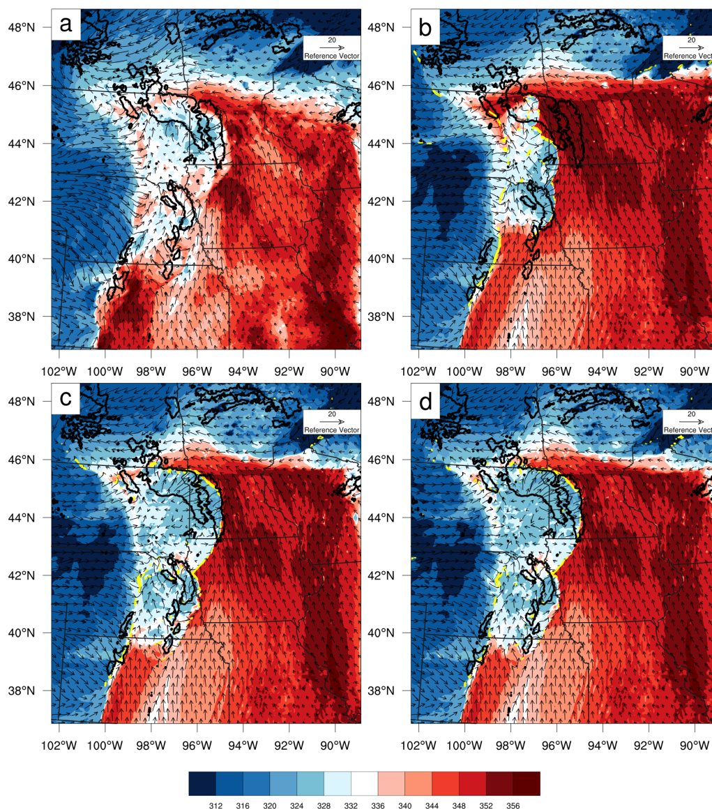
Figure 9. Equivalent Potential Temperature (shaded; K) at 2 m and wind vectors at 10 m ( \text{m s}^{-1} ) for (a) URMA, (b) NODA, (c) GSI-New, and (d) JEDI-New. Black contours denote areas where observed MRMS composite reflectivity exceeds 30 dBZ and are included in each panel as a common observational reference.
