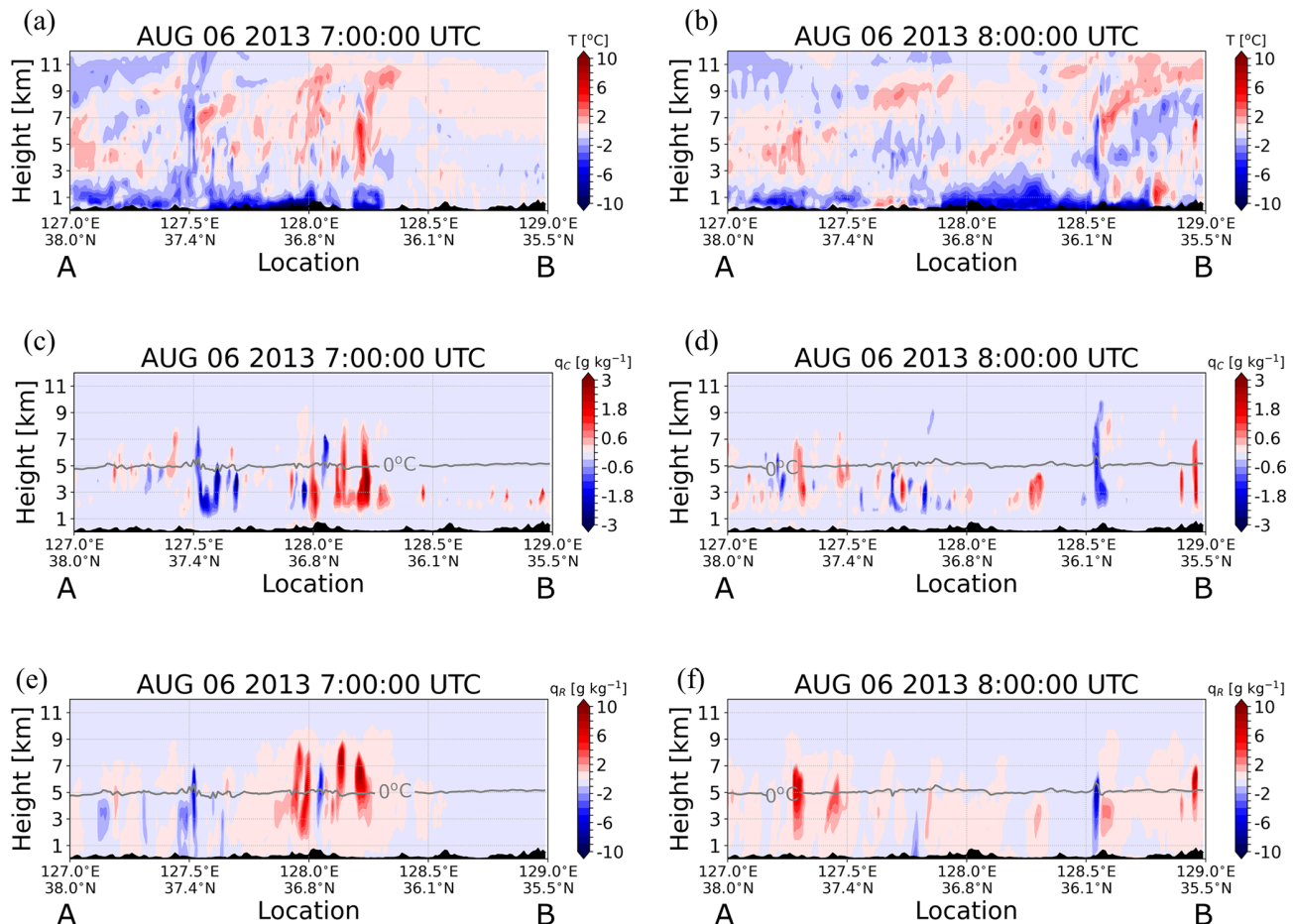
Figure 10. Differences (GDMN – WDM6) in (a) temperature ( ^{\circ}C ), (c) cloud mixing ratio ( g\ kg^{-1} ), and (e) rain mixing ratio ( g\ kg^{-1} ), shown with terrain (black color) along the cross-section indicated by the red line in Fig. 3b at 07:00 UTC, 6 August 2013. Panels (b), (d), and (f) show the same fields as (a), (c), and (e), respectively, at 08:00 UTC.
