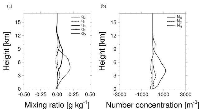
Figure 11. Differences in the time-domain averaged vertical distribution (GDMN minus WDM6) over the region denoted by the red dashed box in Fig. 3b for (a) mixing ratio ( g\ kg^{-1} ) and (b) number concentration ( m^{-3} ) between 06:00 and 08:00 UTC on 6 August 2013.
