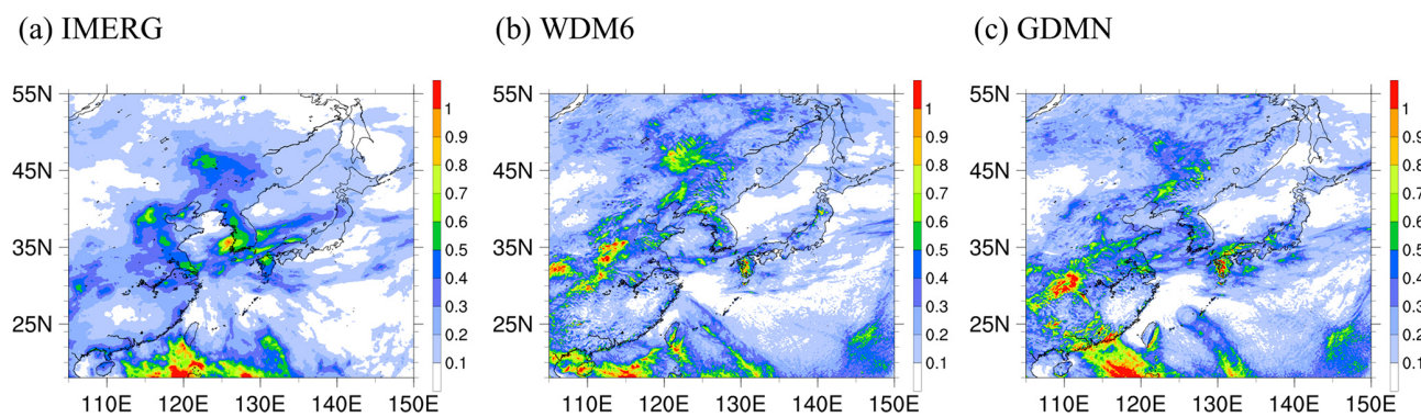
Figure 14. Spatial distribution of hourly precipitation [ \text{mm h}^{-1} ] from (a) the IMERG observations and model simulations using (b) WDM6 and (c) GDMN for the one-month simulation conducted during July 2023.
