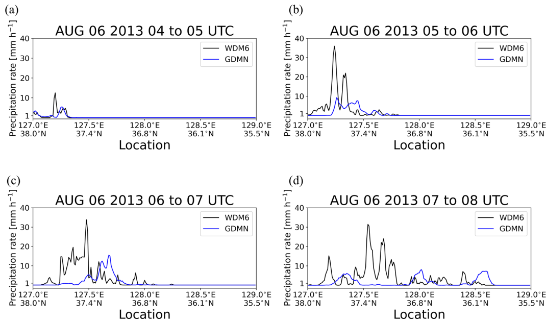
Figure 8. 1 h accumulated surface precipitation along the cross-sectional area indicated by the red solid line in Fig. 3b for (a) 04:00 to 05:00 UTC, (b) 05:00 to 06:00 UTC, (c) 06:00 to 07:00 UTC, and (d) 07:00 to 08:00 UTC on 6 August 2013. Black and blue lines represent WDM6 and GDMN, respectively.
