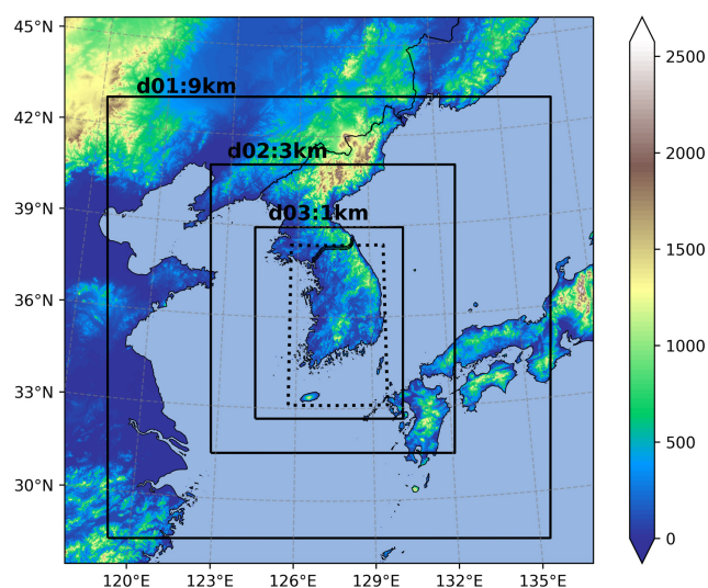
Figure 4. The model domain, consisting of three nested domains with resolutions of 9 km (d01), 3 km (d02), and 1 km (d03). Shading indicates the terrain height in meters above sea level. The analysis domain is denoted by the black dotted line within the innermost domain (d03).
