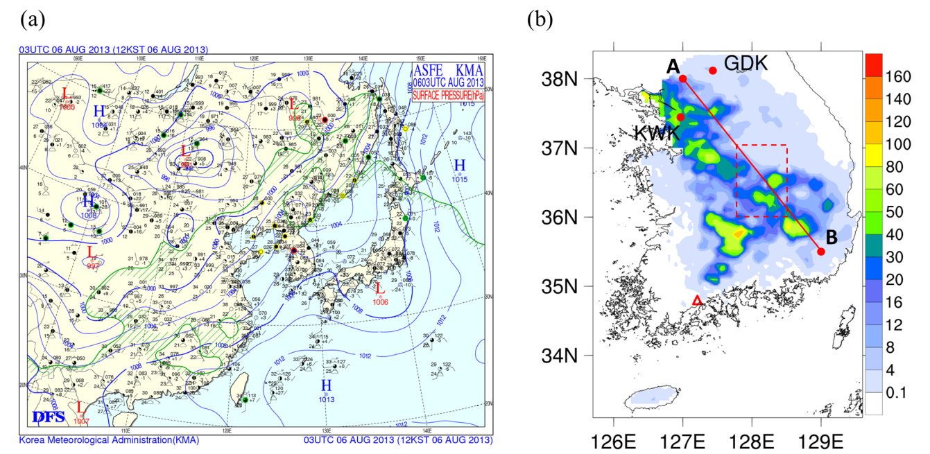
Figure 3. (a) Surface synoptic chart at 03:00 UTC on 6 August 2013, and (b) 15 h accumulated surface precipitation (mm) during the analysis period (02:00–17:00 UTC on 6 August 2013), obtained from the Korea Meteorological Administration (KMA) Automatic Weather Station (AWS) network. The red dots in (b) indicate the locations of the Kwanaksan (KWK) and Gwangdeuksan (GDK) radar sites used to validate simulated radar reflectivity. The red solid line from A to B denotes the transect for cross-sectional analysis, while the red dashed box indicates the area used for microphysical process analysis. The red triangle marks the Boseong standard weather observatory, where a two-dimensional video disdrometer (2DVD) was installed to observe rain drop size distributions (DSDs).
