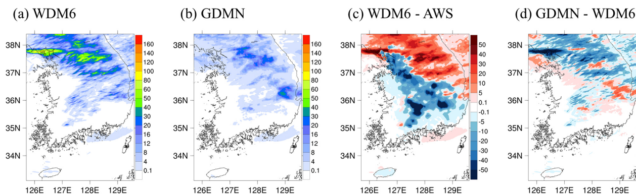
Figure 6. Accumulated surface precipitation (mm) during the analysis period (from 02:00 to 17:00 UTC on 6 August 2013) for (a) WDM6, (b) GDMN, and (c) the difference between WDM6 and Automatic Weather Station (AWS) observations (WDM6 minus AWS). (d) Same as (c), but for the difference between GDMN and WDM6 (GDMN minus WDM6).
