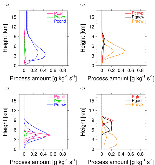
Figure 12. The vertical profiles of the time-domain averaged (a) sources and (b) sinks of the cloud mixing ratios ( \text{g kg}^{-1} \text{s}^{-1} ) over the region indicated by the red dashed box in Fig. 3b between 06:00 and 08:00 UTC on 6 August 2013. Only the major microphysical processes are represented. The solid and dashed lines represent GDMN and WDM6, respectively. Panels (c) and (d) show the same as (a) and (b) but for the rain mixing ratio ( \text{g kg}^{-1} \text{s}^{-1} ).
