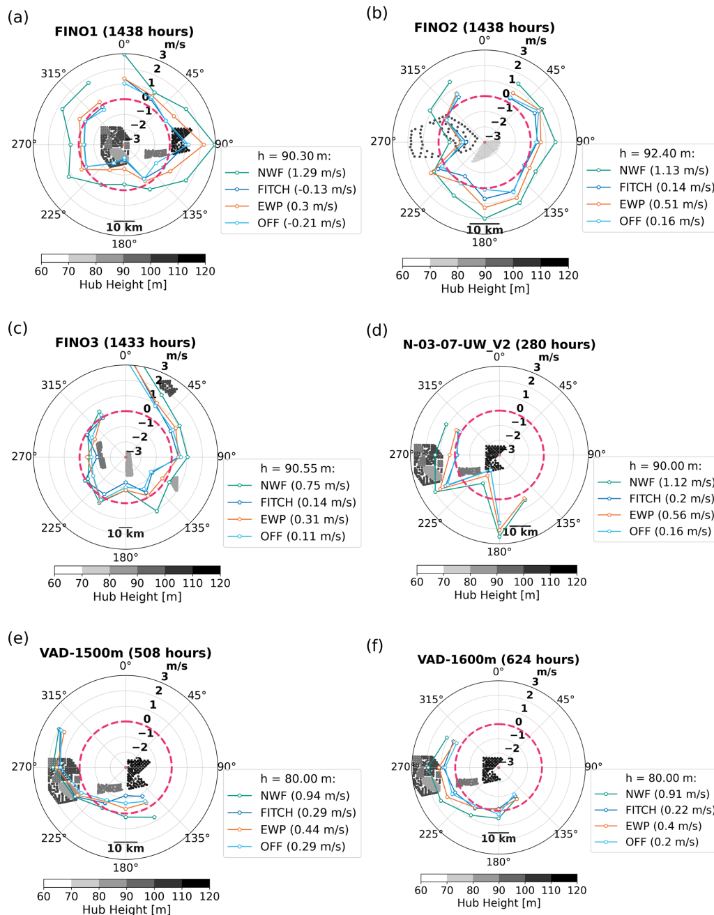
Figure 13. Directional bias (simulation minus measurements) of the different simulation scenarios (colored lines) for measurement sites close to wind farms. Bold dashed magenta circle highlights zero bias. Lines within the magenta circle indicate negative biases, while lines outside indicate positive biases. The averaged bias over all directions is shown in the legend. Dots show the location and hub height of wind turbines in the vicinity of each site, which is shown as a red dot in the center of the plot. The total duration of observational data for each site is shown in the subtitle. Sectors with fewer than 10 occurrences in either the observations or the simulations are not shown.
