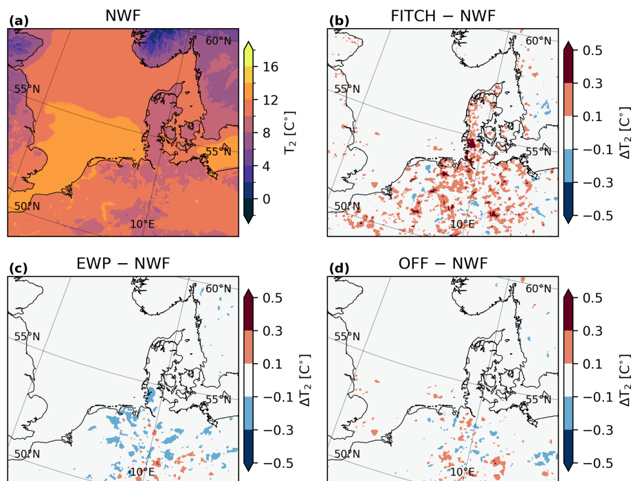
Figure 19. As Fig. 18, but averaged during nighttime (00:00–04:00 UTC) conditions only.
