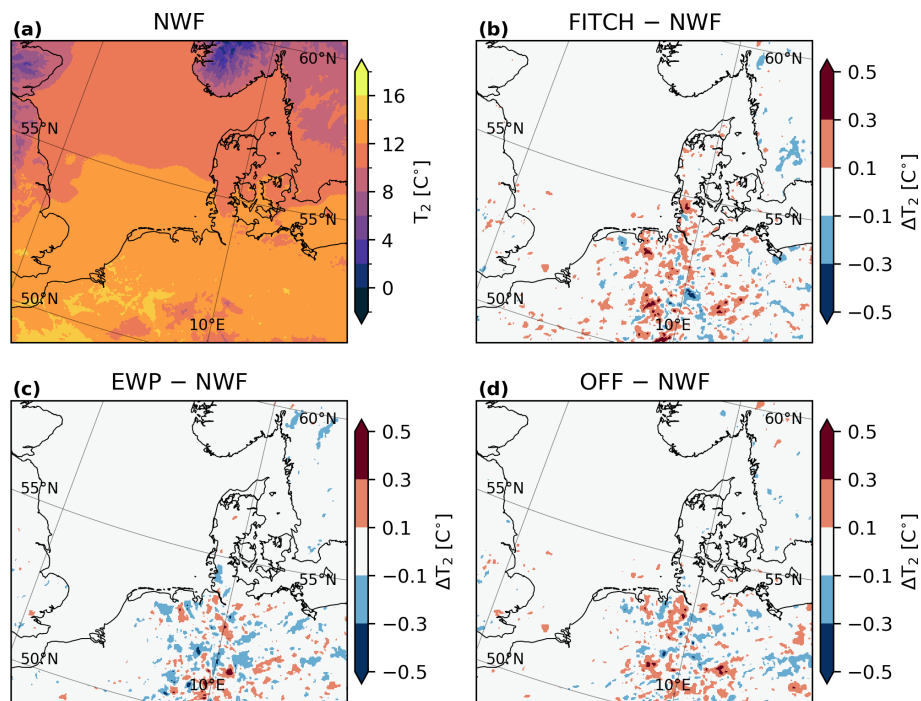
Figure 18. (a) Average 2 m temperature for February 2020 and August 2022 for the simulation without wind farms (NWF) and difference to simulations with (b) FITCH WFP, (c) EWP WFP and (d) FITCH WFP for offshore turbines only zoomed into the North Sea and Danish Baltic.
