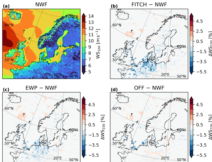
Figure 14. (a) Average wind speed at a height of 100 m for February 2020 and August 2022 for the simulation without wind farms (NWF) and normalized difference with respect to NWF to simulations with (b) FITCH WFP, (c) EWP WFP and (d) FITCH WFP for offshore turbines only.
