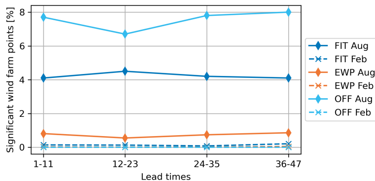
Figure 16. Relative number of significant grid points with respect to the number of grid points with wind turbines for different lead times for different scenarios (colors) and the 2 months (solid lines are August 2022 and dashed lines are February 2020).
