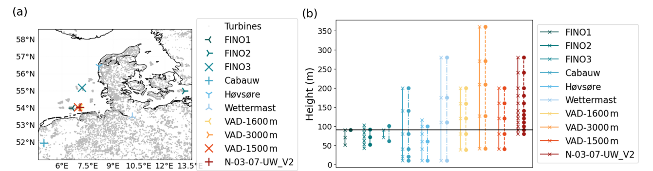
Figure 10. (a) Locations of the observations (blueish colors for masts, reddish colors for lidars) used for validation. (b) Measurement heights for wind speed (solid lines with crosses) and wind direction (dashed lines with dots) following filtering of heights with too low data availability (see text). Horizontal black line indicates height of the wind-rose bias plots in Fig. 13.
