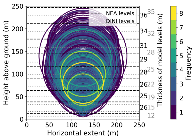
Figure 9. Height of the lowest HARMONIE model levels and turbine rotors included in the domain for the NEA simulations, color-coded by occurrence frequency in the WTD. Dashed lines show levels of the NEA domain used for our month-long simulations; dotted lines show levels of the DINI domain used in the vertical sensitivity study (Sect. 5.4). The numbers on the right indicate the thickness of each model level for NEA (black) and DINI (gray).
