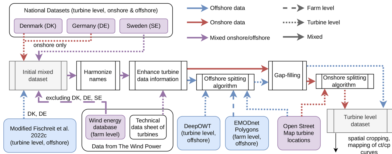
Figure 2. Illustration of the workflow behind the wind farm database connecting the different input sources in Table 1 to the final merged, gap-filled, turbine-level wind farm dataset.
