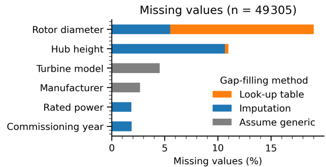
Figure 3. Proportion of missing values in the full European wind turbine database.
