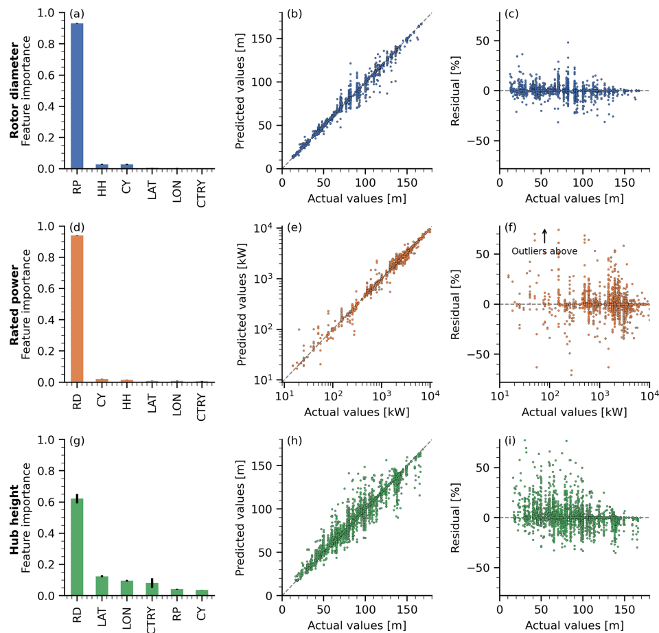
Figure 6. Feature importance and model evaluation for gap-filling models of rotor diameter, rated power, and hub height. (a, d, and g): Feature importance of explanatory variables – rotor diameter (RD), hub height (HH), rated power (RP), commissioning year (CY), country (CTRY), latitude, and longitude (LAT and LON). Bars represent the mean and standard deviation of feature importance estimated by MDI across 100 random forest estimators. (b, e, and h): Scatter plots of actual versus predicted values. (c, f, and i): Model residuals (errors) in percent relative to actual values.
