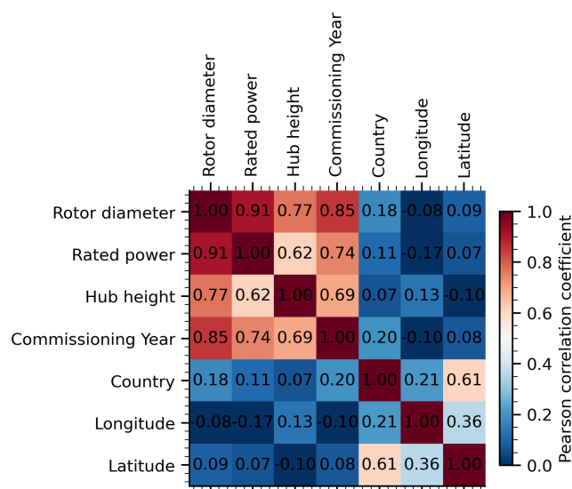
Figure 4. Correlation matrix between the various variables used for the gap-filling models.
