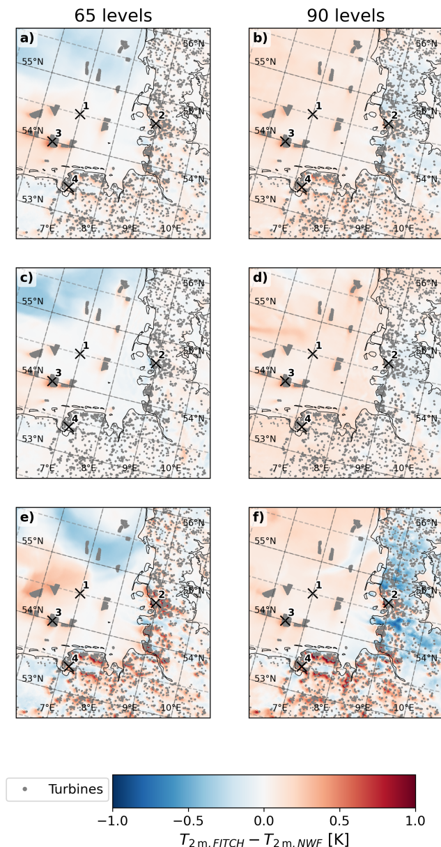
Figure 20. 2 m temperature difference for FITCH-NWF for (a, c, and e) 65 levels and (b, d, and f) 90 levels averaged (a, b) over the full week 8–17 May 2025 and (c, d) over daytime (12:00–16:00 UTC) and (e, f) over nighttime conditions (00:00–04:00 UTC) only. Turbines are shown as gray dots, and the four crosses highlight locations used in Fig. 21.
