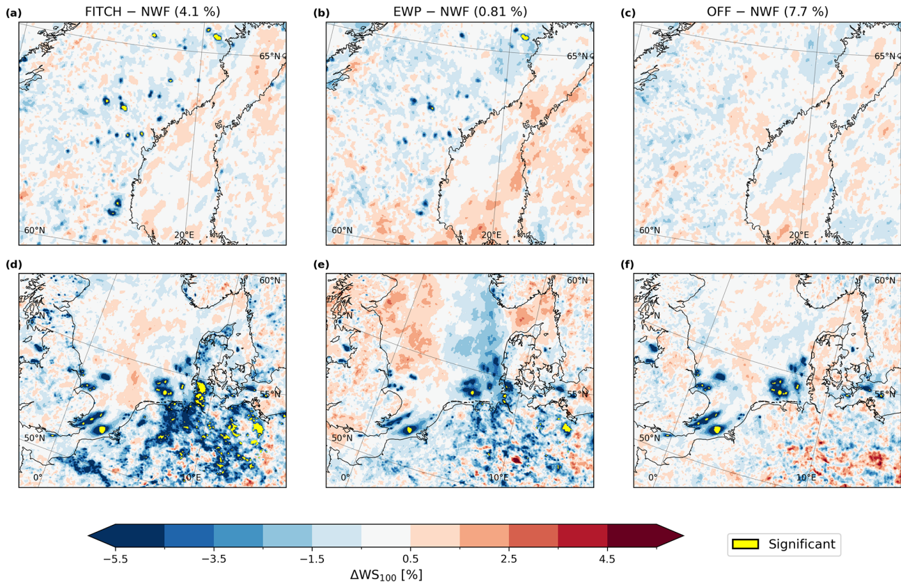
Figure 17. Statistically significant grid points (yellow) for the three scenarios with wind farm parameterizations (FITCH, EWP, OFF) compared to the NWF scenario for the lead time 1–11 h for August 2022 for (a,b,c) focusing on Northern Sweden and (d,e,f) focusing on the North Sea region and the Danish Baltic. The percentage number shows the number of significant grid points relative to the number of grid points with wind turbines for the entire domain. Colors in the background show normalized differences with respect to NWF for the different wind farm parameterizations.
