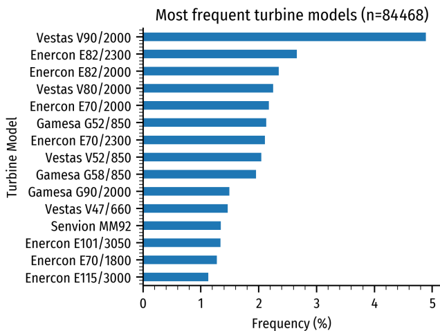
Figure 7. Frequency of turbines in the dataset after gap-filling and splitting all wind farms into individual turbine entries.
