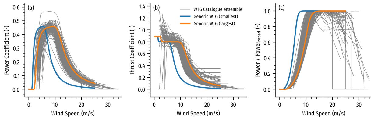
Figure 8. Turbine operational curves: (a) power coefficient curves, (b) thrust coefficient curves, and (c) power curve relative to the rated power. The grey lines show all curves for all different turbine models. The blue and orange lines show the generic curves using PyWake’s standard_power_ct_curve function (PyWake-Team, 2022), respectively, for the smallest and largest turbines in the turbine dataset.
