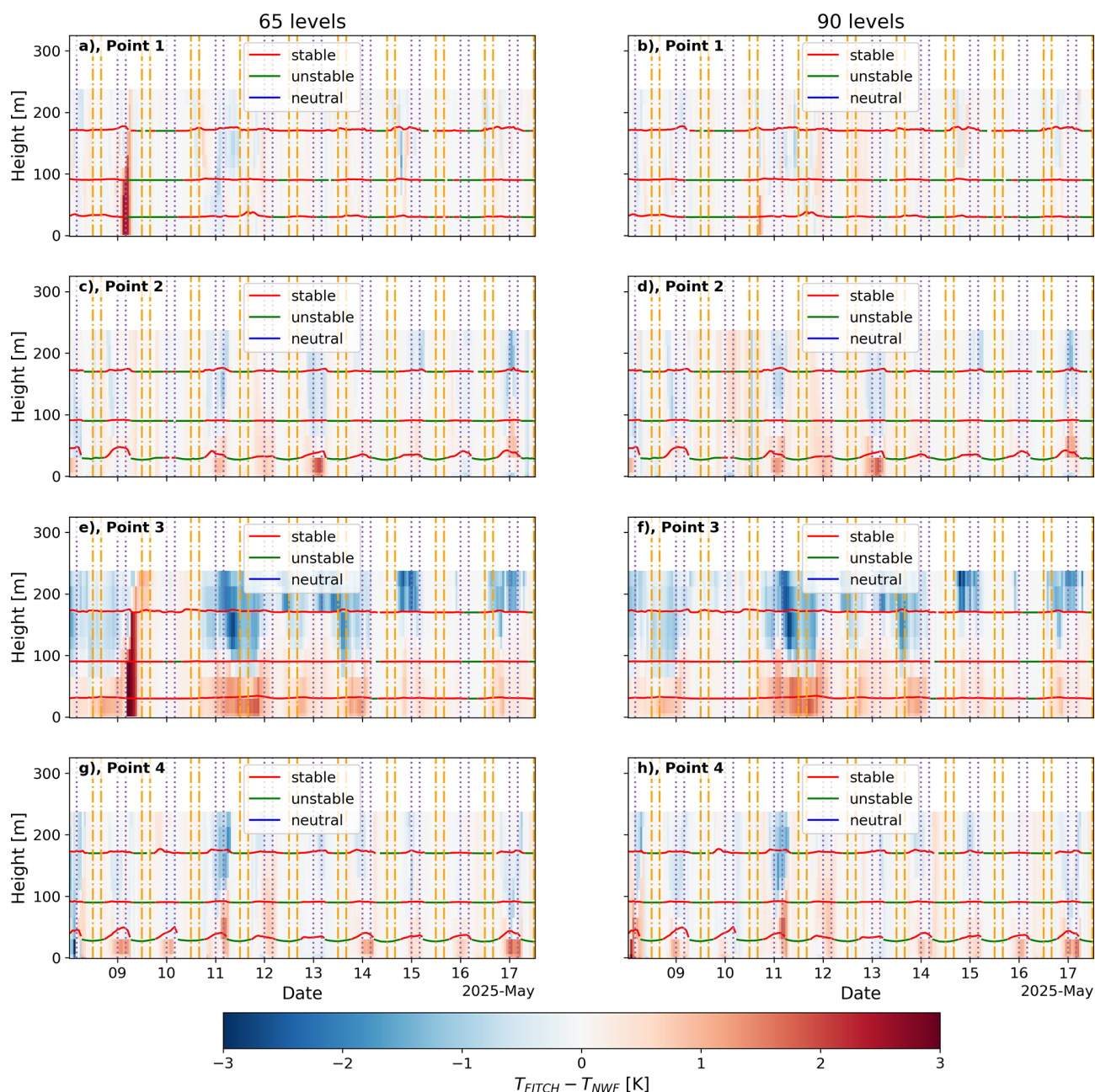
Figure 21. Timeseries of temperature profile difference of FITCH minus NWF for four points (rows) highlighted in Fig. 20 for the (a, c, e, and g) 65 levels and (b, d, f, and h) 90 levels. The background color shows the temperature difference at each altitude and date. The horizontal lines highlight the color-coded virtual potential temperature gradient ( \gamma )-derived stability for three heights (10–50, 80–100 and 140–200 m) and shown at the center of these layers. Purple dotted vertical lines highlight periods used for nighttime averages (00:00–04:00 UTC) and orange dash-dotted vertical lines highlight daytime average periods (12:00–16:00 UTC).
