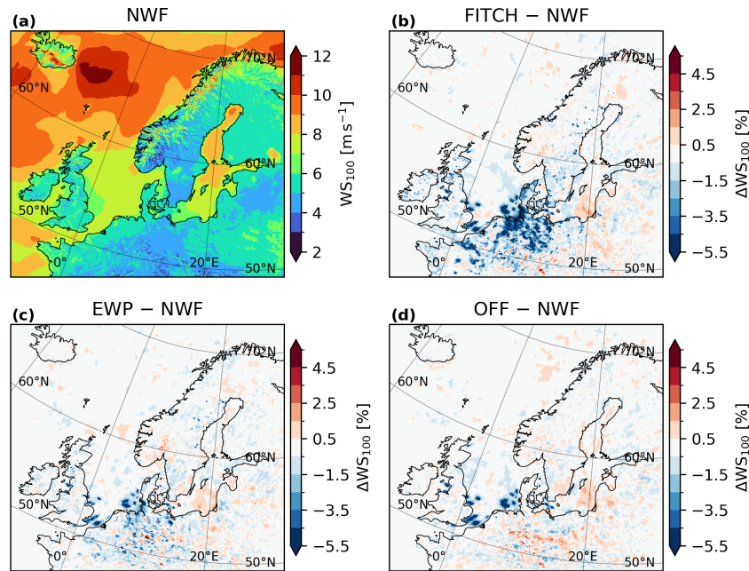
Figure A7. Same as Fig. 14, but only for August 2022.
