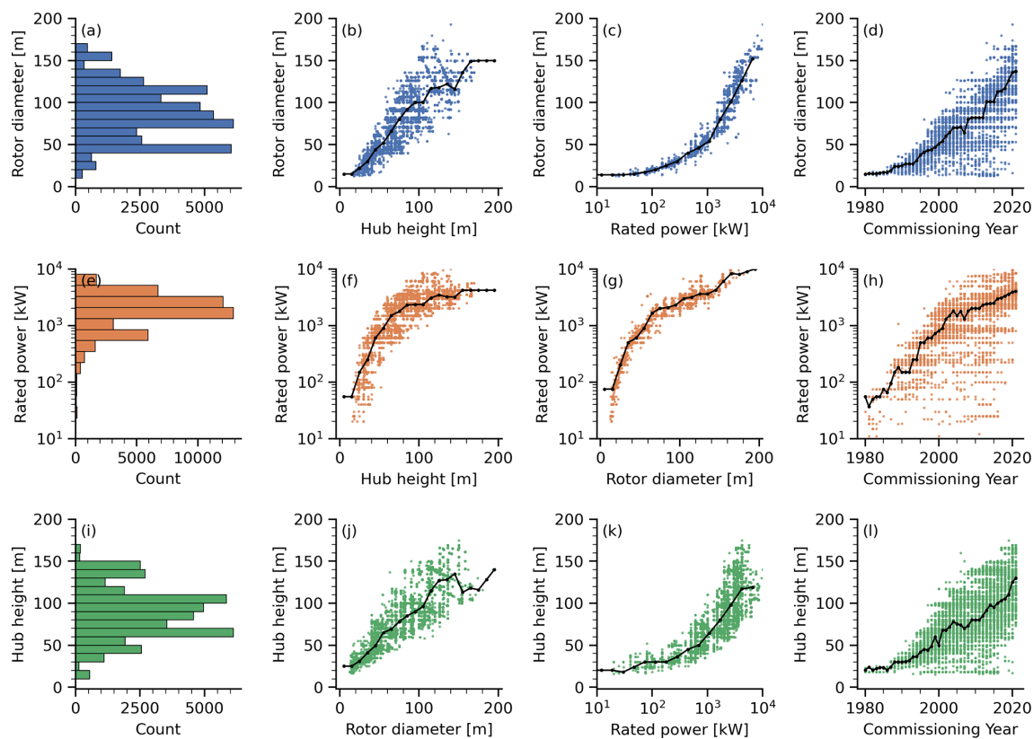
Figure 5. Rotor diameter, rated power and hub height distributions and relationships in the turbine dataset. Top, middle, and bottom rows represent each variable. First column (plots a, e, and i) displays histograms; Middle plots (b, c, f, g, j, and k) illustrate co-variation between variables: rotor diameter with hub height and rated power; rated power with hub height and rotor diameter; and hub height with rotor diameter and rated power. Last column (plots d, h, and l) show variation over commissioning year. Black lines indicate median values within variable bins.
