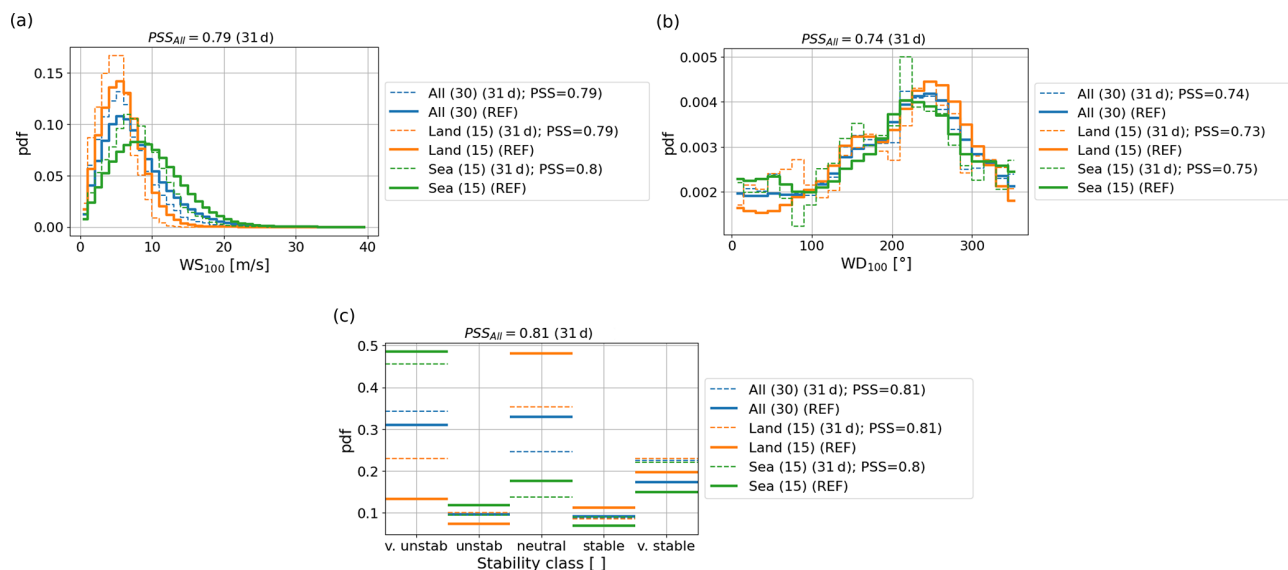
Figure A5. As Fig. A3, but only for August 2022 (31 d).
