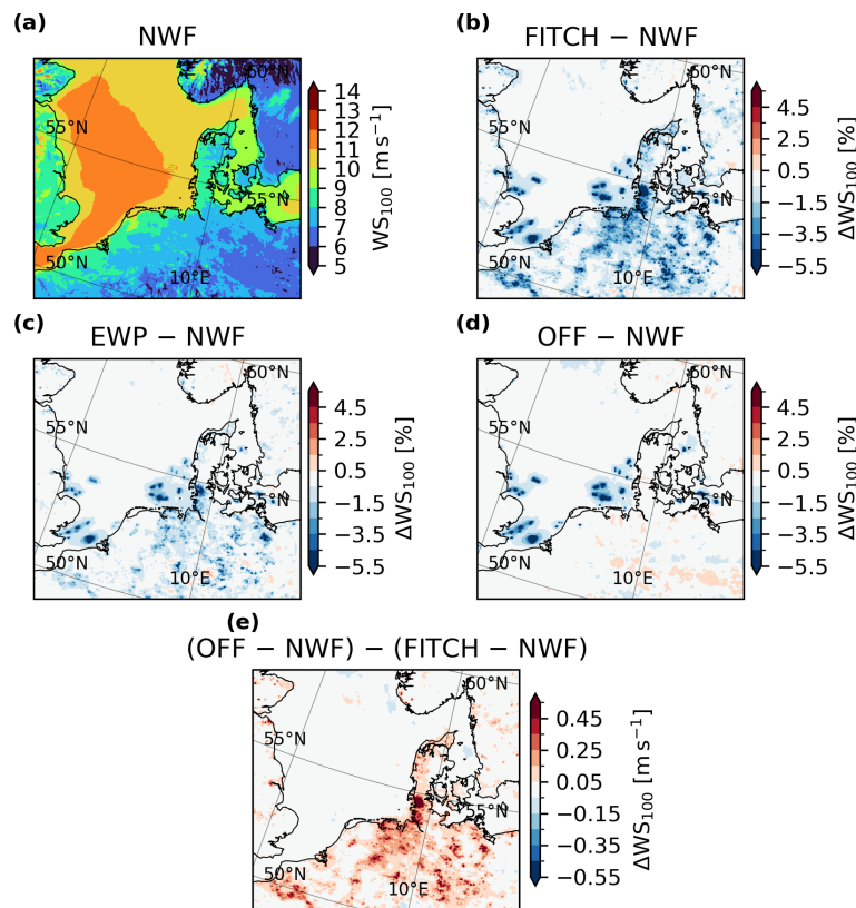
Figure 15. (a) Average wind speed at a height of 100 m for February 2020 and August 2022 for the simulation without wind farms (NWF) and normalized difference with respect to NWF to simulations with (b) FITCH WFP, (c) EWP WFP, (d) FITCH WFP for offshore turbines only and (e) the absolute difference between (d) and (b); zoom into the North Sea and Danish Baltic.
