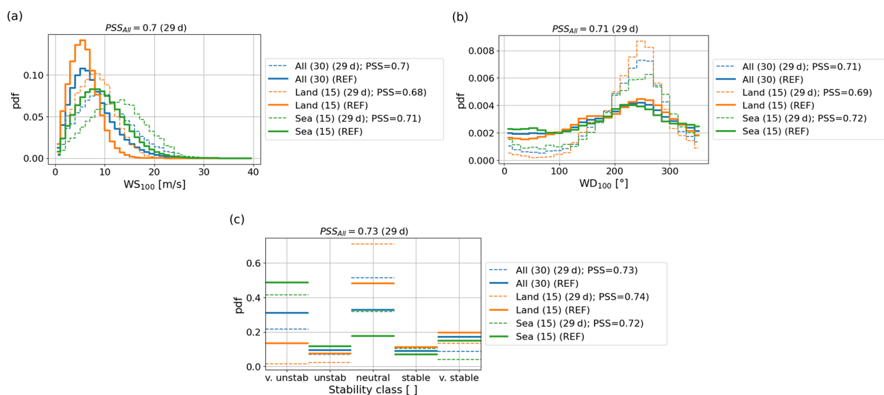
Figure A4. As Fig. A3, but only for February 2020 (29 d).
