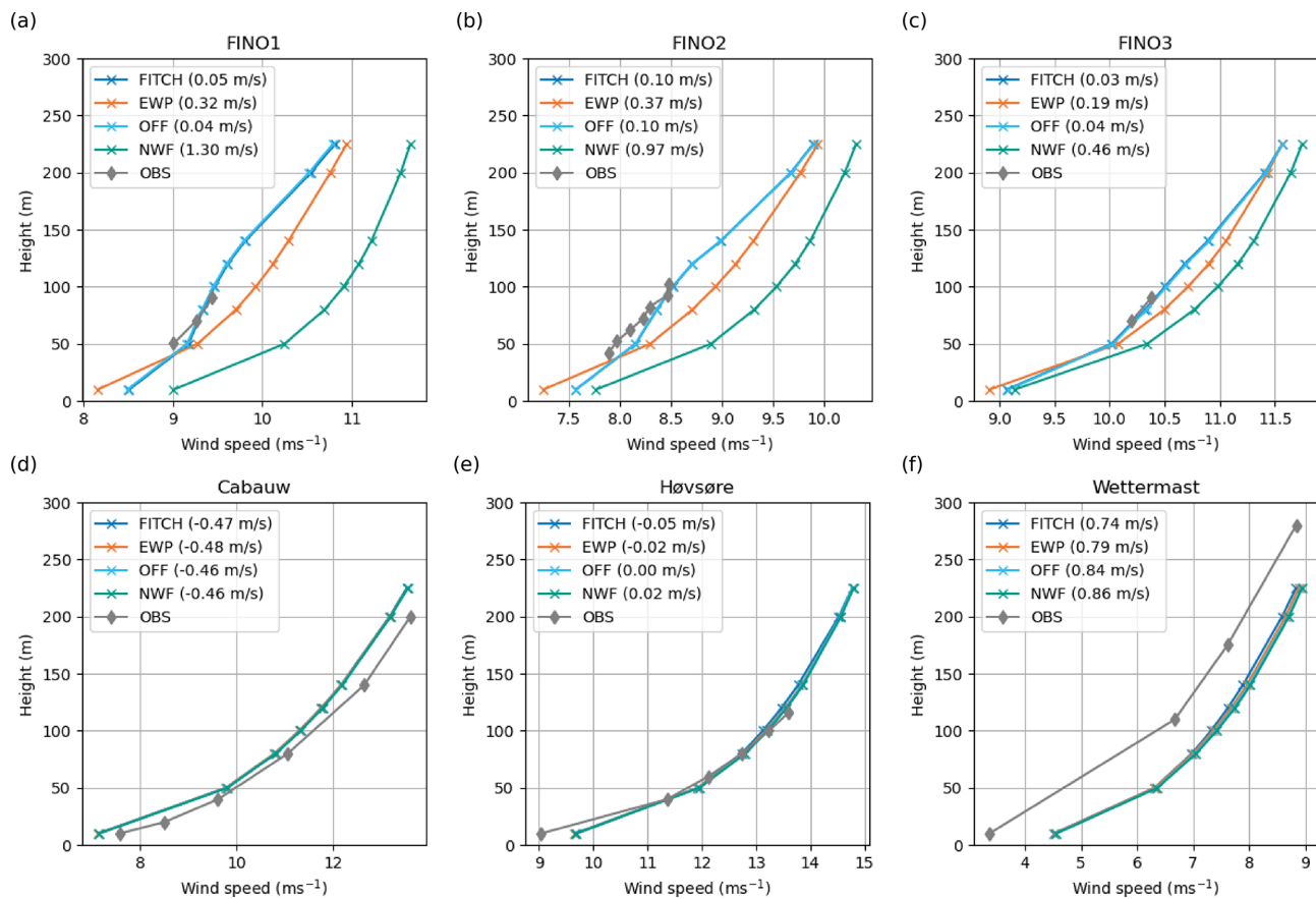
Figure 11. Time-averaged profiles from the forecasts and from mast measurements for both months. Mean biases over all heights are shown for the different scenarios. Note that the x axis varies from site to site and FITCH and OFF are almost identical.
