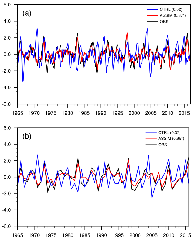
Figure 5. Time series of the (a) monthly and (b) winter Niño 3.4 indices from 1965 to 2016 for the observation (black line), ASSIM (red line), and CTRL (blue line). The correlation coefficients with the observation for ASSIM and CTRL are also shown in parentheses. The asterisk indicates that the correlation is statistically significant at the 95 % confidence level.
