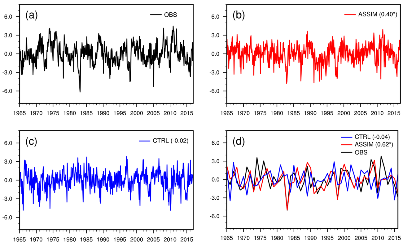
Figure 7. Time series of the (a–c) monthly and (d) winter Southern Oscillation Index (SOI) from 1965 to 2016 for the observation (black line), ASSIM (red line), and CTRL (blue line). Panels (a)–(c) show individual monthly time series from observation, ASSIM, and CTRL, respectively, while panel (d) shows the winter SOI averaged over December–February (DJF). The correlation coefficients with the observation in ASSIM and CTRL are also indicated in parentheses. The asterisk indicates that the correlation is statistically significant at the 95 % confidence level.
