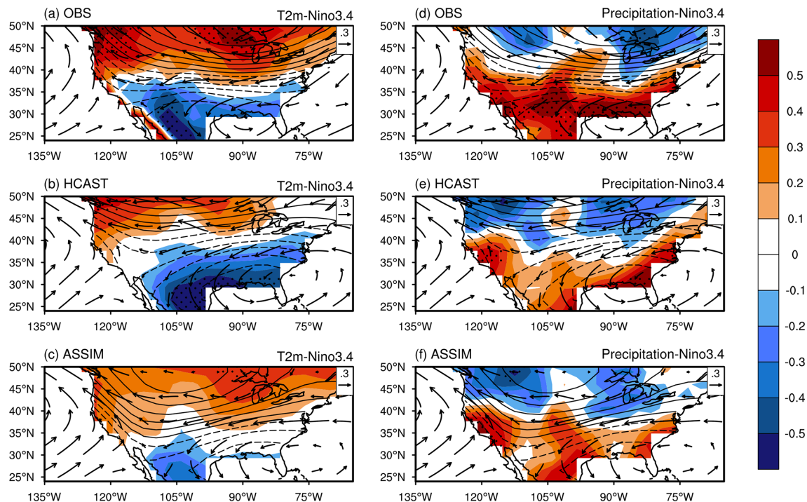
Figure A5. Regression patterns of winter surface air temperature (left column; shaded) and precipitation (right column; shaded), 500 hPa geopotential height (contours), and 850 hPa winds (vectors) on the standardized winter Niño 3.4 index from 1981 to 2010 for (a, d) the observation, (b, e) HCAST, and (c, f) ASSIM. The HCAST results are based on the ensemble mean hindcasts initialized at five-year intervals from 1981 to 2006, as described in Fig. A4. The successive five-year segments are then concatenated to form a continuous time series from 1981 to 2010, without any bias correction applied. Dotted areas indicate regions where the regressions are statistically significant at the 95 % confidence level.
