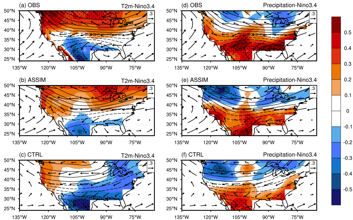
Figure 14. Regression patterns of winter surface air temperature (left column; shaded) and precipitation (right column; shaded), 500 hPa geopotential height (contours), and 850 hPa winds (vectors) on the standardized winter Niño 3.4 index from 1980 to 2016 for (a, d) the observation, (b, e) ASSIM, and (c, f) CTRL. In each panel, the Niño 3.4 index is calculated separately using each corresponding dataset and all regressions are based on simultaneous winter (DJF) averages. Dotted areas indicate regions where the regressions are statistically significant at the 95 % confidence level.
