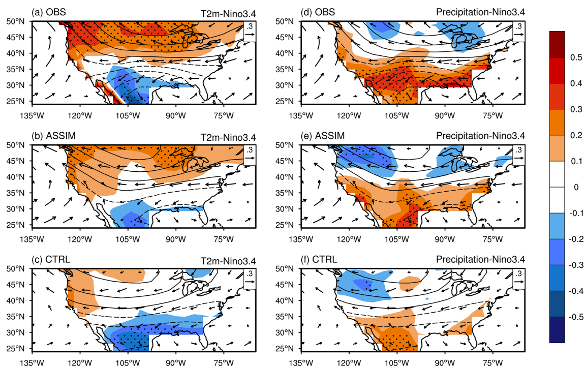
Figure A3. Lagged regression patterns of monthly winter (DJF) surface air temperature (left column; shaded), precipitation (right column; shaded), 500 hPa geopotential height (contours), and 850 hPa winds (vectors) onto the corresponding one-month-earlier standardized Niño 3.4 index (NDJ) for (a, d) the observation, (b, e) ASSIM, and (c, f) CTRL. Specifically, monthly atmospheric variables from December to February (DJF) are regressed onto the standardized monthly Niño 3.4 index from November to January (NDJ), corresponding to a one-month lead time. The Niño 3.4 index is calculated separately from each corresponding dataset. Dotted areas denote statistical significance at the 95 % confidence level.
