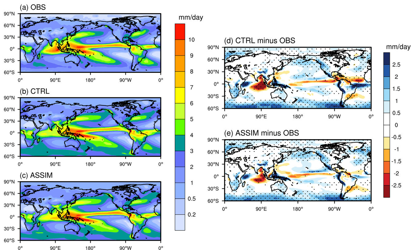
Figure 4. Spatial patterns of (a–c) climatological mean precipitation (units: \text{mm d}^{-1} ) and (d, e) precipitation differences for the period 1980–2016. Panels (a)–(c) show precipitation climatology from observation, CTRL, and ASSIM, respectively. Panels (d) and (e) represent precipitation differences between model simulations and observations: (d) CTRL minus observation and (e) ASSIM minus observation. Dotted areas indicate regions where the differences are statistically significant at the 95 % confidence level.
