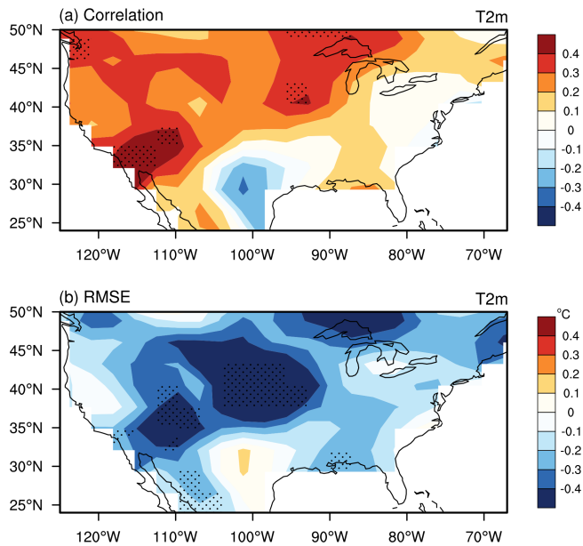
Figure 12. Spatial patterns of the differences between ASSIM and CTRL in (a) correlation coefficients and (b) root-mean-square errors (RMSE; °C) of detrended winter surface air temperature anomalies relative to observations from 1980 to 2016 over the contiguous US. Dotted areas indicate regions where the differences are statistically significant at the 95 % confidence level.
