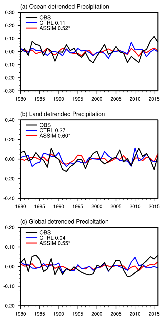
Figure 3. Time series of linearly detrended annual mean precipitation anomalies (units: \text{mm d}^{-1} ) over (a) ocean, (b) land, and (c) global domains from 1980 to 2016. Black line: observation; blue line: CTRL; red line: ASSIM. Precipitation anomalies are computed by removing both the climatological mean and long-term trend. For the detrended series, a linear trend is removed from the domain-averaged time series. The correlation coefficients of CTRL and ASSIM with the observation are also shown. The asterisk denotes a statistically significant correlation at the 95 % confidence level.
