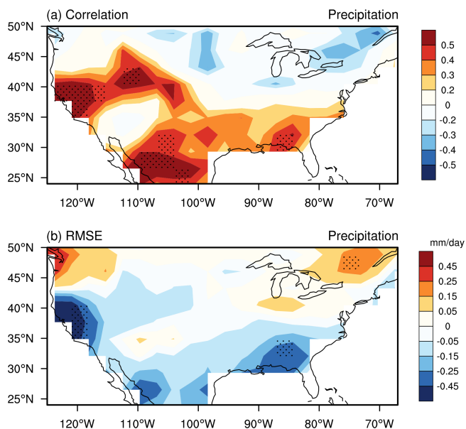
Figure 13. Similar to Fig. 12 but for detrended winter precipitation. Dotted areas denote regions where the differences are statistically significant at the 95 % confidence level.
