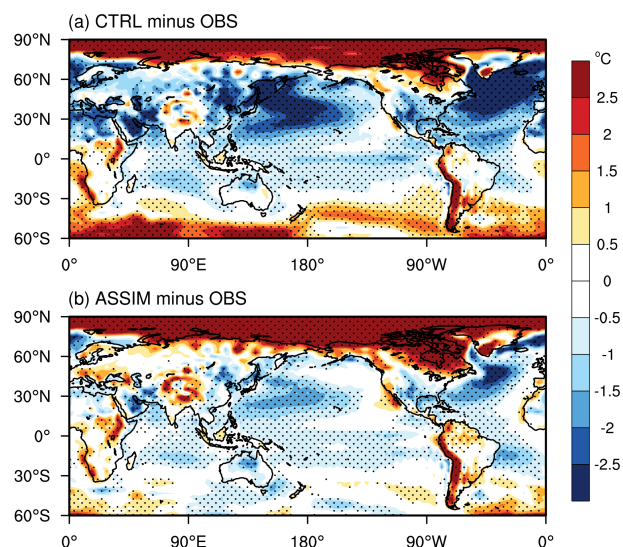
Figure 2. Spatial patterns of climatological mean differences in surface air temperature (units: ^{\circ}\text{C} ) between model simulations and observations for the period 1965–2016. Panel (a) shows the difference between CTRL and observation, and panel (b) shows the difference between ASSIM and observation. Dotted areas denote regions where the differences are statistically significant at the 95 % confidence level.
