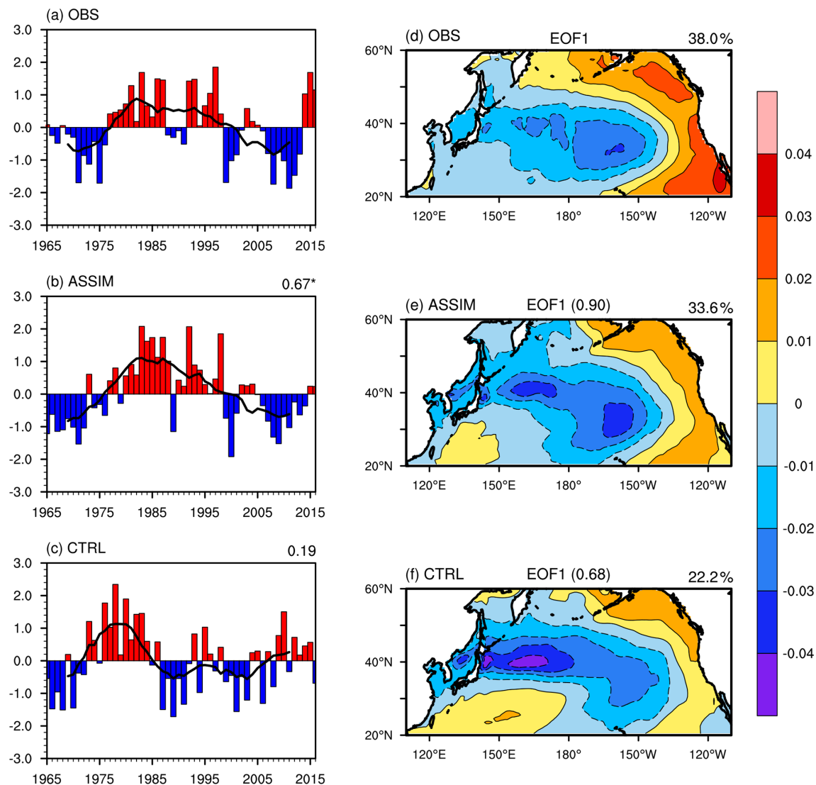
Figure 9. Time series and spatial patterns of the Pacific Decadal Oscillation (PDO) index from 1965 to 2016 for (a, d) the observation, (b, e) ASSIM, and (c, f) CTRL. The black lines in panels (a)–(c) denote the 10-year running mean of the annual PDO index. The numbers at the top right of (b) and (c) indicate the temporal correlations of ASSIM and CTRL with observations. The asterisk indicates that the temporal correlation is statistically significant at the 95 % confidence level. The percentage of variance explained by EOF1 is shown at the top right of (d)–(f), and the numbers at the top center of (e) and (f) indicate the spatial correlations with the observed pattern. The EOF analysis is performed separately for the observations and model outputs after interpolating both onto a common horizontal grid and removing linear trends at each grid point.
