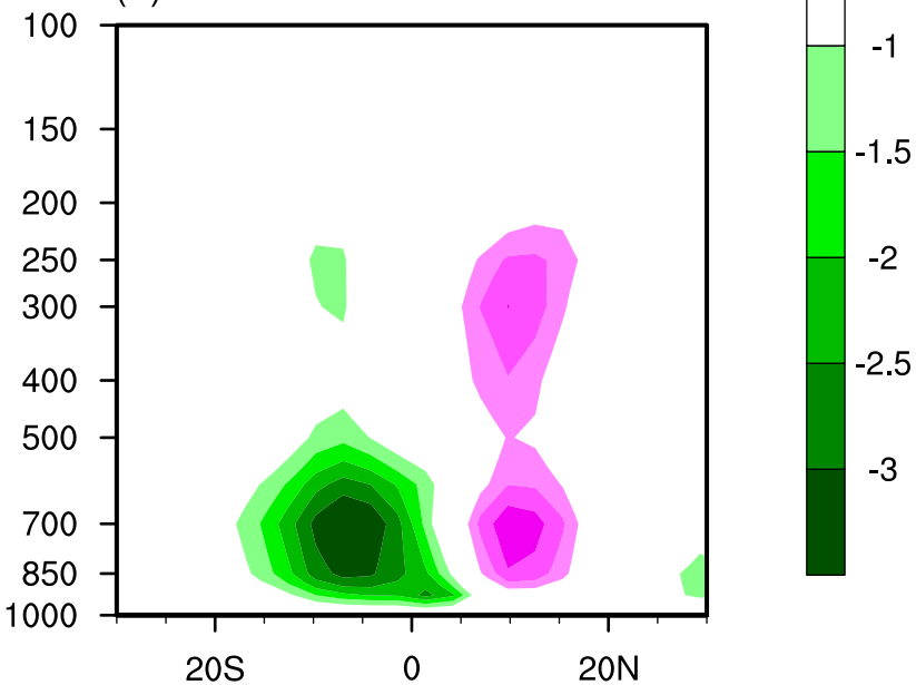
(b) ASSIM minus OBS
