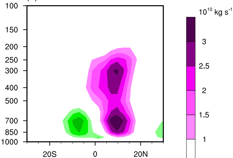
(a) CTRL minus OBS
