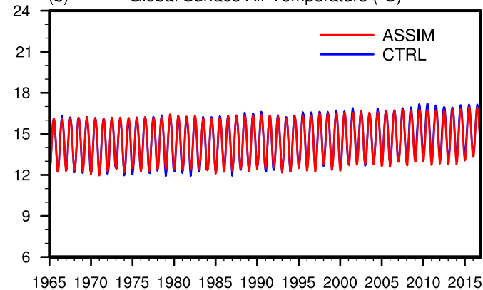
(b) Global Surface Air Temperature ( ^{\circ}\text{C} )
