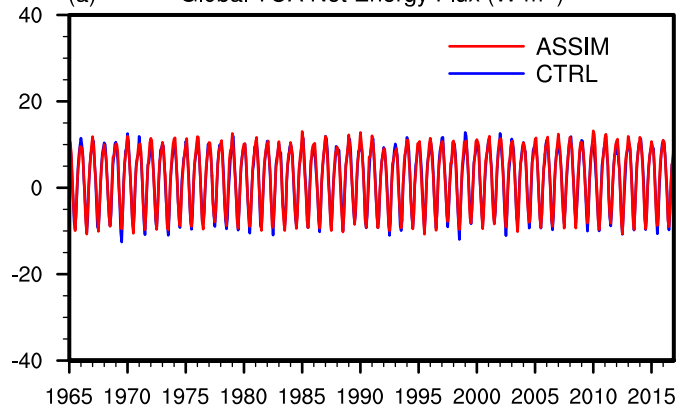
(a) Global TOA Net Energy Flux ( \text{W m}^{-2} )
