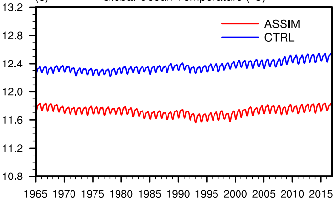
(c) Global Ocean Temperature ( ^{\circ}\text{C} )
