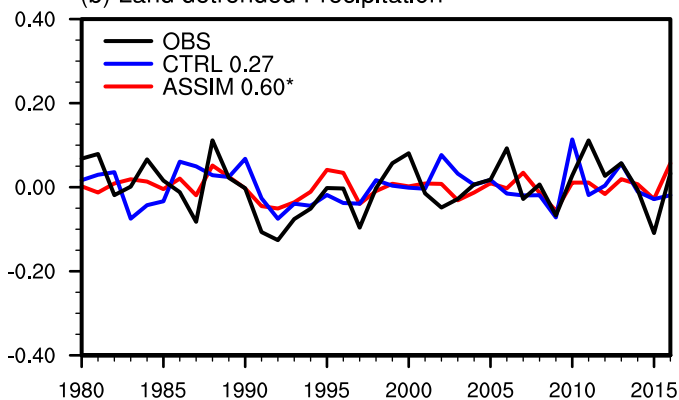
(b) Land detrended Precipitation
