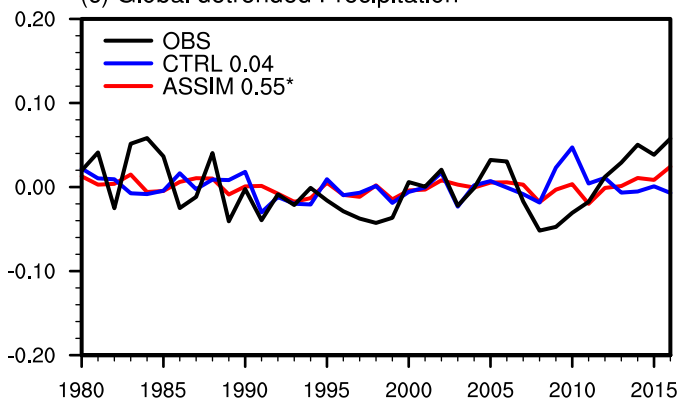
(c) Global detrended Precipitation
