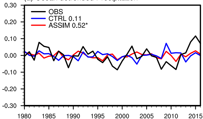
(a) Ocean detrended Precipitation
