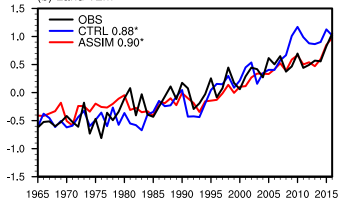
(b) Land T2m
