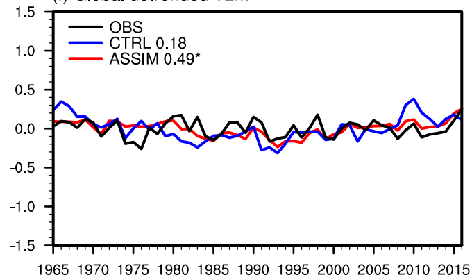
(f) Global detrended T2m
