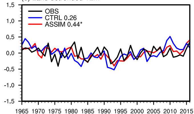
(e) Land detrended T2m
