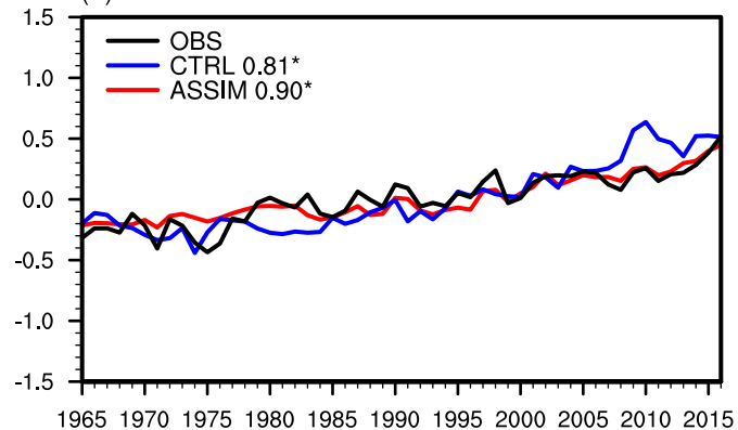
(a) Ocean T2m
