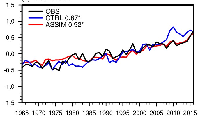
(c) Global T2m
