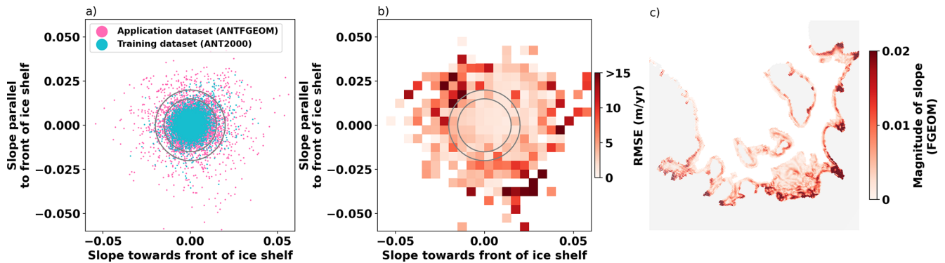
Figure 7. Average RMSE as a function of ice-shelf draft slope. (a) The distribution of data in the training dataset, ANT2000 (blue) and the ANTFGEOM simulation (pink), compared to (b) the RMSE as a function of the ice-shelf draft slope parallel ( s_{\parallel} ) and perpendicular ( s_{\perp} ) to the ice front when the neural network trained on the ANT2000 dataset is applied to the ANTFGEOM simulation. (c) The magnitude of the slope ( \sqrt{s_{\perp}^2 + s_{\parallel}^2} ) of the ice-shelf draft in the Filchner-Ronne region in the FGEOM simulation. The grey circles show where the magnitude of the slope is 0.015 (inner) and 0.02 (outer) respectively.
