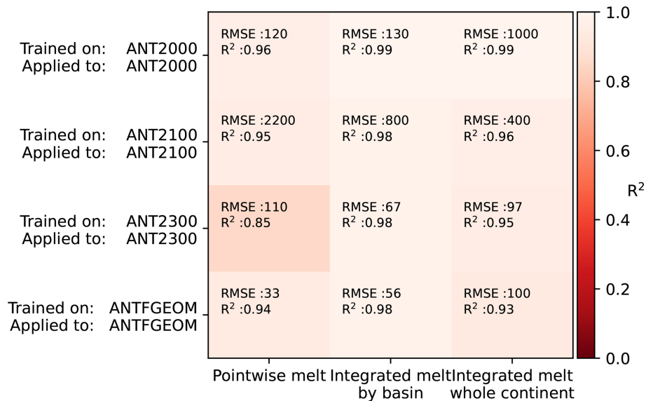
Figure A5. Metrics for the trained neural networks used in model validation. In each case, a trained neural network is applied to one of the simulations. We report the root-mean-squared error (RMSE) and correlation coefficient ( R^2 ) of the reference melt rate from the simulation compared to the melt rate predicted using the neural network, for the pointwise melt in \text{m yr}^{-1} (ice equivalent) and for the integrated melt in \text{Gt yr}^{-1} (integrated by basin and over the whole continent).
