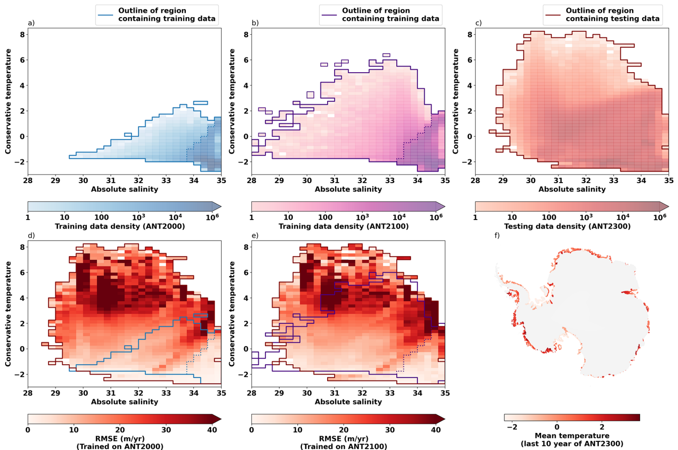
Figure 5. The highest RMSE values are observed for temperatures outside the range of the training dataset. The distribution of temperature and salinity for (a) the ANT2000 simulation, (b) the ANT2100 simulation and (c) the ANT2300 simulation. For ease of comparison, an outer contour is marked (solid line), and an inner contour bounding the region of highest data density (dotted line). (d) RMSE as a function of temperature and salinity when a neural network trained on the ANT2000 simulation is applied to the ANT2300 dataset. (e) RMSE as a function of temperature and salinity when a neural network trained on the ANT2100 simulation is applied to the ANT2300 dataset. (f) The mean temperature for the last 10 years of the ANT2300 dataset for each ice shelf grid point, showing that the highest temperatures are in basins such as B-C (Amery Ice Shelf) and F-G (Marie Byrd Land), where the neural network results in Fig. 4 were poorer.
