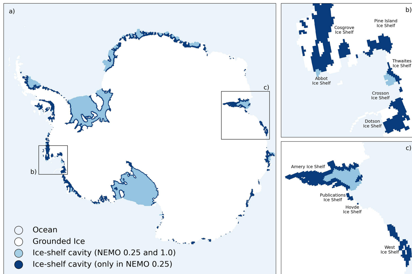
Figure 1. The spatial distribution of ice-shelf cavities which are resolved in the NEMO model at 0.25 and 1°. Panel (a) shows the distribution of cavities resolved at 0.25° (dark and light blue) and the ones that would be resolved at 1.0° (light blue only) for the whole Antarctic continent, illustrating that although the largest ice shelves are resolved in the 1.0° model, many important and fast-changing regions require a higher resolution for sub-ice shelf dynamics to be included in ocean models. Panels (b) and (c) show zoomed-in insets for the Amundsen Sea sector and Amery Ice Shelf as examples. We use the regions which are only resolved in the 0.25° simulations (dark blue) for training the neural network, with ocean properties there propagated from the area that would be resolved at 1° (light blue area).
