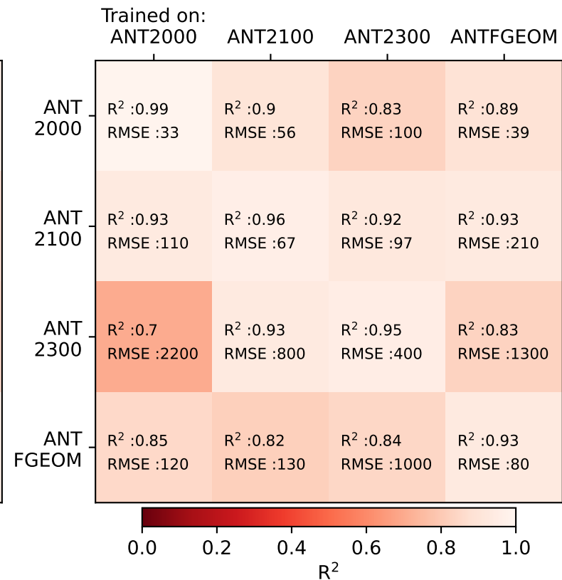
Integrated melt (Gt/yr) whole continent
