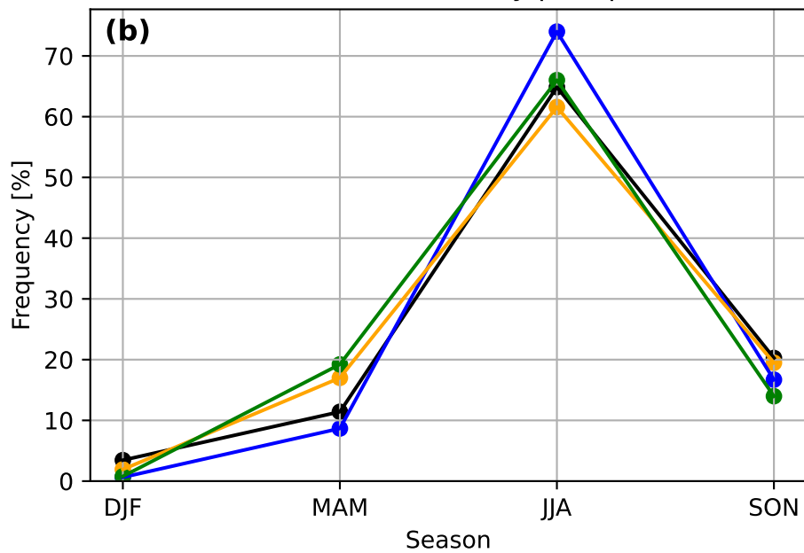
Seasonal cycle of annual-maximum hourly precipitation
