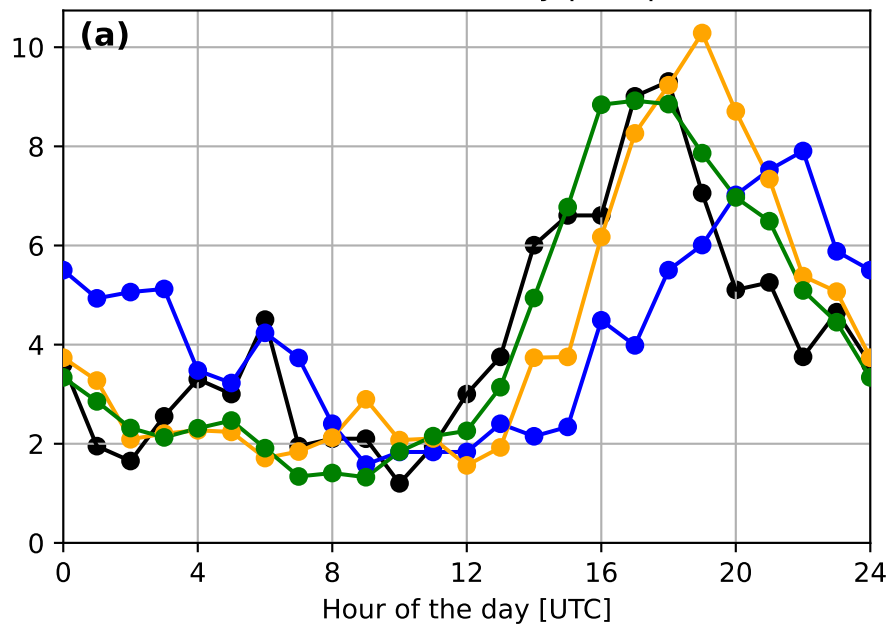
Diurnal cycle of annual-maximum hourly precipitation
