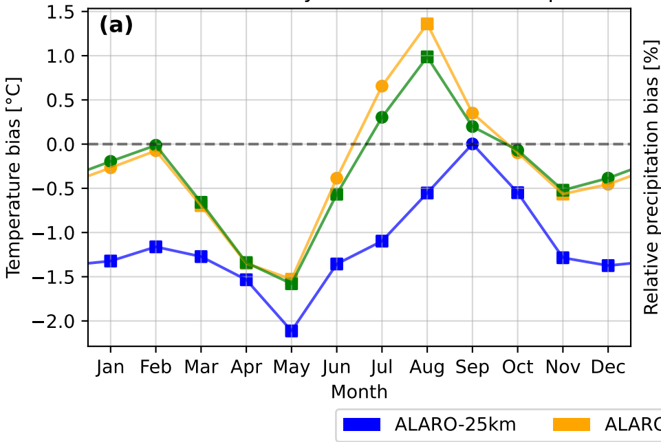
Bias in mean monthly near-surface air temperature
