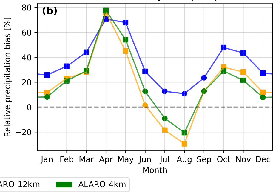
Bias in mean monthly total precipitation
