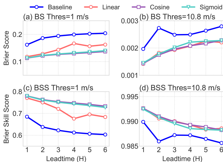
Figure 8. Brier Score (BS) and Brier Skill Score (BSS) of the wind speed ensemble nowcasts as a function of forecast lead time for two wind speed thresholds. (a, c) Threshold: 1 \text{ m s}^{-1} . (b, d) Threshold: 10.8 \text{ m s}^{-1} . In all panels, results are shown for the climatological baseline (blue) and the three DDPM noising schedules: Linear (orange), Cosine (purple), and Sigmoid (teal).
