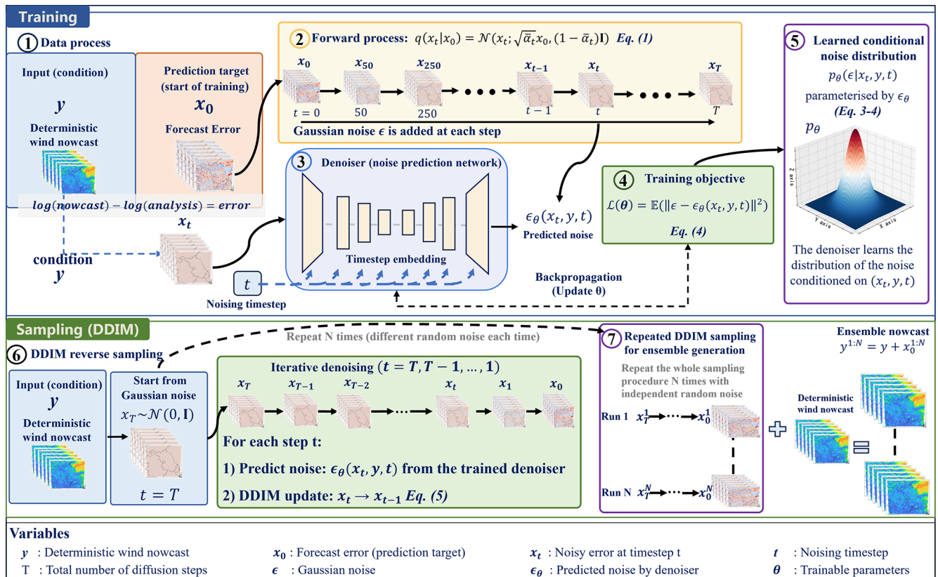
Figure 2. Framework of DDPM.
