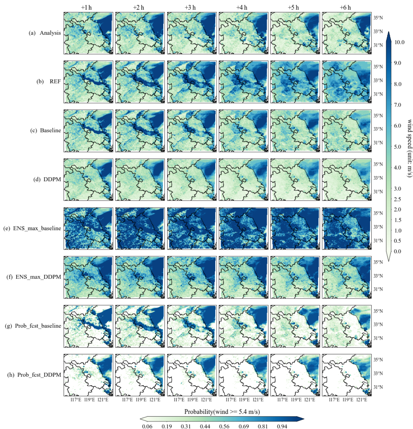
Figure 11. Wind speed from 08:00 to 13:00 UTC on 10 June 2023. (a) Analysis, (b) Deterministic Nowcast (REF), (c, d) Ensemble Mean forecast of baseline and DDPM with cosine schedule, (e, f) ensemble maxima and (g, h) the probability forecast with threshold 5.4 \text{ m s}^{-1} .
