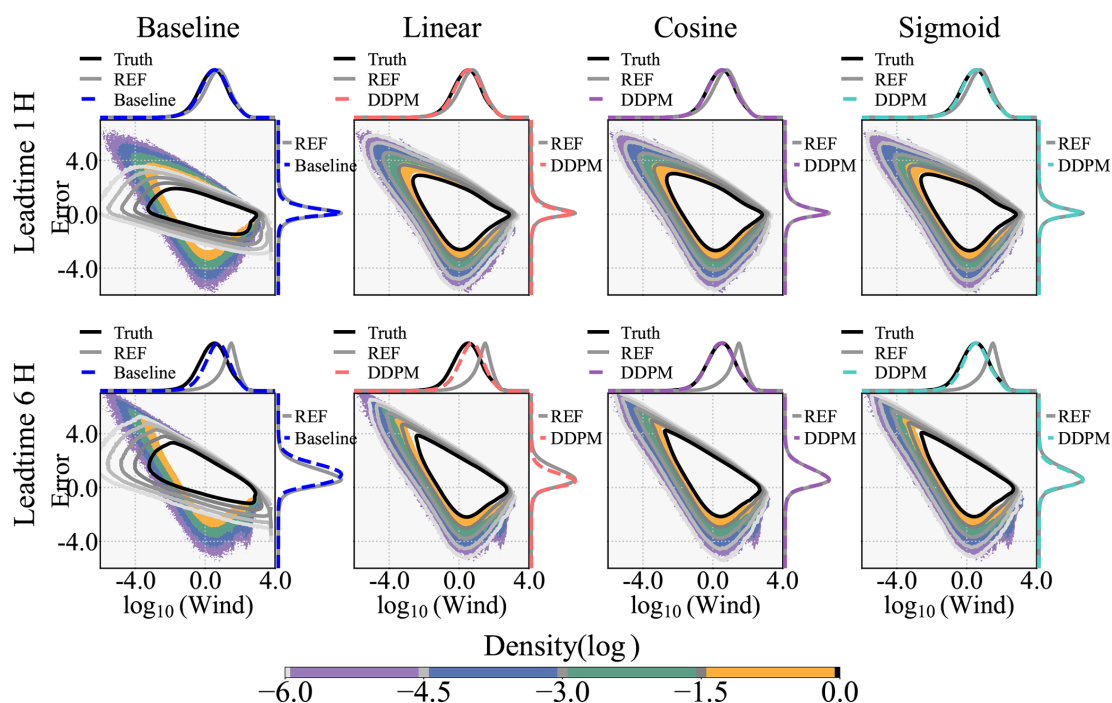
Figure 3. Joint distribution of error and wind speed for the 1 h (top row) and 6 h (bottom row) forecast. The shaded contours and contour lines represent the deterministic reference (REF) and ensemble predictions of baseline or DDPM, respectively. Marginal distributions of logarithmic wind speed (top x axis) and error (right y axis) are shown for observations (Truth, black solid), the deterministic forecast (REF, grey solid), and the DDPM ensemble (dashed).
