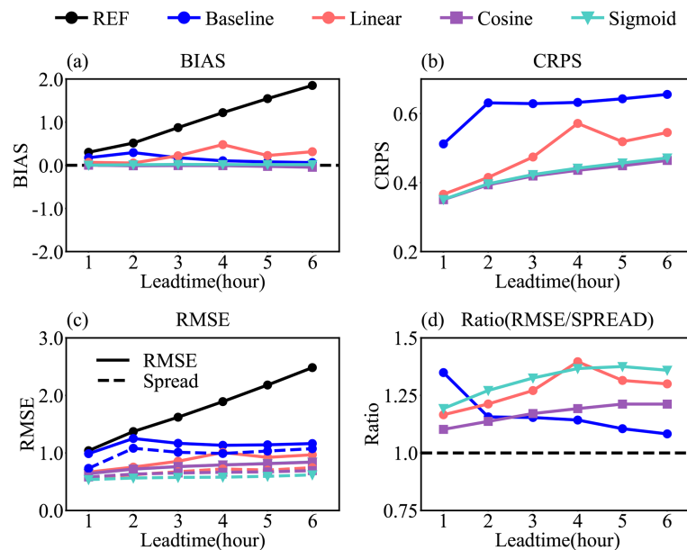
Figure 6. Verification metrics for deterministic and ensemble mean nowcasts over the test period. (a) BIAS, (b) CRPS, (c) RMSE (solid lines) and ensemble spread (dashed lines). (d) Ratio of RMSE to SPREAD. In all panels, the black solid line denotes the deterministic nowcast (REF), the blue line represents the ensemble nowcasts from the climatological baseline, while the orange, purple, and teal lines correspond to the three DDPM noising schedules (Linear, Cosine, and Sigmoid), respectively.
