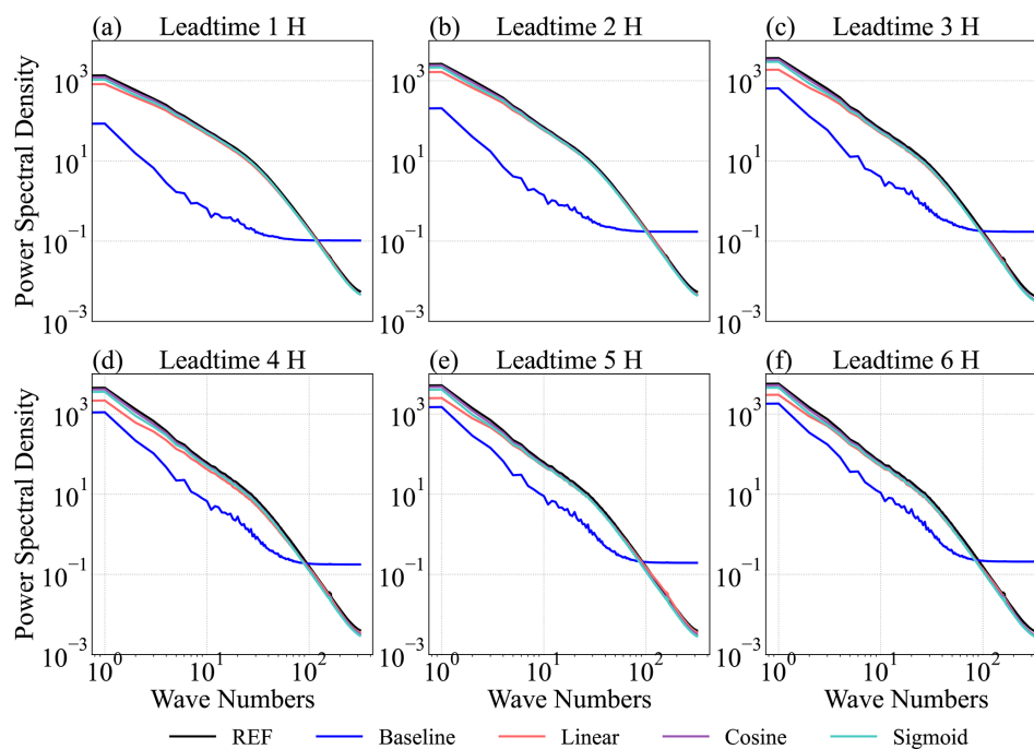
Figure 4. Comparison of power spectra density for Errors in different forecast lead time. The black and blue solid lines denote the errors of deterministic nowcast (REF) and baseline, respectively. While the orange, purple and teal solid lines denote DDPM predictions with different noising schedule (Linear, Cosine and Sigmoid).
