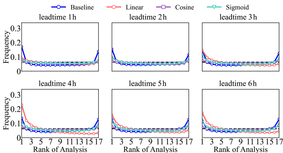
Figure 9. Talagrand Diagrams of wind ensemble nowcasts for different ensembles.
