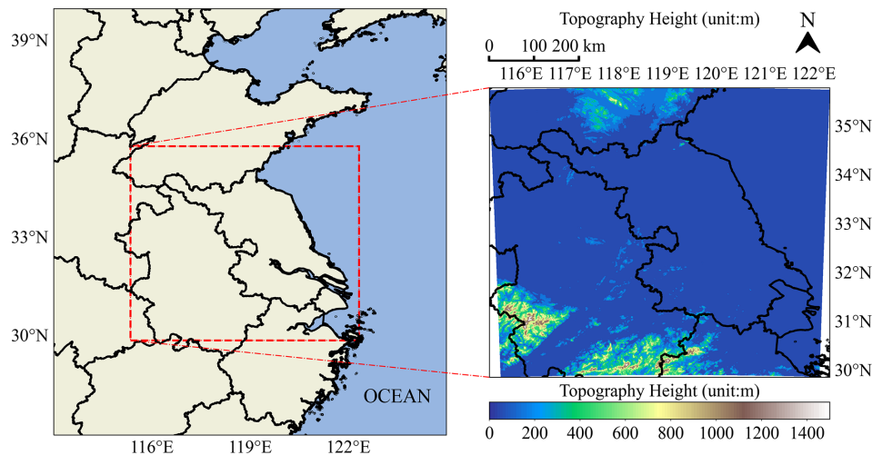
Figure 1. Domain of the dataset (left) and the corresponding topography elevation above sea level (right).
