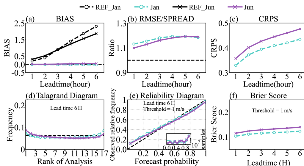
Figure 13. Verification metrics for ensemble nowcasts in January 2023 (dashed teal, \circ ) and June 2023 (solid purple, \times ). (a) BIAS, (b) Ratio of RMSE to SPREAD, (c) CRPS, (d) Talagrand Diagram, (e) reliability diagram, (f) Brier score. In panel (a), the black dashed and solid lines denote the deterministic nowcast (REF) for January and June, respectively.
