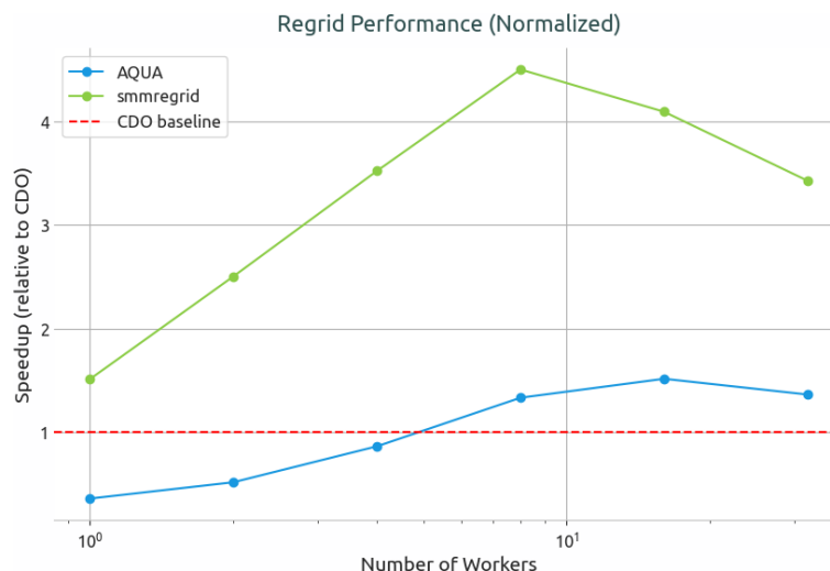
Figure 6. Strong scaling for the regrid operation done with AQUA (blue line, embedding smmregrid package for the regrid) and smmregrid alone (green line), with daily chunking and various number of workers. Times are normalized with respect to the same operation done with serial 1-core CDO and represented as speedup with respect to the baseline, which is represented as a dashed red line.
