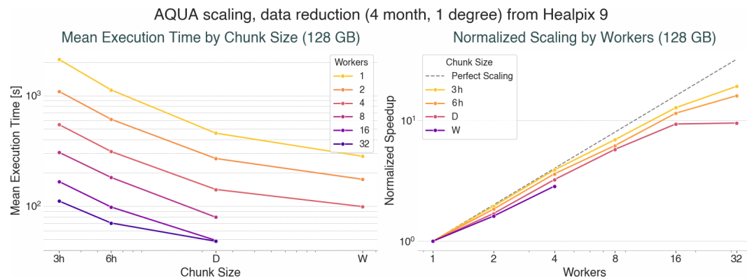
Figure 5. Scaling of the AQUA core functionalities. Both the panels refer to a data reduction setup as described in Sect. 4. The left panel represents the mean total execution time for different worker numbers at different Dask chunk sizes, ranging from 3 h to weekly chunk size. The right panel represent the strong scaling. Different lines for different chunk sizes are shown with an increasing number of workers used, from single thread to 32 workers. The y-axis represents the normalized speedup, whereas the baseline for the normalization is the serial execution of the respective chunk size. The dotted line represents the perfect scaling, where doubling the number of workers doubles the speedup.
