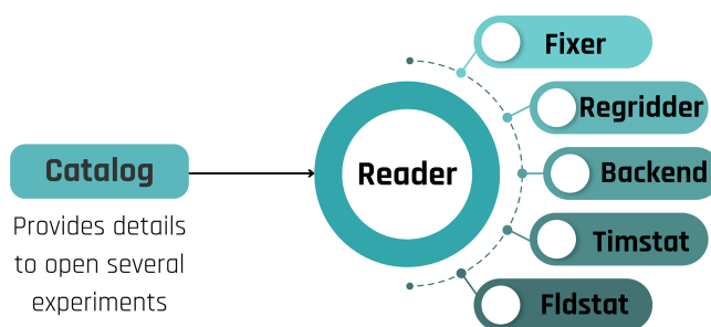
Figure 3. A view of the main component of the AQUA framework code. On the left is the Catalog, described in Sect. 3.1, which provides the details to access climate data. On the right is the Reader class. It constitutes the core of the code, where the other classes depicted in this diagram are modular and available inside any Reader initialization if enabled by the user requirements.
