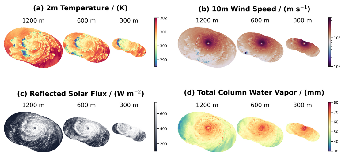
Figure 8. An overview of various variables, shown in the respective nests for a specific grid segment. The grid configuration was chosen so that the re-initialization time is 12 h and the nests have an across-track width of 300, 200, and 100 km, respectively (narrow-size setup). The equivalent grid spacing is indicated above the respective nest. Variables shown are (a) 2 m temperature, (b) 10 m wind speed, (c) reflected solar radiation flux at TOA and (d) total column water vapor for segment 11 at 18:00 UTC on 12 September 2020.
