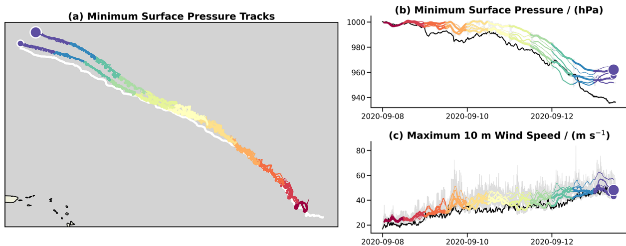
Figure 7. Simulated hurricane characteristics for grid configurations with differently chosen across-track widths. (a) The minimum pressure positions are plotted on a map, with colors representing the respective grid segments. The re-initialization time between successive segments is set to 12 h. The narrow-size setup (small, solid circle at the end of the track) is compared to the medium-size setup (larger, solid circle at the end of the track). Different resolutions are plotted with different line thicknesses, ranging from thick for R2B11 to thin for R2B13, and they partially overlap. Minimum pressure positions from the base run are plotted in white. The minimum pressure and maximum 10 m wind speed are presented using similar color and line encoding as in (a). A running-average filter is applied to the curves in (b), (c) to reduce noise. The original data is shown in light gray shading in the background. Data from the base run is shown in black.
