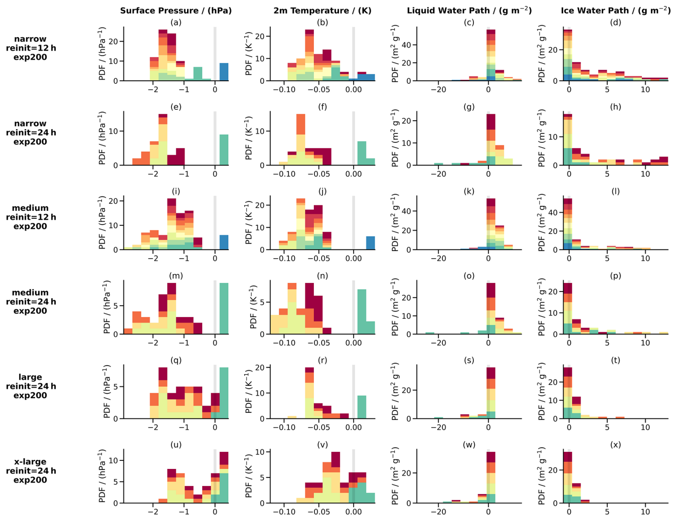
Figure 11. Statistical summary of potential re-initialization effects plotted as colored bars stacked on top of each other for each segment. The color coding is the same as in Fig. 6. At 30 min after initialization of segment k , nine percentiles (10%–90% in 10% steps) of each field are computed across the Lagrangian analysis region separately for segment k and segment k - 1 extended by 3 h, and their pairwise differences are taken. These per-segment differences are statistically summarized as probability density functions. The six rows show the respective setups, with the narrow and medium setups shown for re-initialization periods of 12 and 24 h, respectively. The columns show surface pressure, 2 m temperature, liquid water path, and ice water path. The re-initialization analyses are only shown for the outer nest with a grid spacing of approximately 1 km.
