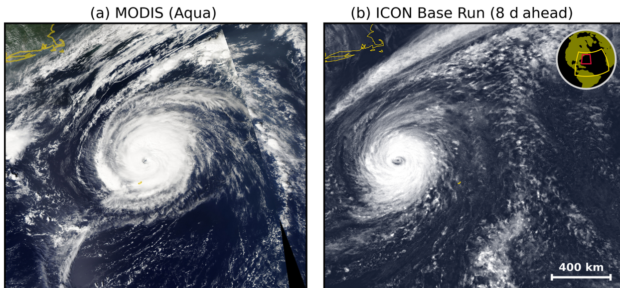
Figure 5. Top view of hurricane Paulette from (a) observations and (b) simulations. A regional cutout in the Atlantic ocean was defined reaching from -74.0 to -53.4^\circ E and from 25.0 – 43.2^\circ N. Subpanel (a) shows a true-colour image acquired by the Moderate Resolution Imaging Spectroradiometer (MODIS) instrument on the NOAA-AQUA satellite during an ascending orbit at overpass time on 14 September 2020, around 18:00 UTC. Subpanel (b) provides a simulation of the reflected solar radiation flux, normalized between 100 and 750 \text{ W m}^{-2} from our ICON base run, which was initialized on 7 September 2020 at 00:00 UTC. The time, geographical region and projection have been matched between the observation and the simulation. The color scale and map in (b) have been adjusted to ensure visual consistency with (a). The length scale of 400 km is shown in the lower right corner of (b) and the inset in the upper right corner of (b) shows the location of the image cutout (red outline) and the inner base run domain (yellow outline) in the Atlantic ocean. MODIS imagery by NASA.
