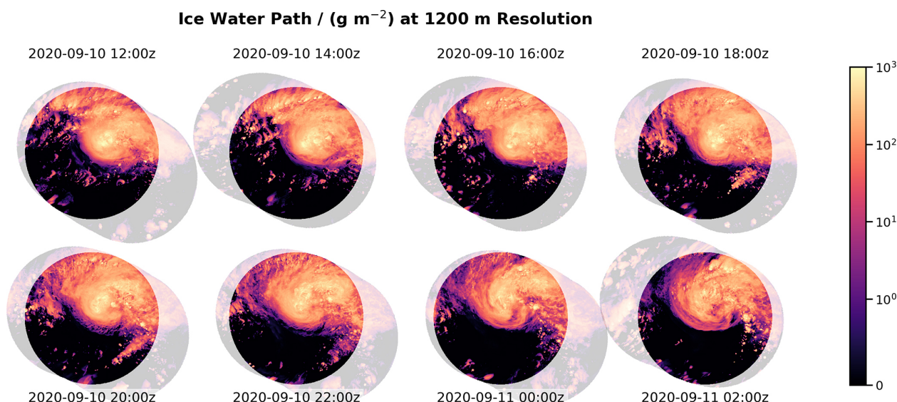
Figure 9. Ice water path is shown as a sequence in a Lagrangian framework. The boldly shaded areas highlight the circular Lagrangian analysis region that follows the track of the reference hurricane. The remaining parts of the respective grid segments are indicated by very light colors. Two-hour steps are made in the temporal sequence. Transitions between segments are visible between the first and second images, as well as between the second-to-last and last images, appearing as shifts in the domain boundaries. Within the Lagrangian analysis region, however, the ice water path evolves smoothly and continuously. Here, the medium-size grid configuration was chosen so that the shown nest (DOM01, 1.2 km grid spacing) has 500 km across-track width with re-initialization time of 12 h.
