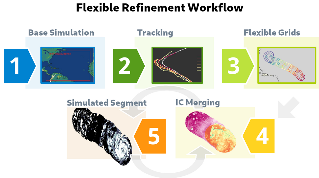
Figure 1. Overview of the flexible refinement workflow: Five steps are shown in different colored boxes and numbered accordingly. The steps of the workflow include (1) creating the base simulation, (2) identifying and tracking the hurricane, (3) creating the flexible grids and other necessary simulation data, (4) combining the initial conditions from the base and newly created simulation data, and (5) performing the actual high-resolution hurricane simulation. Gray arrows indicate the flow in the workflow diagram, with steps 4 and 5 being performed as iterative loop over the respective hurricane segments.
