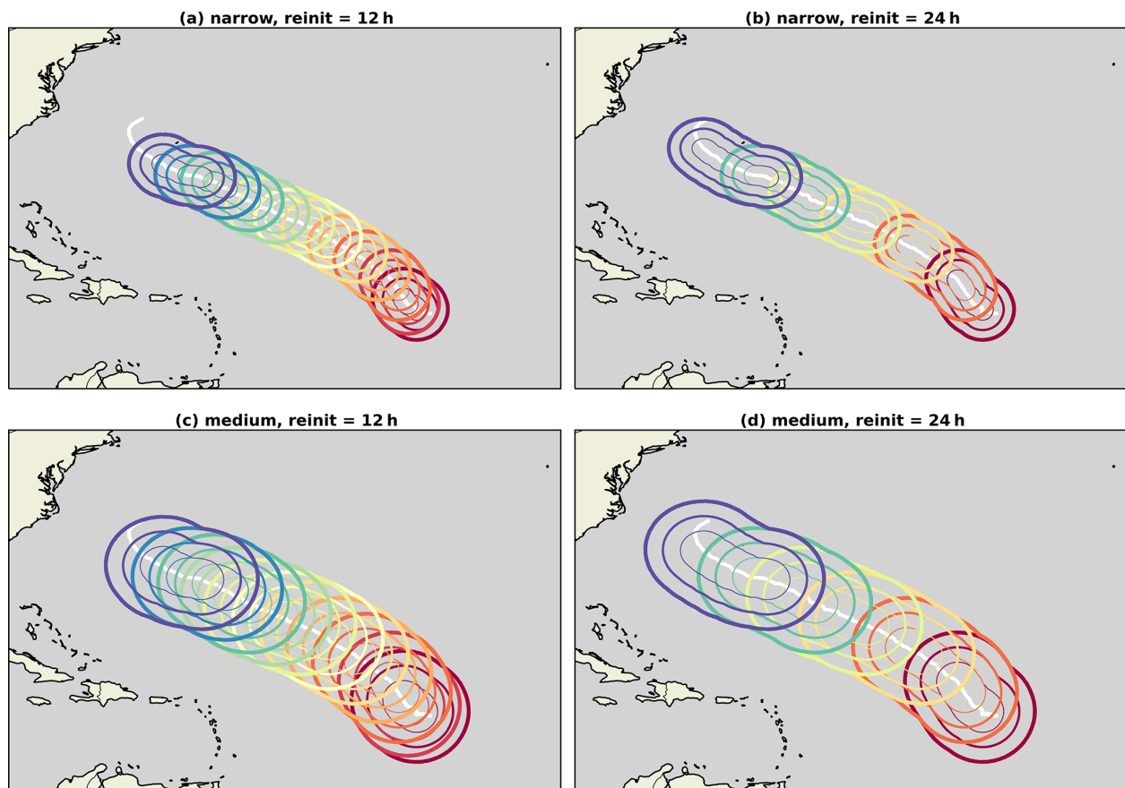
Figure 6. Grid segments prepared for hurricane Paulette (2020) with differently chosen re-initialization times and across-track widths. The narrow setup in (a, b) is compared to the medium setup in (c, d). Re-initialization at 12 h intervals (a, c) leads to twice as many segments as re-initialization at 24 h intervals (see Table 1). The track of the hurricane Paulette in the base simulation is plotted as a white solid line. Each segment consists of three nested domains (solid lines of decreasing thickness) colored by the initialization time, ranging from red on 8 September to blue on 14 September.
