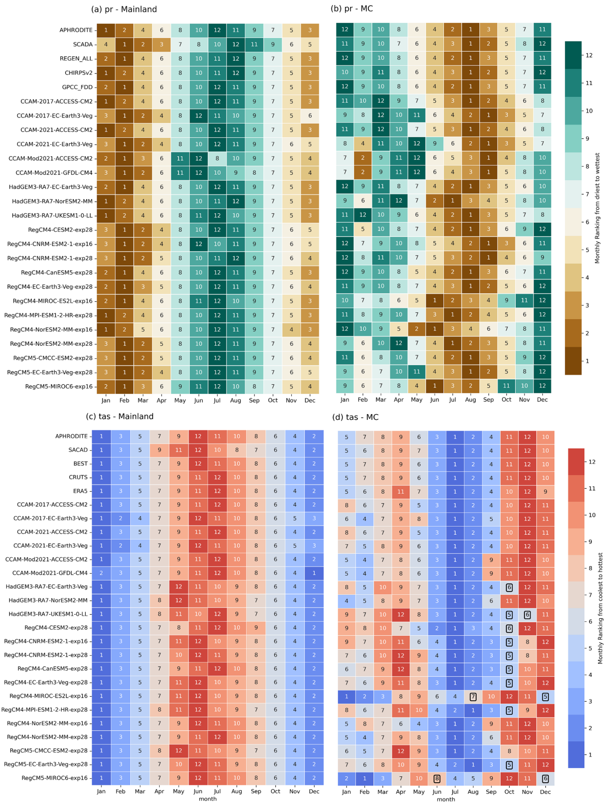
Figure 11. Seasonal cycle benchmark following Isphording et al. (2024) for the unimodal seasonal cycle of (a, b) precipitation (pr) and (c, d) near-surface mean temperature (tas) in the Mainland and MC. Colours and numbers indicate the ranking for latitude-weighted monthly total precipitation/daily temperature, with 1 being the driest/coolest and 12 being the wettest/hottest. The values highlighted in the black box indicate that the simulation does not meet our benchmarking expectations.
