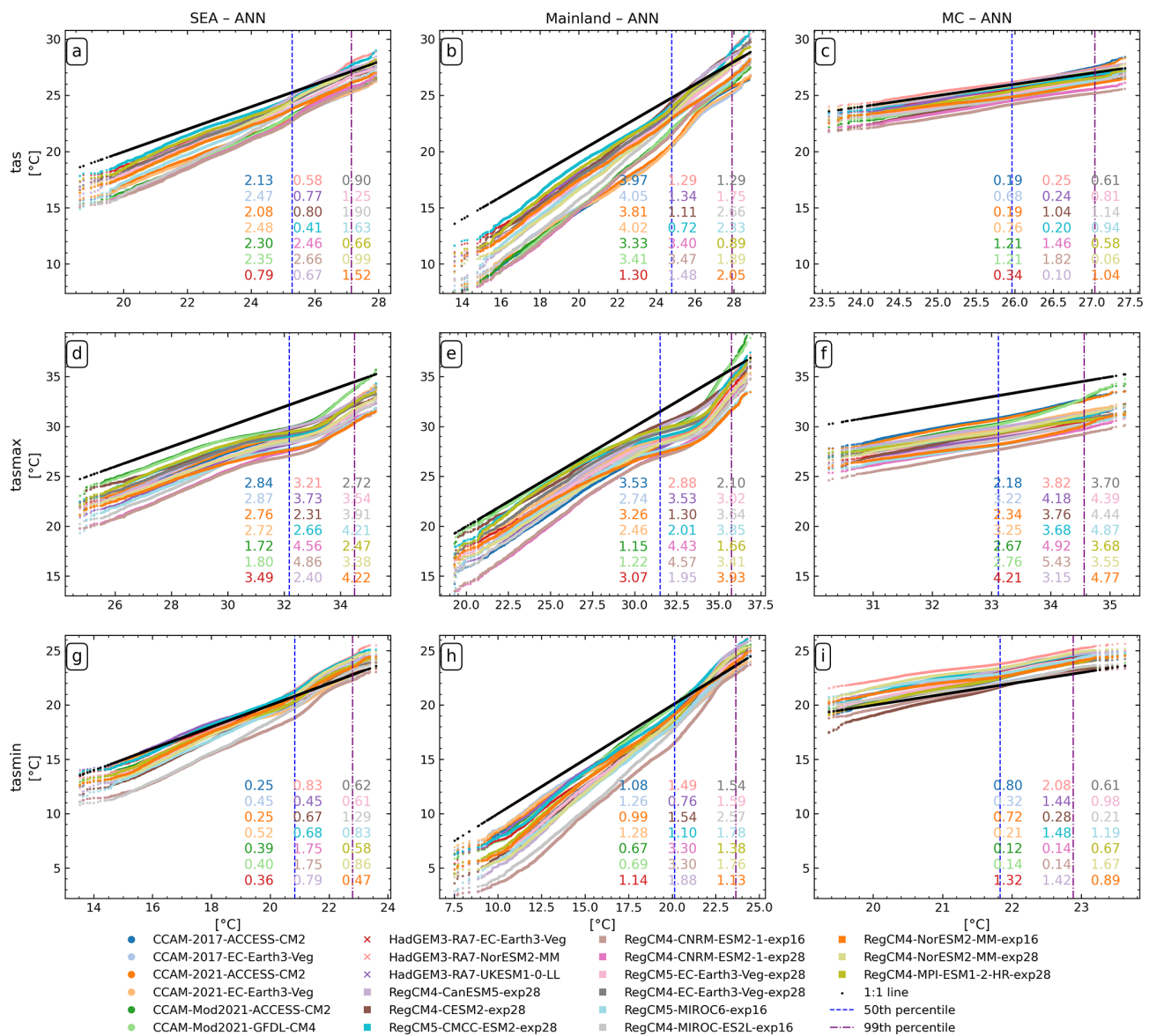
Figure 5. Quantile-quantile plots for regionally averaged daily near-surface temperature (tas, in °C; a–c), temperature (tasmax; d–f), and minimum temperature (tasmin; g–i) across Southeast Asia and its two sub-regions: Mainland (5–27.5° N, 89–147° E) and the Maritime Continent (15° S–5° N, 89–147° E) during the climatological period of 1982–2014. The inserted number indicates the values of the area score metric (ASM; Nguyen et al., 2022), which measures the proximity between the two distributions: the model and the reference (BEST) (Sect. 2.3.1). The vertical lines indicate the 50th percentile (blue) and 99th percentile (purple), respectively.
