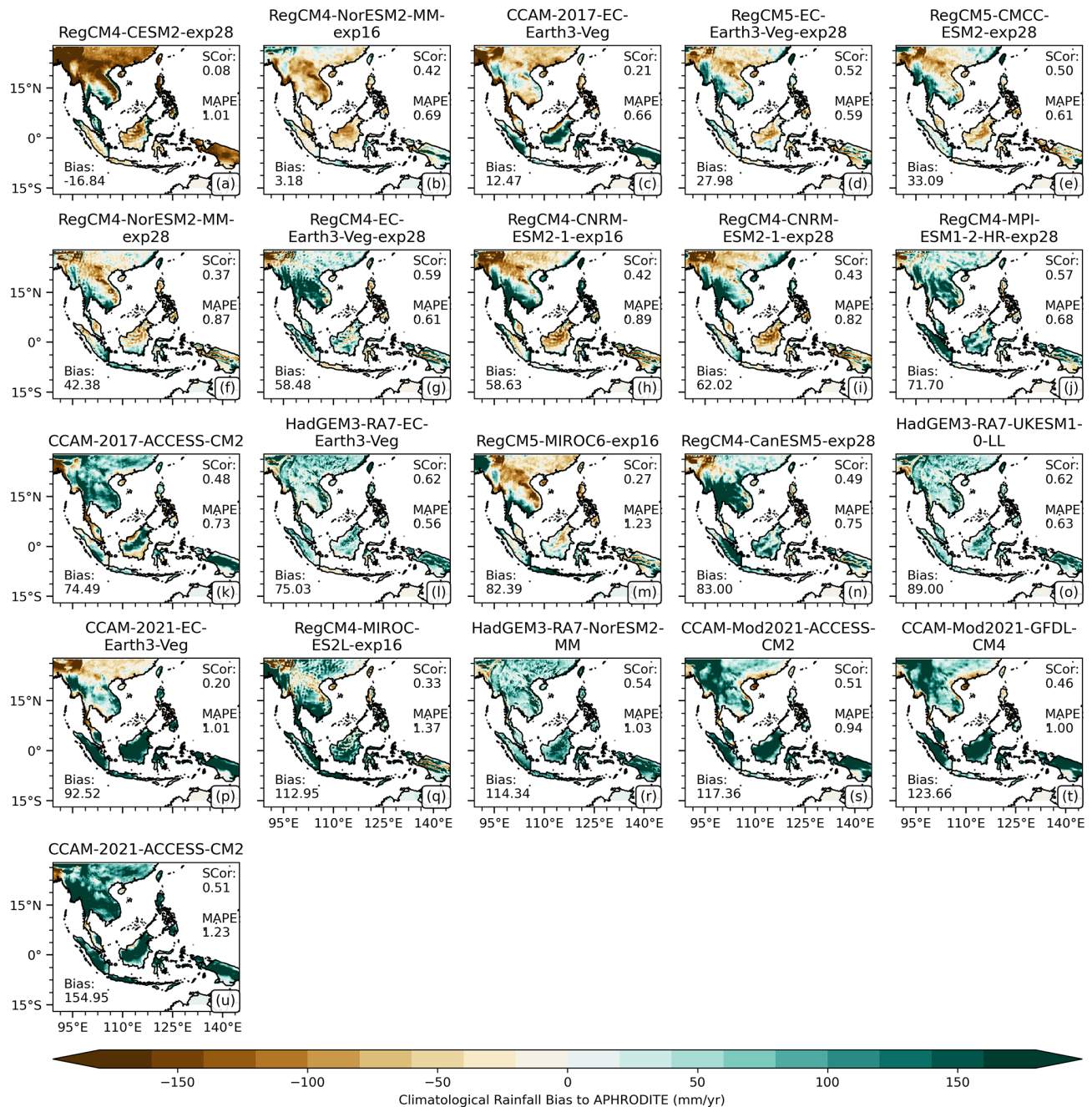
Figure 6. Seasonal climatological (1982–2014) biases (in \text{mm yr}^{-1} ) for each model against the APHRODITE observational product during the May–October (MJJASO) season, ranked from driest to wettest based on regionally averaged bias. The mean absolute percentage errors (MAPEs) and spatial correlations (Scor) calculated against APHRODITE are shown in the upper-right corner. All analyses are considered at the resolution of the CORDEX-SEA simulation (i.e., \sim 25 km). The stippled area indicates locations where RCM shows statistically significant bias ( p < 0.05 ) according to the Mann–Whitney U test.
