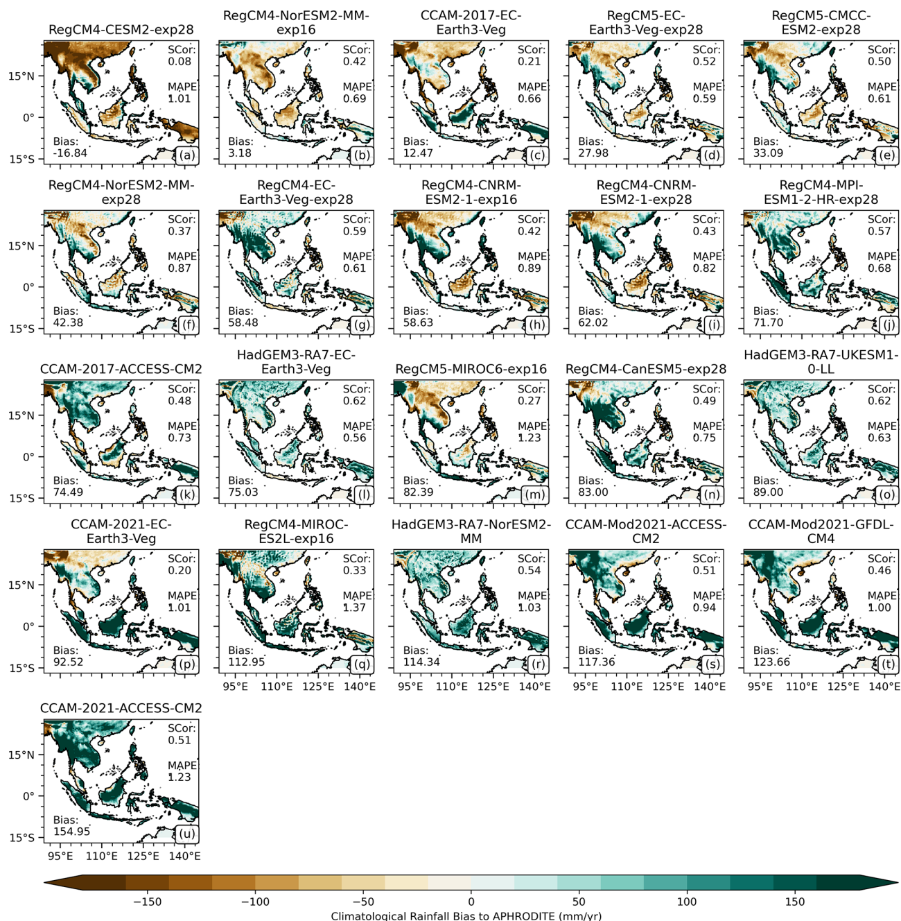
Figure 7. Same as Fig. 6 but for the November–April (NDJFMA) season.
