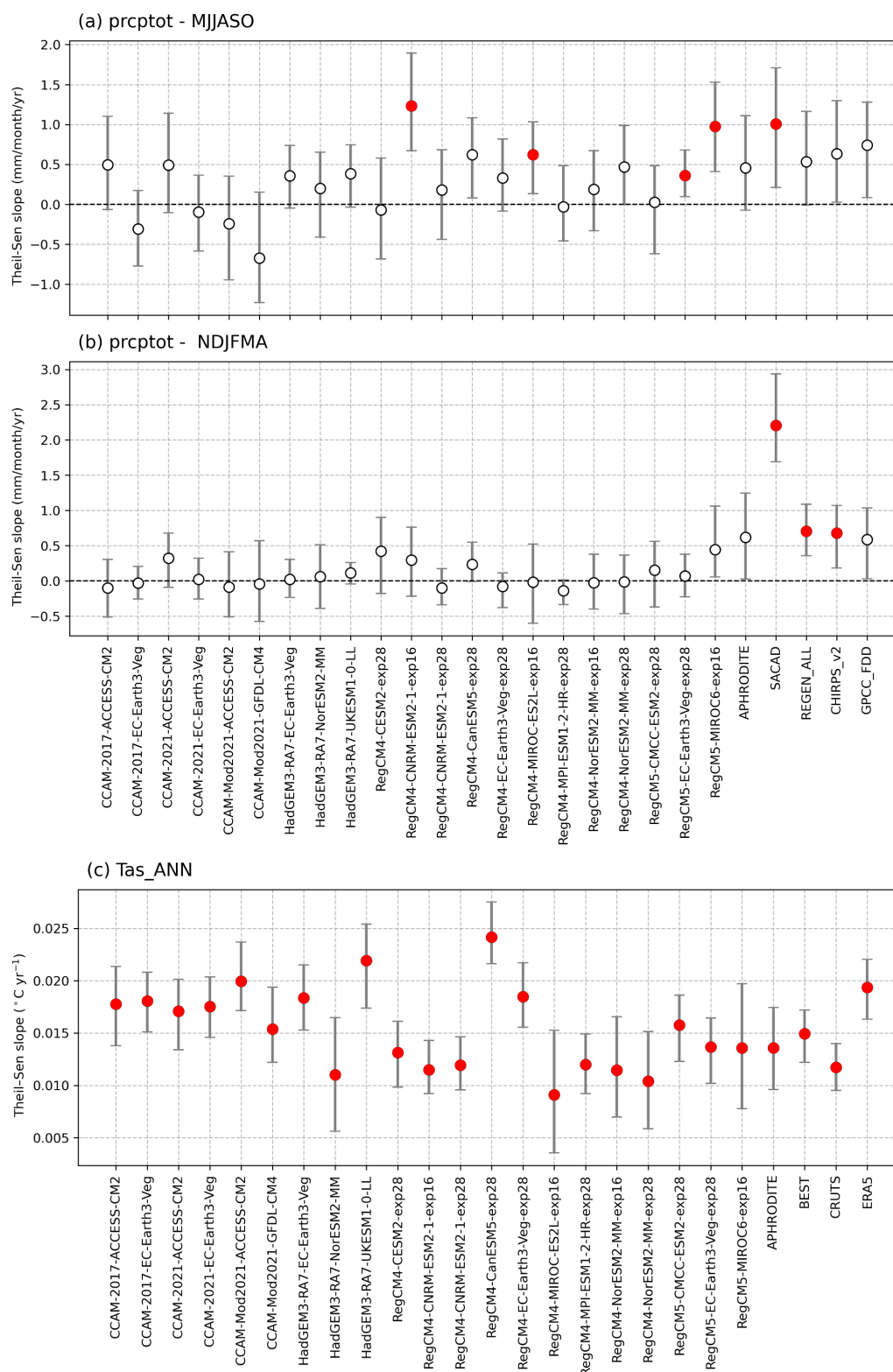
Figure 12. Trend estimated based on the Theil–Sen slope estimator of the time series of seasonal total wet-day precipitation (a, b) and annual near-surface mean temperature (c) among models and observations during 1960–2014. The red dot indicates a significant trend, as determined by the Mann–Kendall test at a 5 % level of confidence. The bar indicates 90 % confidence intervals according to Theil–Sen slope estimator.
