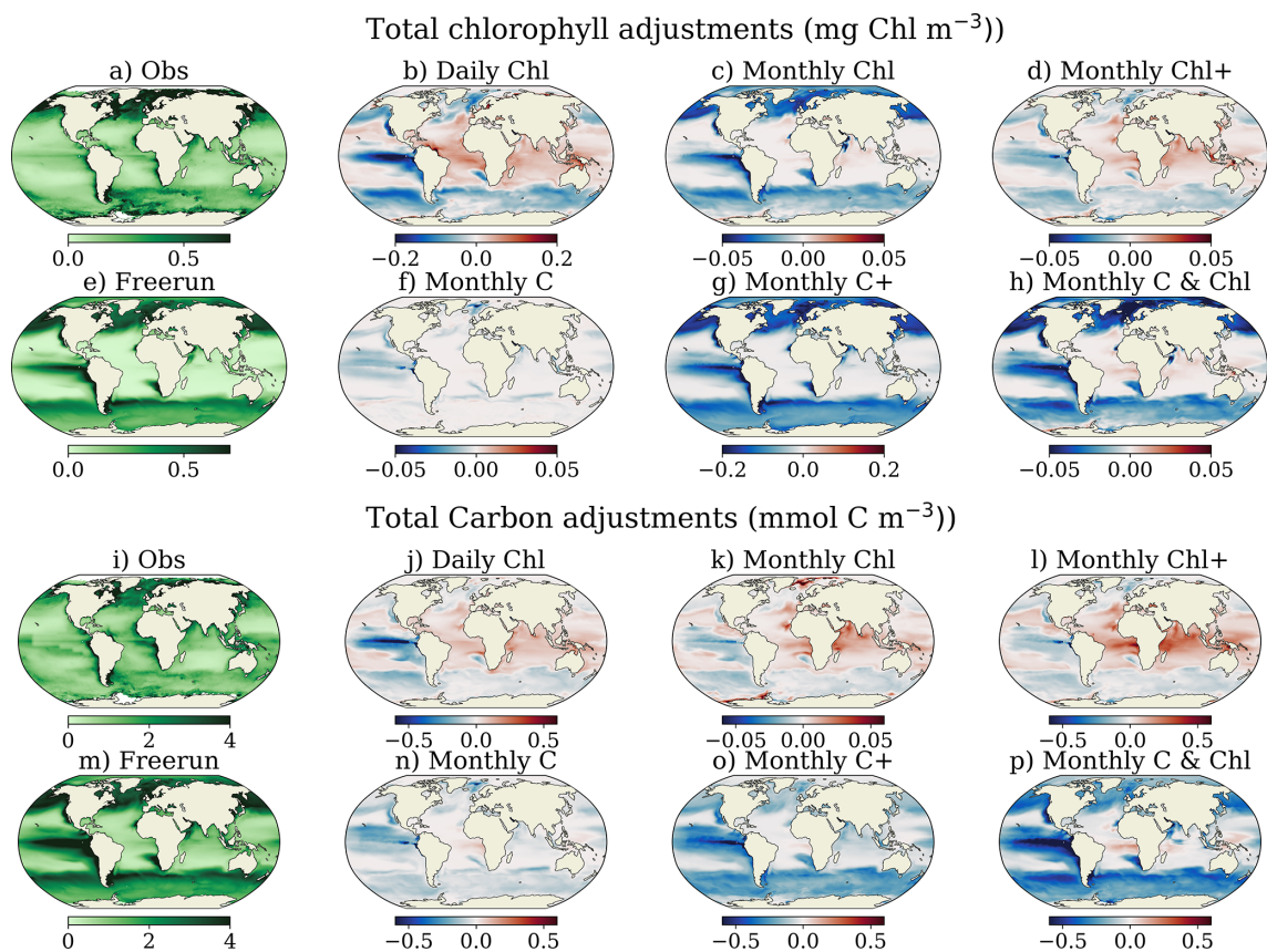
Figure 6. The phytoplankton chlorophyll concentration in (a) observation and Freerun (e) and the differences between the DA experiments and Freerun experiment in (b)–(d) and (f)–(h). The phytoplankton carbon concentration in (i) observation and Freerun (m) and the differences between the DA experiments and Freerun experiment in (j)–(l) and (n)–(p). The differences are computed based on the temporal mean of the ensemble mean of monthly model output over the experiment period. Note that some experiments use a different colour scale.
