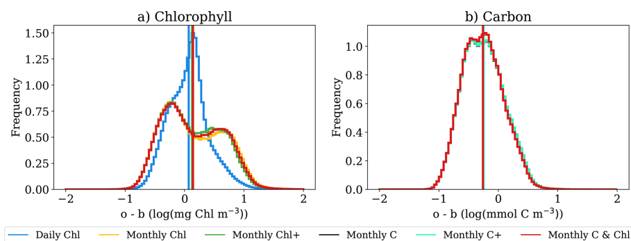
Figure 2. The histogram of the misfit between observations and forecast for log-transformed variables at the analysis step. Large observation and forecast misfits with low probability in (a) are neglected for display purposes. The mean of the misfits for each experiment is presented as vertical lines. This histogram was constructed by global instantaneous data used by DA over the entire experiment period.
