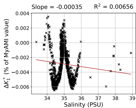
d) K_1^*
