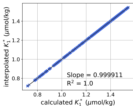
d) K_1^*
