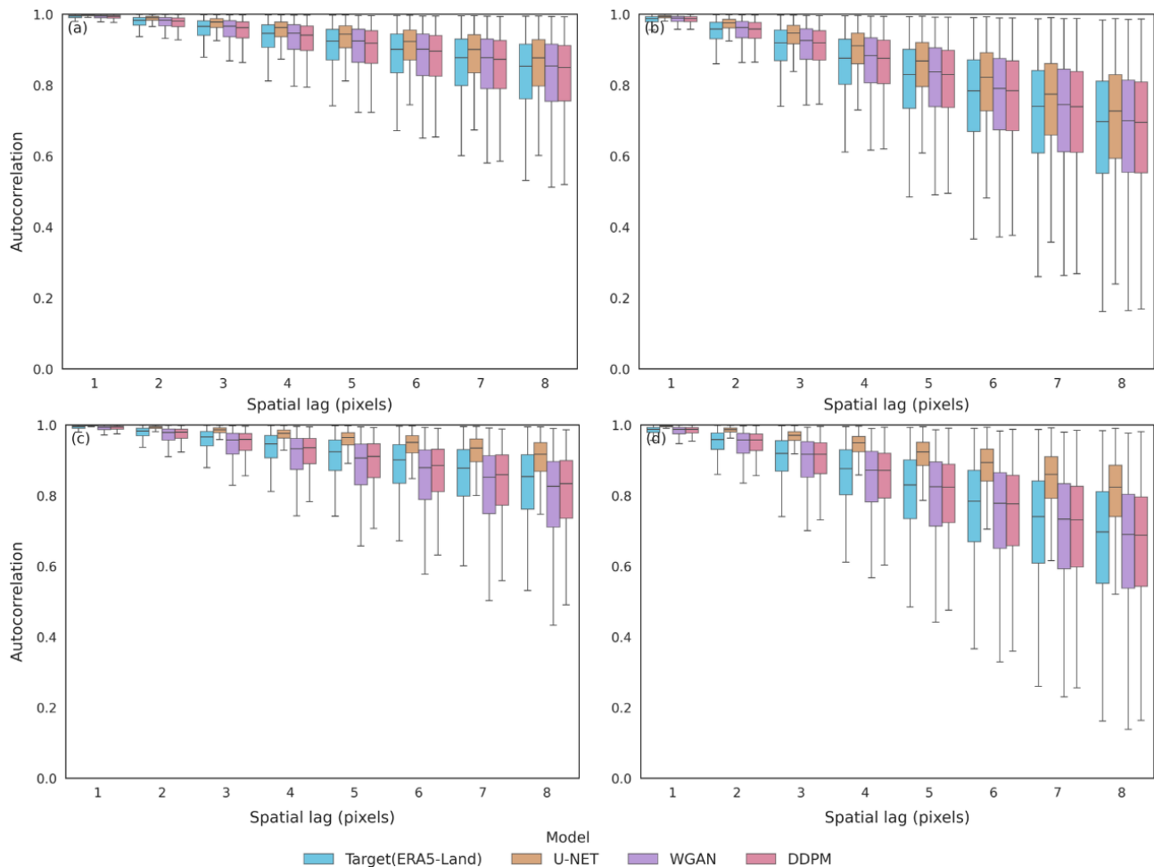
Figure 6. Distributions of horizontal and vertical spatial autocorrelation for lags 1–8 pixels for the ERA5-Land target fields and precipitation fields generated by U-Net, WGAN, and DDPM. Results are aggregated across all test samples and across the 10 independently trained model seeds for each method. Panels (a, b) correspond to the 8× downscaling experiment, while panels (c, d) correspond to the 16× downscaling experiment.
