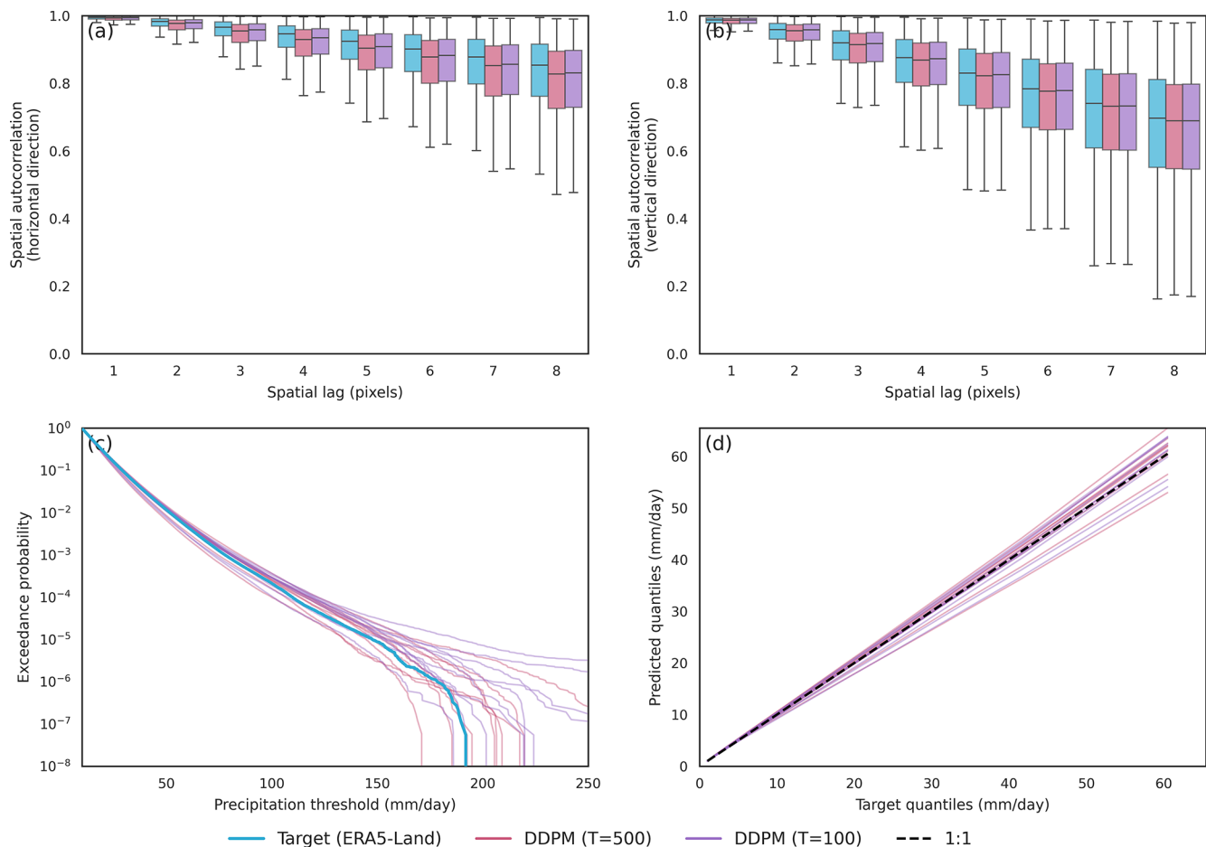
Figure 11. Comparison of DDPM predictions generated using 500 and 100 denoising steps for 16\times precipitation downscaling across ten independently trained seeds. Panels show (a) horizontal spatial autocorrelation, (b) vertical spatial autocorrelation, (c) exceedance probability for precipitation intensities exceeding 10\text{ mm d}^{-1} , and (d) quantile–quantile (Q–Q) relationships relative to Target (ERA5-Land). Boxplots in (a, b) summarize the distribution of spatial correlations across all test samples, while panels (c, d) display individual seed realizations as separate lines. The Target (ERA5-Land) distribution is shown in cyan, DDPM T = 500 in pink, and DDPM T = 100 in purple. The comparison assesses the sensitivity of spatial dependence and precipitation statistics to the number of diffusion inference steps.
