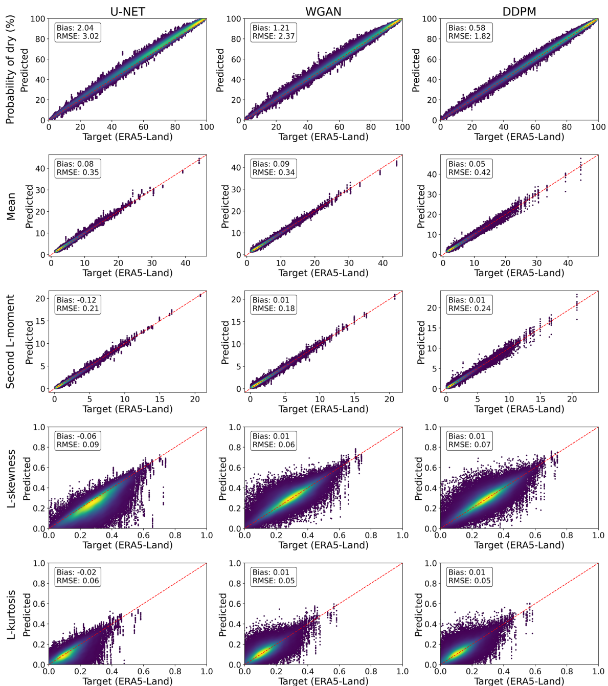
Figure 5. Comparison of precipitation statistics from high-resolution ERA5-Land reanalysis and model predictions for the 16\times downscaling experiment across U-NET, WGAN, and DDPM. Each panel compares reference statistics computed from native high-resolution ERA5-Land fields ( x -axis) with corresponding model predictions ( y -axis), including dry-pixel probability ( P_0 ), mean, second L-moment, L-skewness, and L-kurtosis. Multiple seed-based predictions are evaluated against the same reference samples, leading to repeated x -axis values. Bias and RMSE are shown in each panel.
