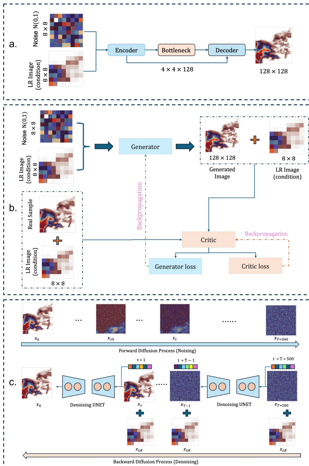
Figure 2. Schematic of the deep-learning architectures used for precipitation super-resolution downscaling (16 \times ). (a) Deterministic U-Net with an encoder–decoder structure and skip connections producing a single high-resolution output. (b) Conditional Wasserstein GAN (WGAN), where a stochastic generator produces high-resolution fields conditioned on low-resolution input and noise and is trained adversarially against a critic. (c) Conditional denoising diffusion probabilistic model (DDPM), which reconstructs high-resolution precipitation through an iterative, noise-to-signal denoising process conditioned on the coarse input.
