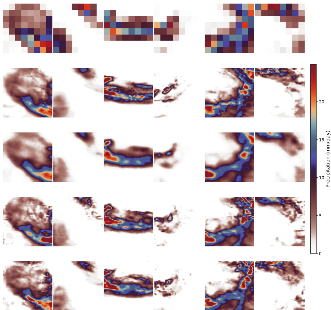
Figure 3. Reconstruction of high-resolution precipitation fields for the 16\times downscaling task ( 8\times 8\rightarrow 128\times 128 ). Columns show six randomly selected test samples, while rows show the low-resolution input, high-resolution target (ERA5-Land), and predictions from U-NET, WGAN, and DDPM, respectively.
