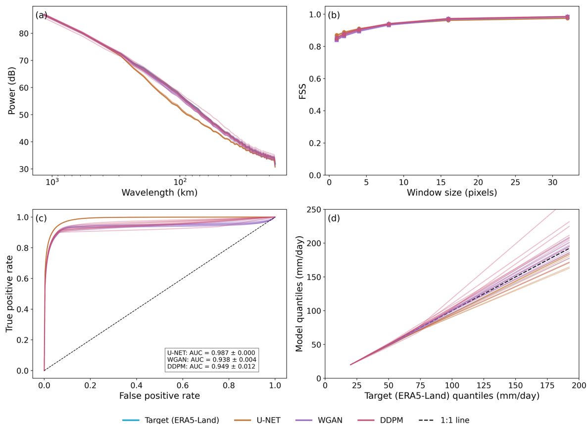
Figure 8. Comparison of U-Net, WGAN, and DDPM performance over the independent Northeast test region at 16\times super-resolution. (a) Radial power spectra showing the distribution of spatial variance across wavelengths relative to the target (ERA5-Land) fields. (b) Fractions Skill Score (FSS) as a function of spatial window size. (c) Receiver Operating Characteristic (ROC) curves for wet-pixel classification, with inset values showing the mean \pm standard deviation of the Area Under the Curve (AUC) across ten independent model initializations. (d) Quantile–Quantile (Q–Q) comparison between model and target precipitation quantiles for precipitation amounts exceeding 20 \text{ mm d}^{-1} . Colored lines represent individual model initializations, and the dashed line in (d) denotes perfect agreement ( 1:1 relationship).
