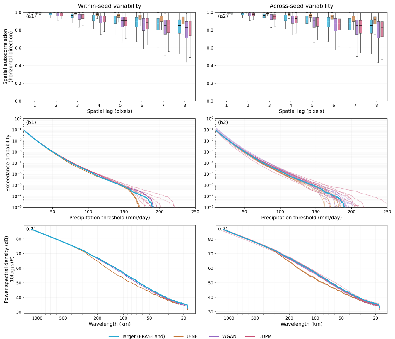
Figure 9. Within-seed and across-seed variability of U-Net, WGAN, and DDPM predictions over the independent Northeast test region at 16\times super-resolution. Panels (a1) and (a2) show boxplots of horizontal spatial autocorrelation at lags 1–8 pixels, where within-seed variability is estimated from multiple stochastic realizations generated by a single trained model and across-seed variability is estimated from independently trained model initializations. Panels (b1) and (b2) present exceedance probability curves as a function of precipitation threshold ( \text{mm d}^{-1} ), illustrating variability in the representation of moderate-to-extreme precipitation intensities. Panels (c1 and c2) show radial power spectra describing the distribution of spatial variance across wavelengths. Left-column panels correspond to within-seed variability and right-column panels correspond to across-seed variability.
