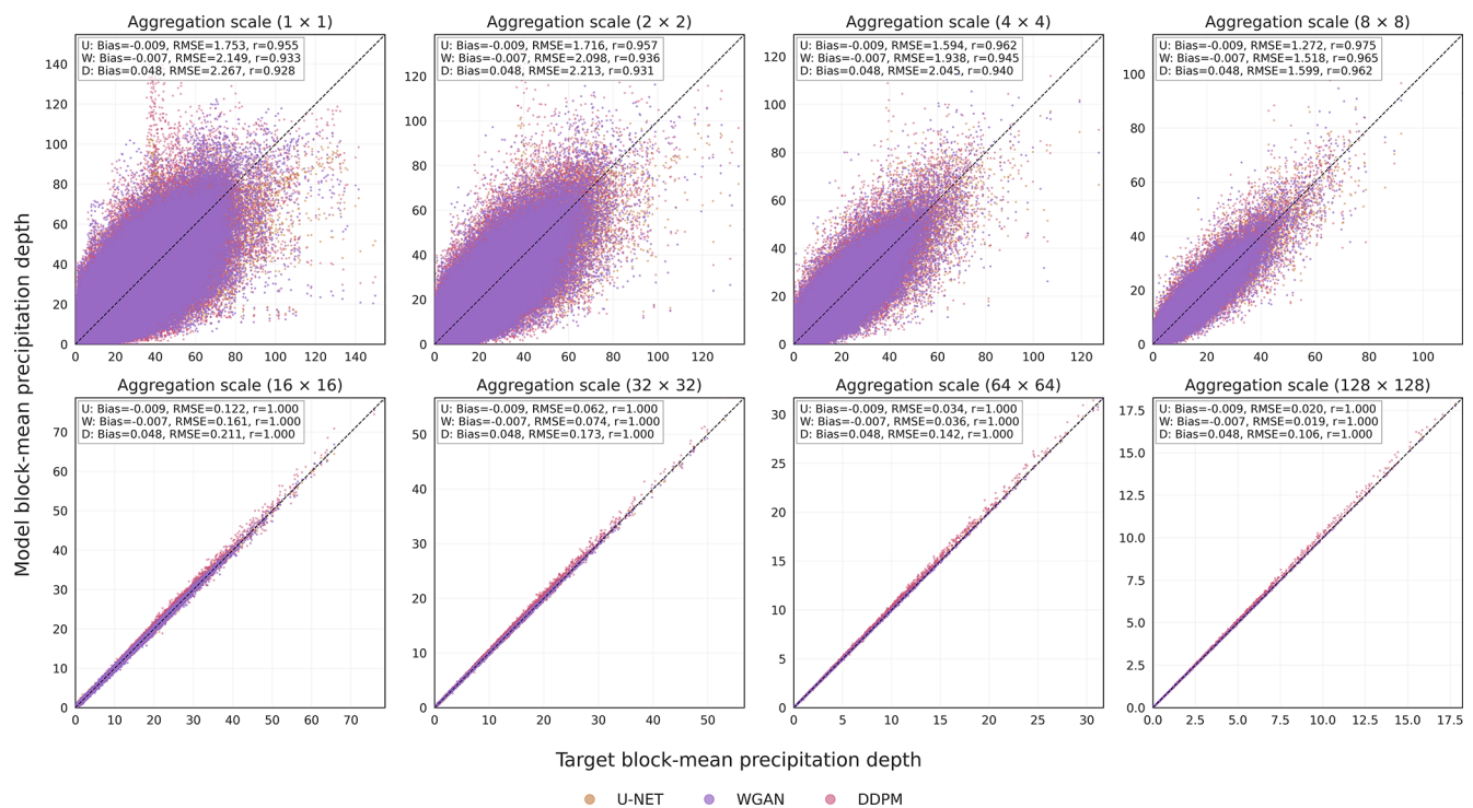
Figure 4. Mass (rainfall depth) consistency across spatial aggregation scales for 16 \times downscaling. Scatter plots compare block-averaged predicted and target (ERA5-Land) precipitation depths at aggregation scales of 1 \times 1 , 2 \times 2 , 4 \times 4 , 8 \times 8 , 16 \times 16 , 32 \times 32 , 64 \times 64 , and 128 \times 128 . Each point represents a spatially aggregated precipitation value computed over the corresponding block size. Results are shown for single seed initialized U-NET (orange), WGAN (purple), and DDPM (pink). The dashed black line denotes perfect 1 : 1 agreement. Panel annotations report model-specific mean bias, root-mean-square error (RMSE), and Pearson correlation coefficient ( r ) at each scale. The analysis was performed using 2000 randomly selected samples from the test set (Northeast region) and one representative model initialization for each generative framework due to the computational expense associated with evaluating the full test dataset and multiple model initializations.
