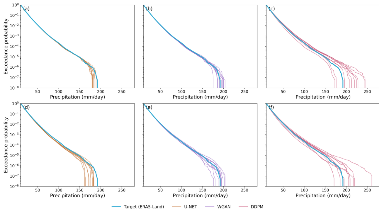
Figure 7. Exceedance probability curves for precipitation generated by U-Net, WGAN, and DDPM across 10 independent seed initializations for the 8\times (a–c) (top row) and 16\times (d–f) (bottom row) downscaling experiments. The Target (ERA5-Land) distribution is shown in blue, while other colored lines represent individual seed realizations. Exceedance probability is displayed on a logarithmic scale to highlight differences in the upper tail of the precipitation distribution.
