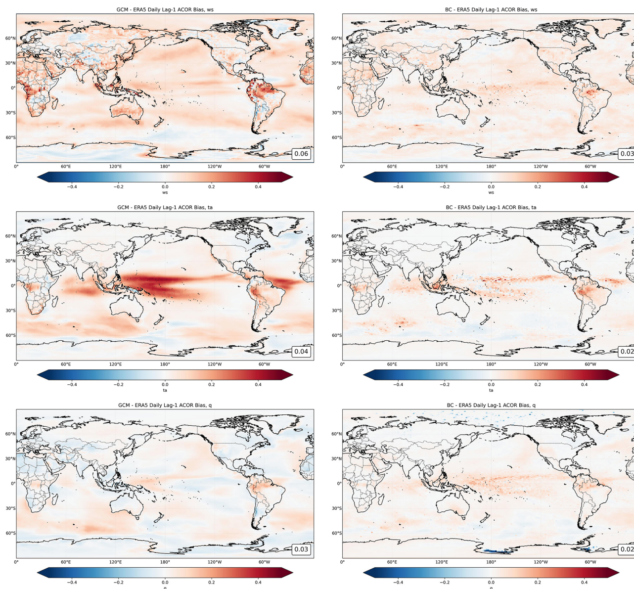
Figure 11. As in Fig. 9, but for lag1 auto-correlation.
