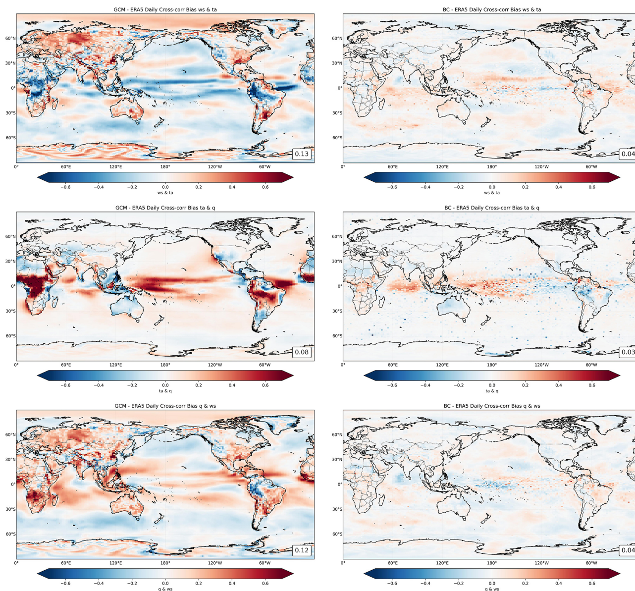
Figure 12. As in Fig. 9, but for cross-correlation.
