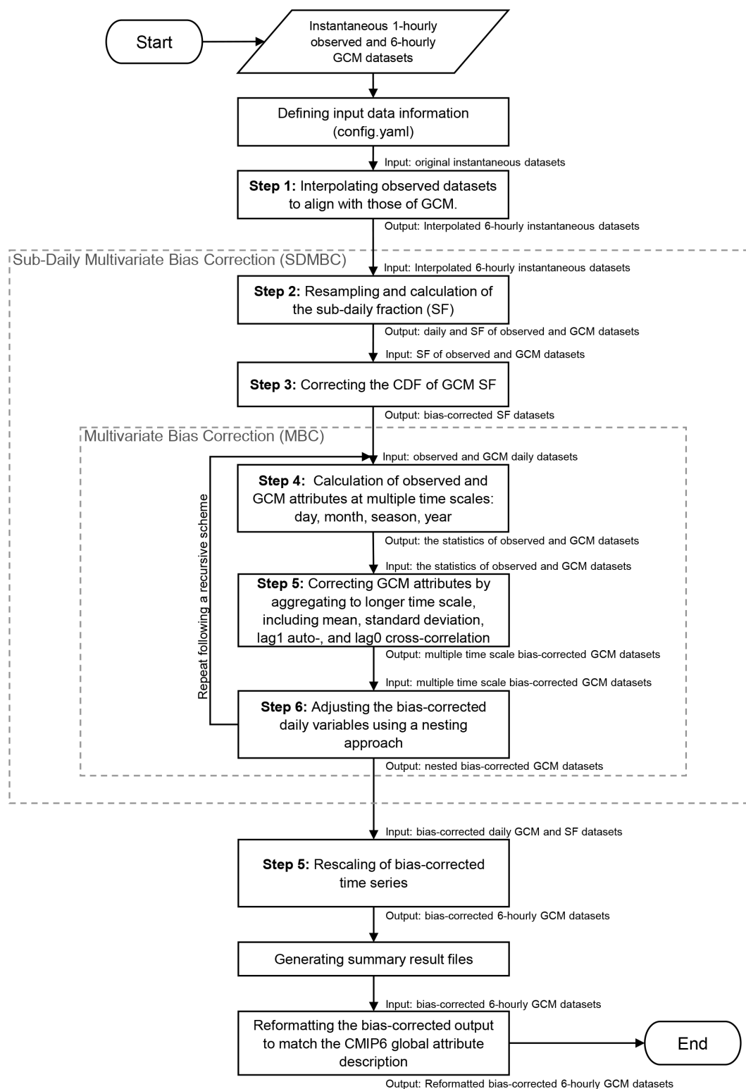
Figure 1. A schematic diagram of SDMBCv2.
