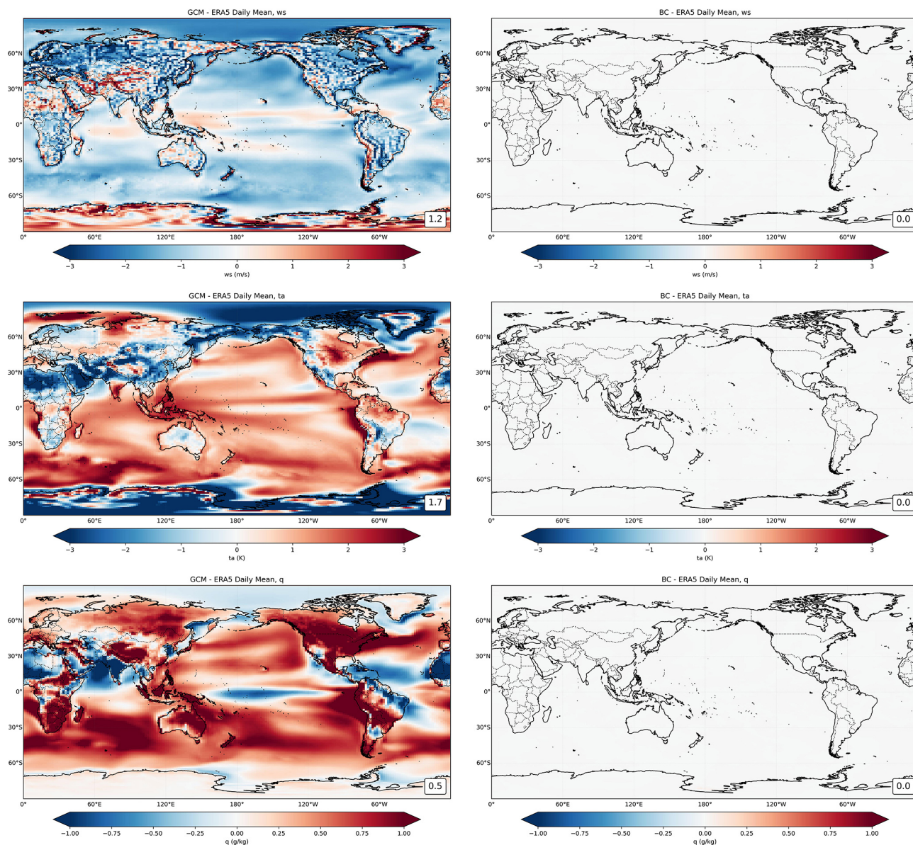
Figure 3. Climatological mean bias maps comparing ERA5 with GCM outputs before (left panels) and after (right panels) bias correction (BC), evaluated at the lowest model level on a daily time scale for the calibration period (1959–1989). The panels show results for wind speed ( ws ), air temperature ( ta ), and specific humidity ( q ). The number at the bottom right shows the mean absolute error.
