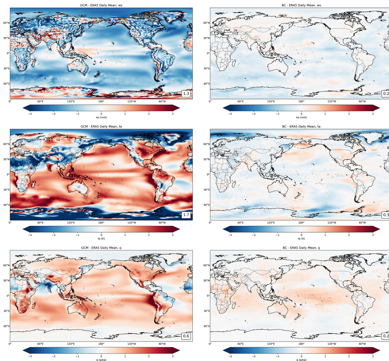
Figure 9. Bias maps of the climatological mean during the validation period (1990–2020), comparing uncorrected (GCM) and bias-corrected GCM outputs (BC) against ERA5 for three key atmospheric variables at the lowest model level. The left panels illustrate the raw GCM, while the right panels show the results after applying SDMBCv2. The number at the bottom right shows the mean absolute error.
