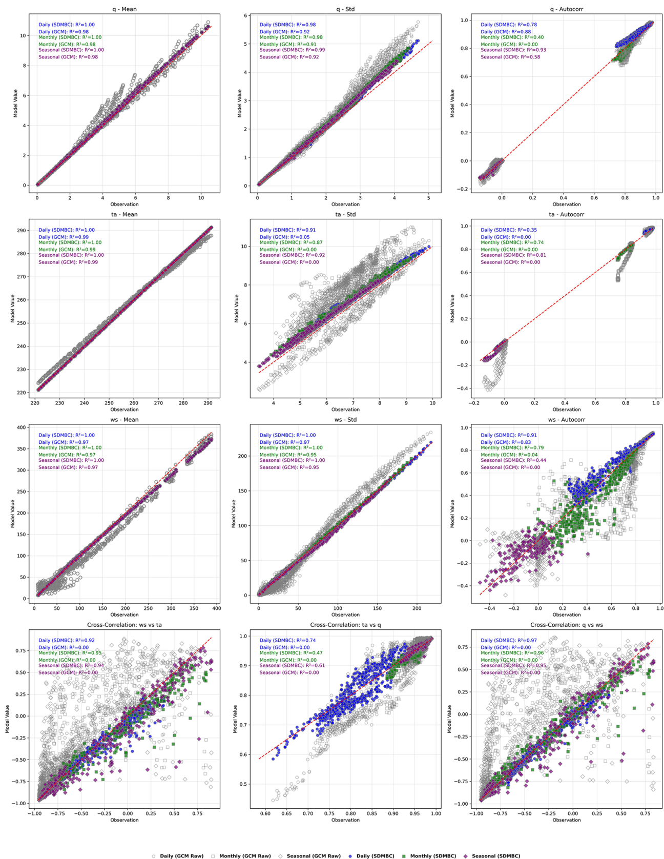
Figure 13. As in Fig. 7, but for validation periods from 1990 to 2020.
