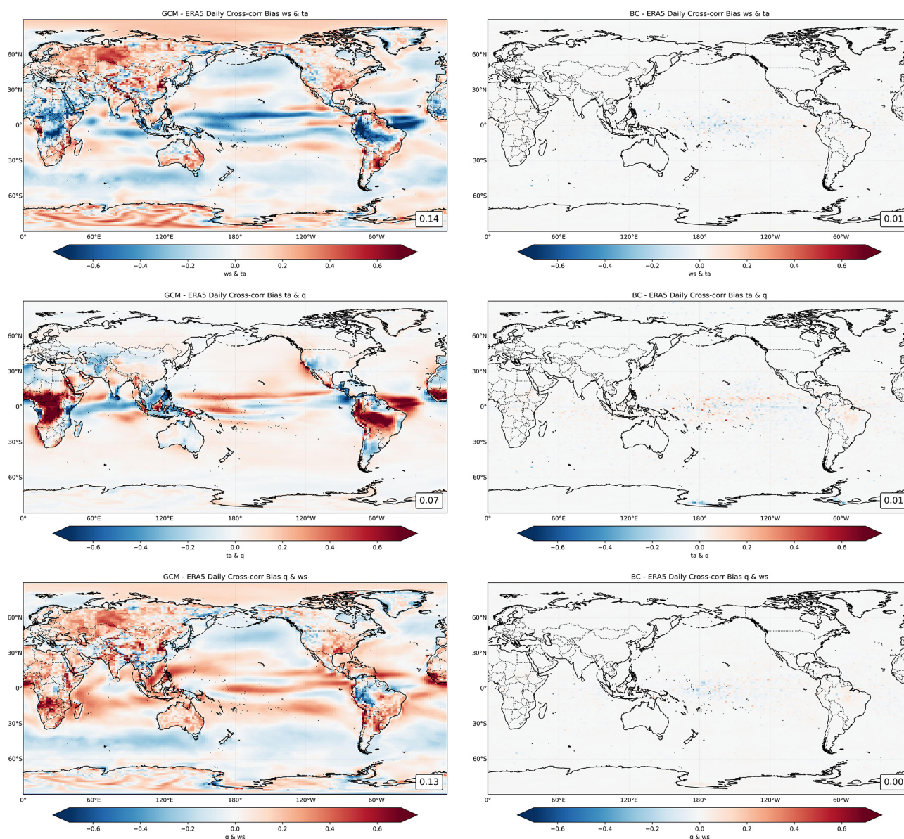
Figure 6. As in Fig. 3, but for lag0 cross-correlation.
