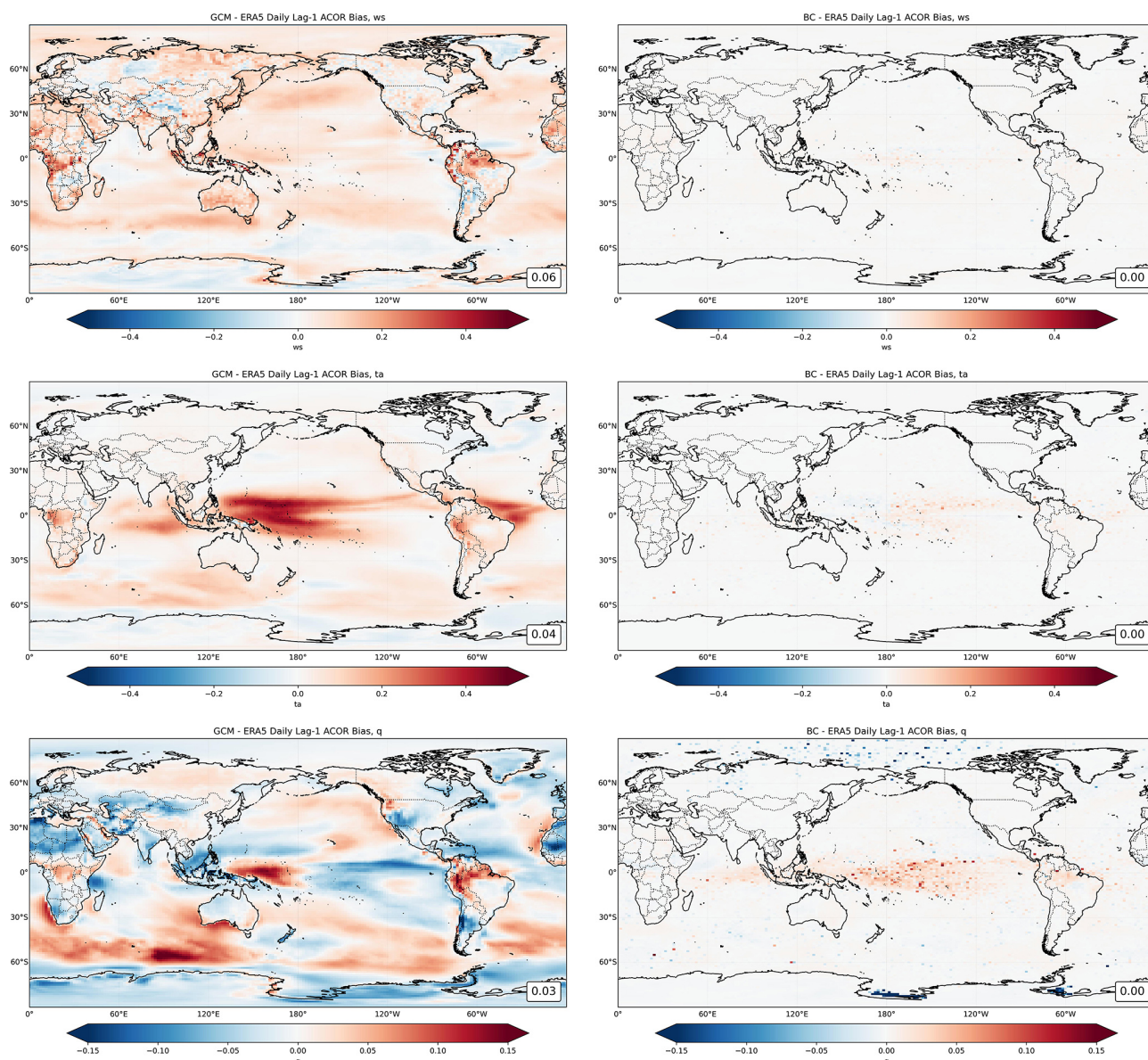
Figure 5. As in Fig. 3, but for lag1 auto-correlation. Domain-averaged MAE values are shown; very small errors ( \sim 10^{-3} ) appear as 0.00 due to rounding.
