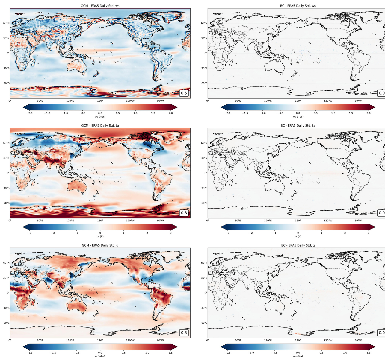
Figure 4. As in Fig. 3, but for standard deviation.
