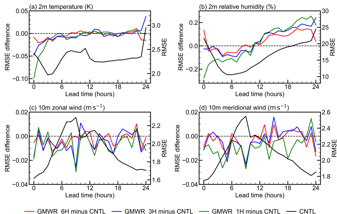
Figure 11. Verification of the forecasts against surface station observations, based on the 10 d assimilation experiment conducted from 13 to 22 October 2023. RMSE (black line) for the CNTL experiment and RMSE differences (colored lines) between the assimilation experiments and the CNTL experiment for (a) temperature, (b) relative humidity, (c) zonal wind, and (d) meridional wind.
