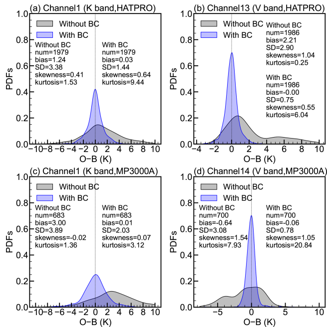
Figure 6. Probability density functions (PDFs) of the O - B distributions, based on a test set randomly selected from 30 % of the three-month sample dataset collected from August to October 2023. The top and bottom rows correspond to the HATPRO and MP3000A sensors, respectively, while the left and right columns represent the K-band and V-band, respectively. Each panel displays the number of samples (num), the mean (bias), standard deviation (SD), skewness, and kurtosis of the distributions.
