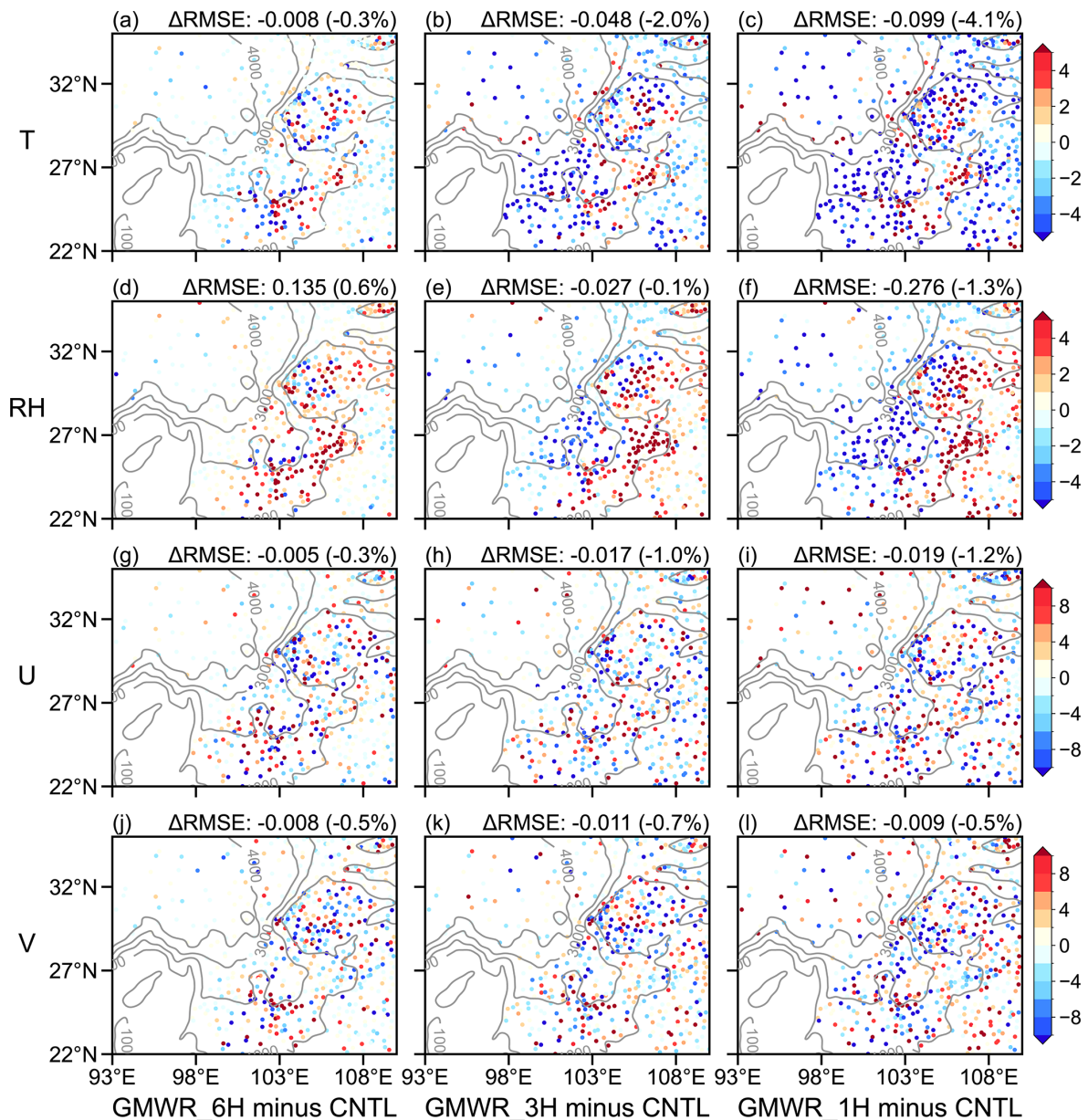
Figure 10. Verification of the initial conditions against surface station observations, based on the 10 d assimilation experiment conducted from 13 to 22 October 2023. The percentage differences in RMSE (scatter) of temperature ( T ), relative humidity ( RH ), zonal wind ( U ), and meridional wind ( V ) in the target region of Southwest China (green rectangle in Fig. 1). The grey solid line represents the topography height (m).
