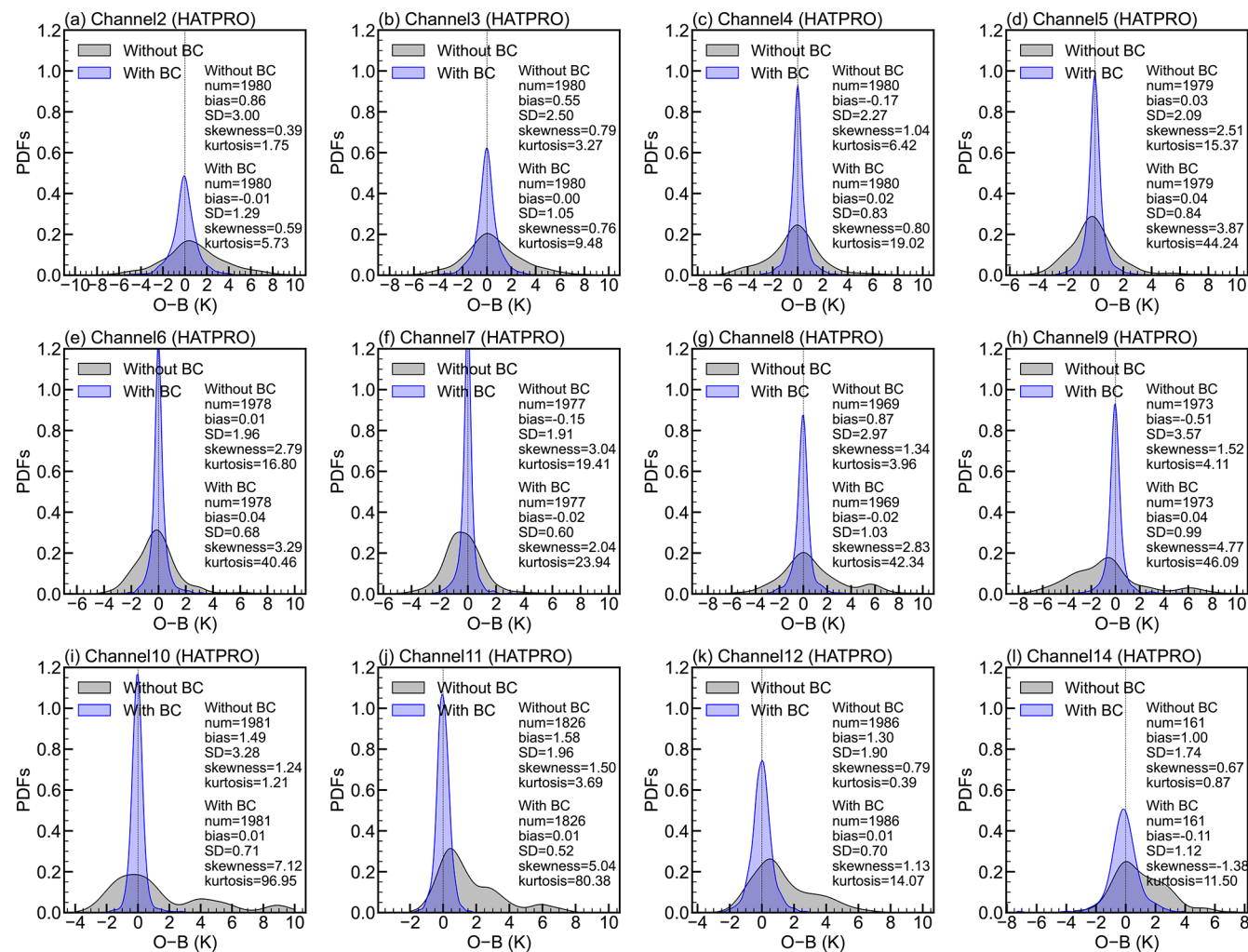
Figure B1. Probability density functions (PDFs) of the O - B distributions for HATPRO. Same as Fig. 6 but for additional channels.
