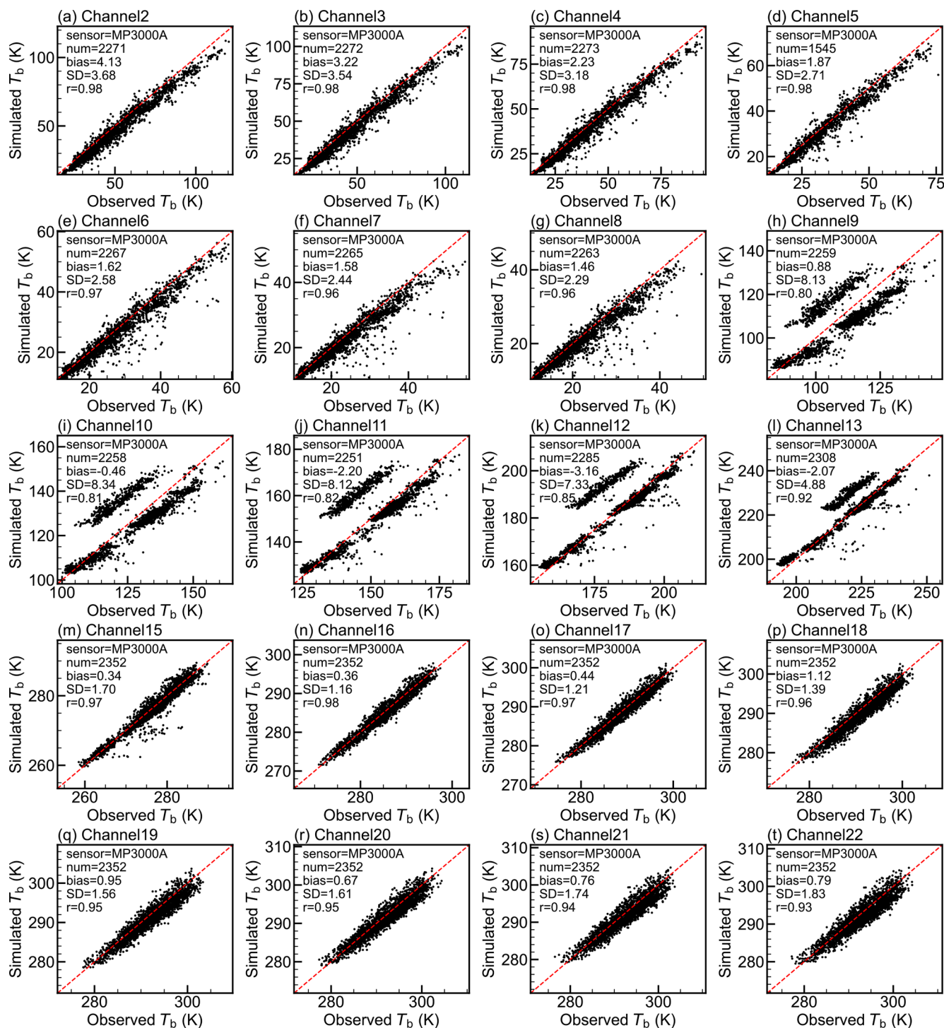
Figure A2. Scatterplots of observed brightness temperature ( T_b ) versus simulated T_b for MP3000A. Same as Fig. 3 but for additional channels.
