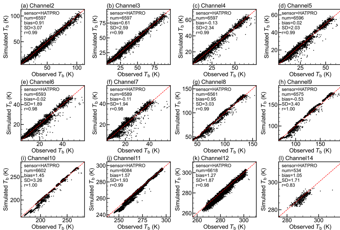
Figure A1. Scatterplots of observed brightness temperature ( T_b ) versus simulated T_b for HATPRO. Same as Fig. 3 but for additional channels.
