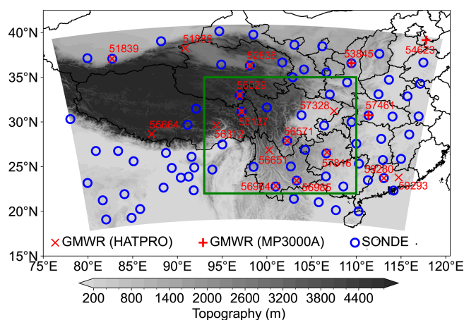
Figure 1. Computational domain (shaded). The shading denotes topography (units: m). The green rectangle denotes the target region of Southwest China. The blue open circles denote radiosondes. The “x” and “+” symbols denote HATPRO and MP3000A, respectively.
