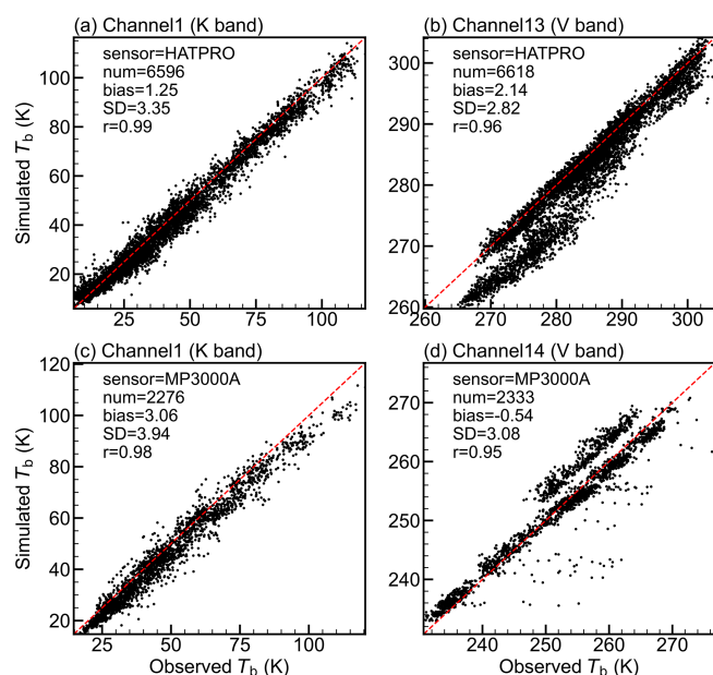
Figure 3. Scatterplots of observed brightness temperature ( T_b ) versus simulated T_b , based on samples collected from August to October 2023. The top and bottom rows correspond to the HATPRO and MP3000A sensors, and the left and right columns represent the K-band and V-band, respectively. Each panel displays the number of samples (num), the O - B mean (bias), O - B standard deviation (SD), and the correlation coefficient ( r ) between observed and simulated T_b .
