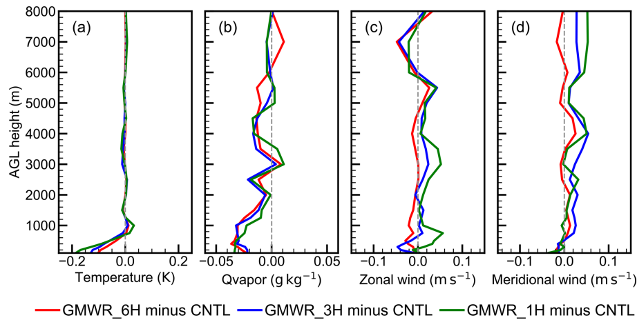
Figure 9. Verification of the initial conditions against radiosonde observations. RMSEs are computed from all samples over the 10 d assimilation experiment conducted from 13 to 22 October 2023. Root mean square error (RMSE) of (a) temperature, (b) water vapor mixing ratio (QVAPOR), (c) zonal wind, and (d) meridional wind in the target region of Southwest China (green rectangle in Fig. 1).
