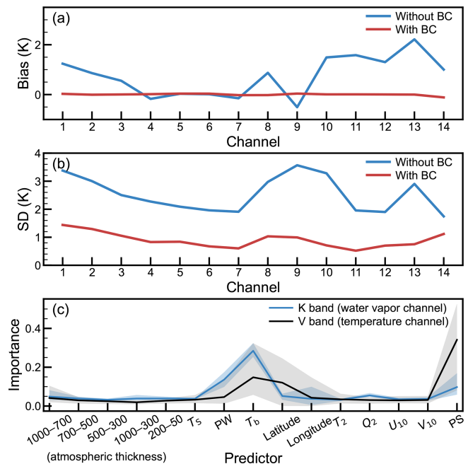
Figure 7. (a) Bias and (b) standard deviation (SD) of O - B , based on a test set randomly selected from 30 % of the three-month sample dataset collected from August to October 2023. (c) Feature importance of the predictors used in the bias correction (BC) model. For each band, the shaded regions and solid lines represent the range and mean feature importance, respectively.
