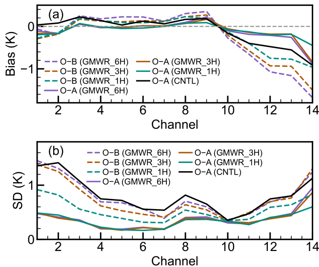
Figure 8. Verification of the initial conditions against GMWR observations, based on the 10d assimilation experiment conducted from 13 to 22 October 2023. (a) Bias and (b) standard deviation (SD) of the observation minus background ( O - B ) and observation minus analysis ( O - A ) for the GMWR assimilation in the target region of Southwest China (green rectangle in Fig. 1).
