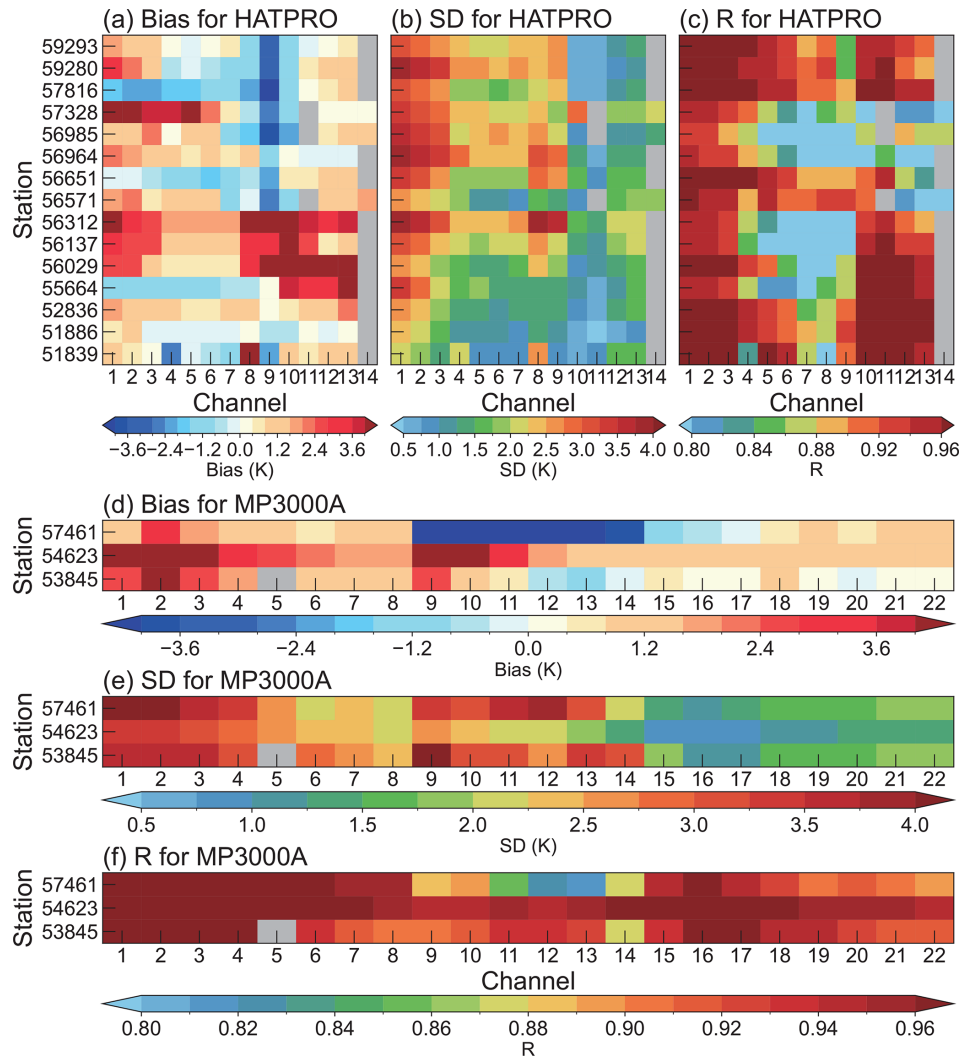
Figure 4. Statistics at each station based on samples collected from August to October 2023. O – B (a) bias and (b) standard deviation (SD) for HATPRO; (c) correlation coefficient ( r ) between observed and simulated brightness temperatures for HATPRO; (d)–(f) same as (a)–(c) but for MP3000A. Some stations did not provide observations for specific channels; the corresponding missing data are displayed in grey in the figure.
